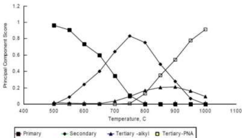
Figure 26. Relative composition of pyrolysis oils by tar class as a function of cracking temperature
