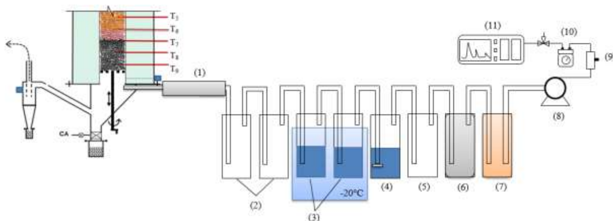
Figure 46. Sampling system for condensable and non-condensable gas
