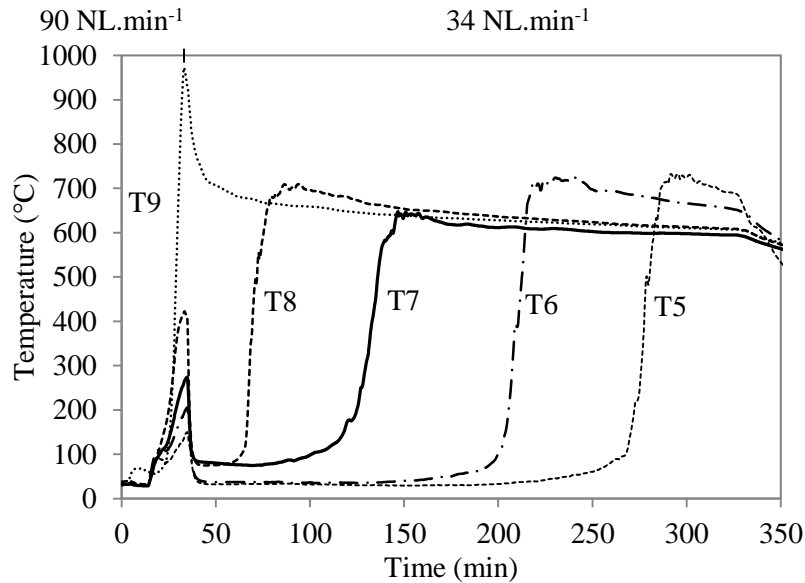
Figure 53. A typical temperature versus time profile obtained from an experiment in batch with pine pellets, 0.022 \text{ kg.m}^{-2}.\text{s}^{-1} air flux.
