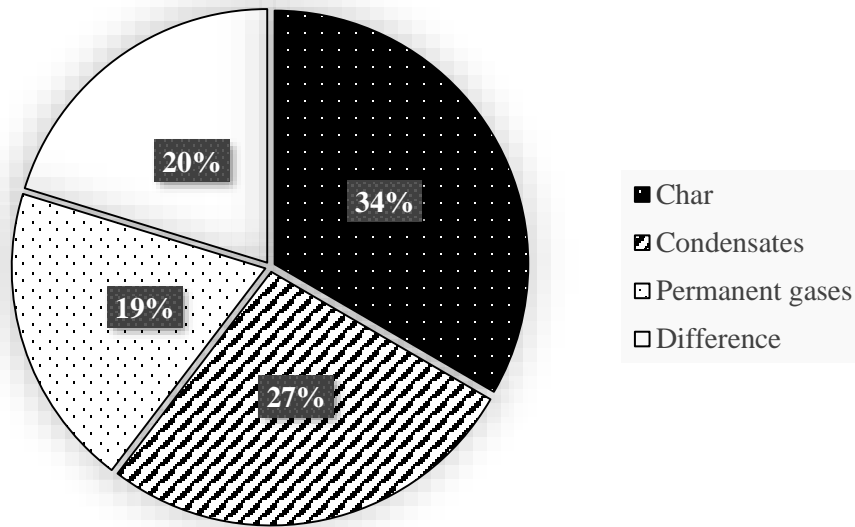
Figure 60. Energy repartition in the products from the oxidative pyrolysis of pinewood pellets, 0.022 kg.m^{-2}.s^{-1} air flux (daf)
