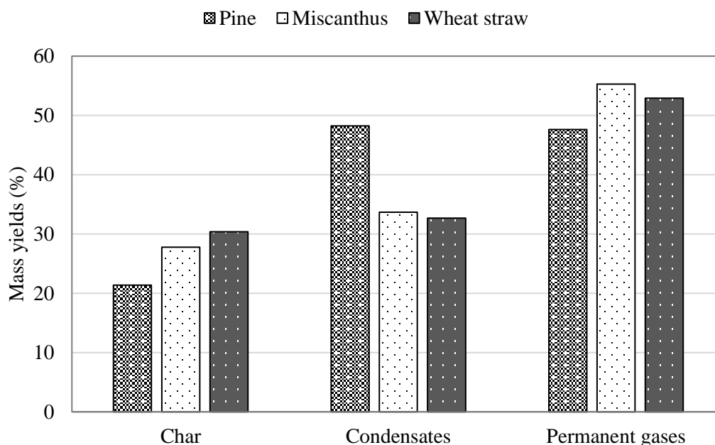
Figure 59. Mass yields (daf) of the oxidative pyrolysis products from different biomasses, 0.022 \text{ kg.m}^{-2}.\text{s}^{-1} air flux
