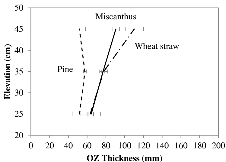
Figure 79. OZ thickness in different pellet beds with 0.022 \text{ kg}\cdot\text{m}^{-2}\cdot\text{s}^{-1} air flux
