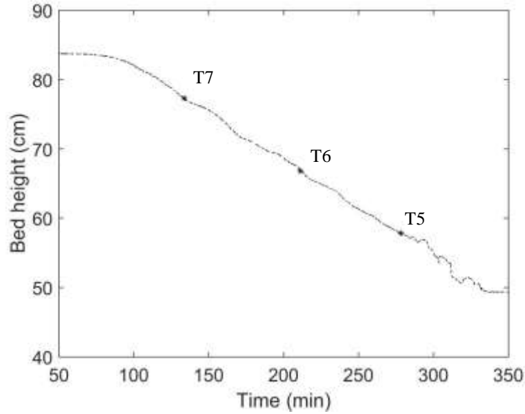
Figure 66. Bed height measurement in a batch experiment with pine pellets, 0.022 \text{ kg}\cdot\text{m}^{-2}\cdot\text{s}^{-1} air flux
