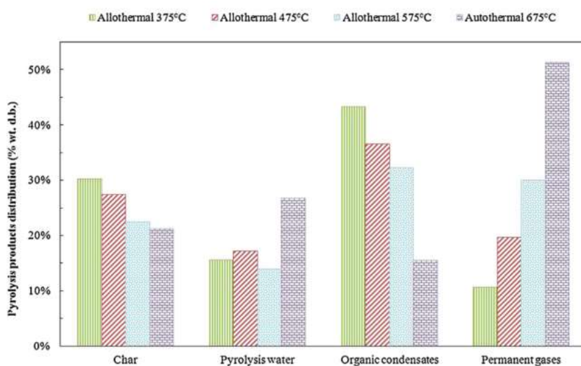
Figure 37. Distribution of pyrolysis products; yields are calculated on the basis of dry wood chips
