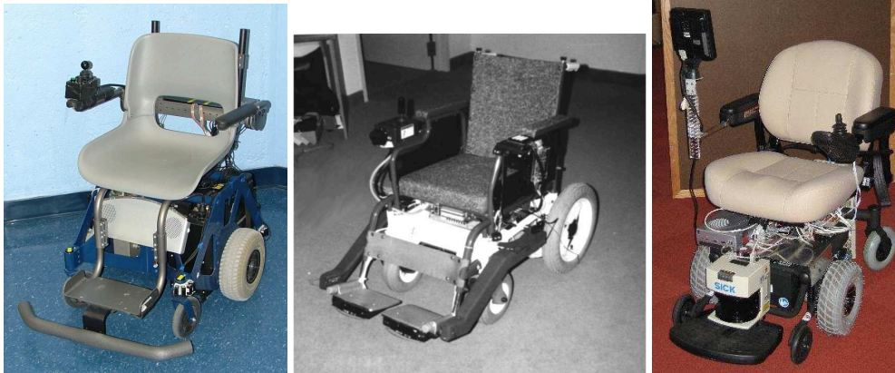
Figure 2.1: Evolution of Robotic Wheelchairs. The Wheelchair from MIT, 1996 (left), The TAO project wheelchair, 1998 (middle), and the MIT Intelligent Wheelchair Project, 2010 (right). Early intelligent wheelchair designs were robots built from the ground up or adapted by rigidly attaching a chair on a mobile robot base.
