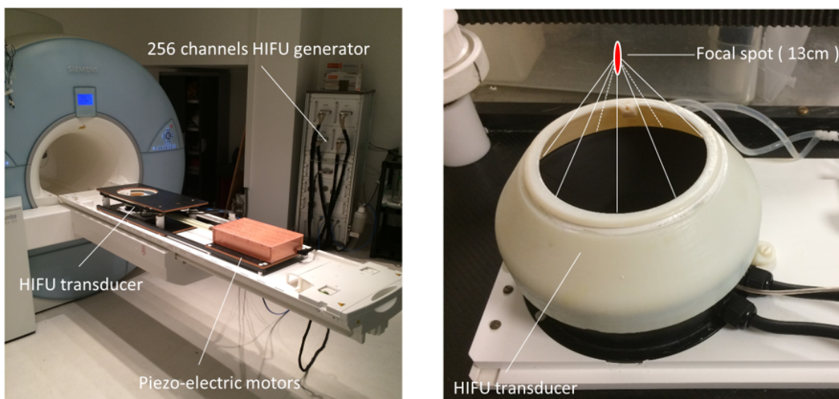
Figure 2.3: 256 elements, large animal HIFU platform.
