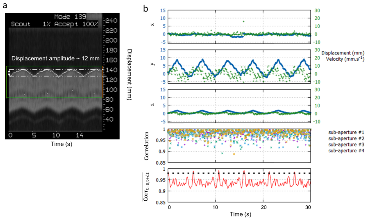
Figure 5.8: Displacement estimation in vivo on pig liver. a: Navigator signal positioned along the y-axis acquired during 20 s. b: Representative displacement estimations in (\vec{x}, \vec{y}, \vec{z}) obtained during in vivo experiment on liver. The blue and green curves represent the displacement estimations and the corresponding instantaneous speed computed from estimated positions, respectively. The bottom graph displays the cross-correlations between two successive US acquisitions along time, for each sub-apertures. The red curve displays the mean correlation between current and the first acquisition taken as reference. The black dashed line represents the threshold above which absolute displacement estimations in performed to reset the position.
