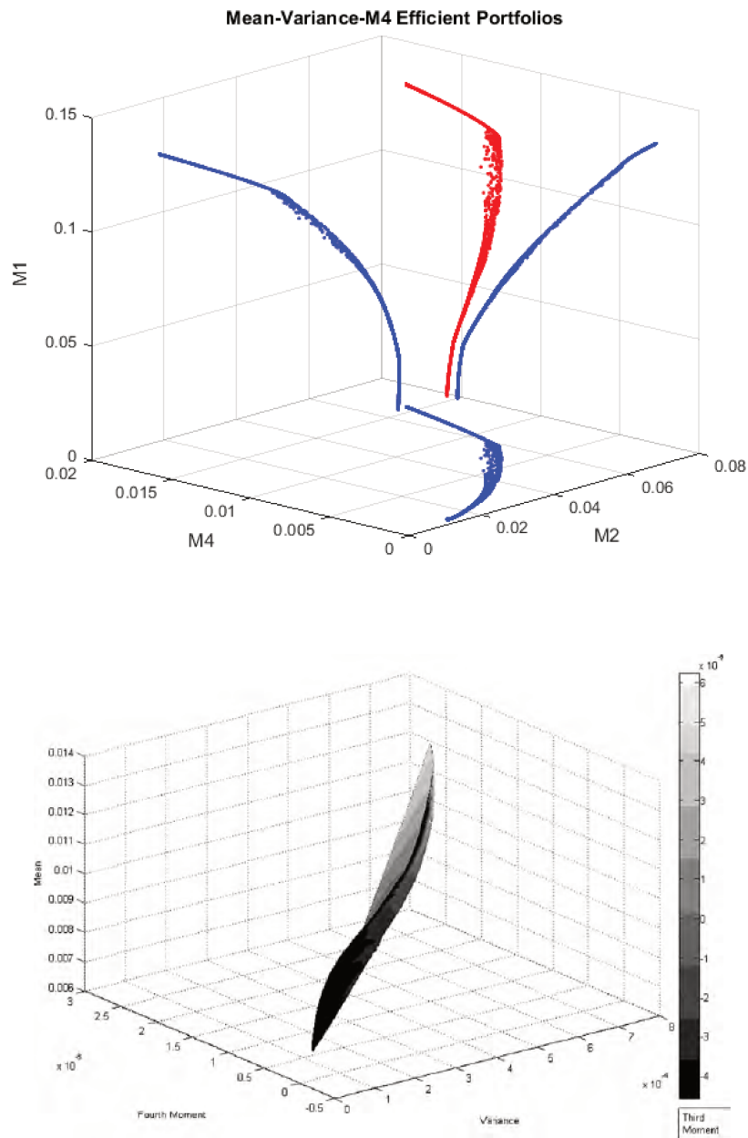
Figure 3.2 Mean–variance–skewness–kurtosis constrained efficient frontier in the mean–variance–fourth moment space. Source: HFR, monthly net asset values (1995–2005), computations by the authors. The constrained efficient frontier is obtained after optimisation of 20 hedge funds in 1296 directions. Grey shading represents the level of the third noncentral moment.
