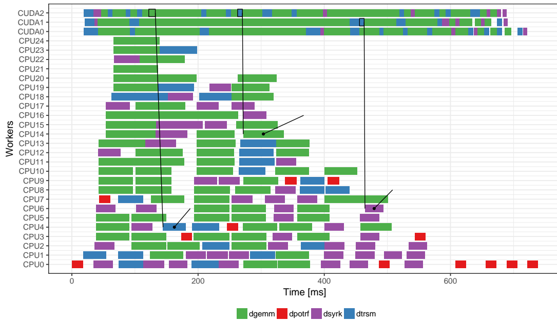
Figure 5.11: Space-time view showing only the last dependency of a some given tasks.
