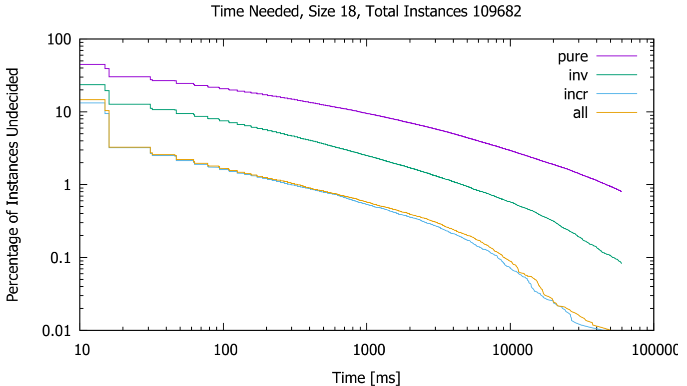
Figure 15.1 – Comparing constraint variants, undecided instances percentage for size 18 as a function of time, timeout is 60s.
