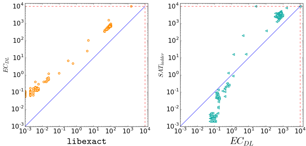
(a) x = \text{libexact} and y = EC_{DL}
