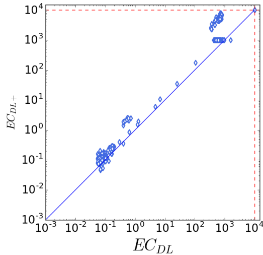
(c) (1) x = EC_{DL} and y = EC_{DL+}
