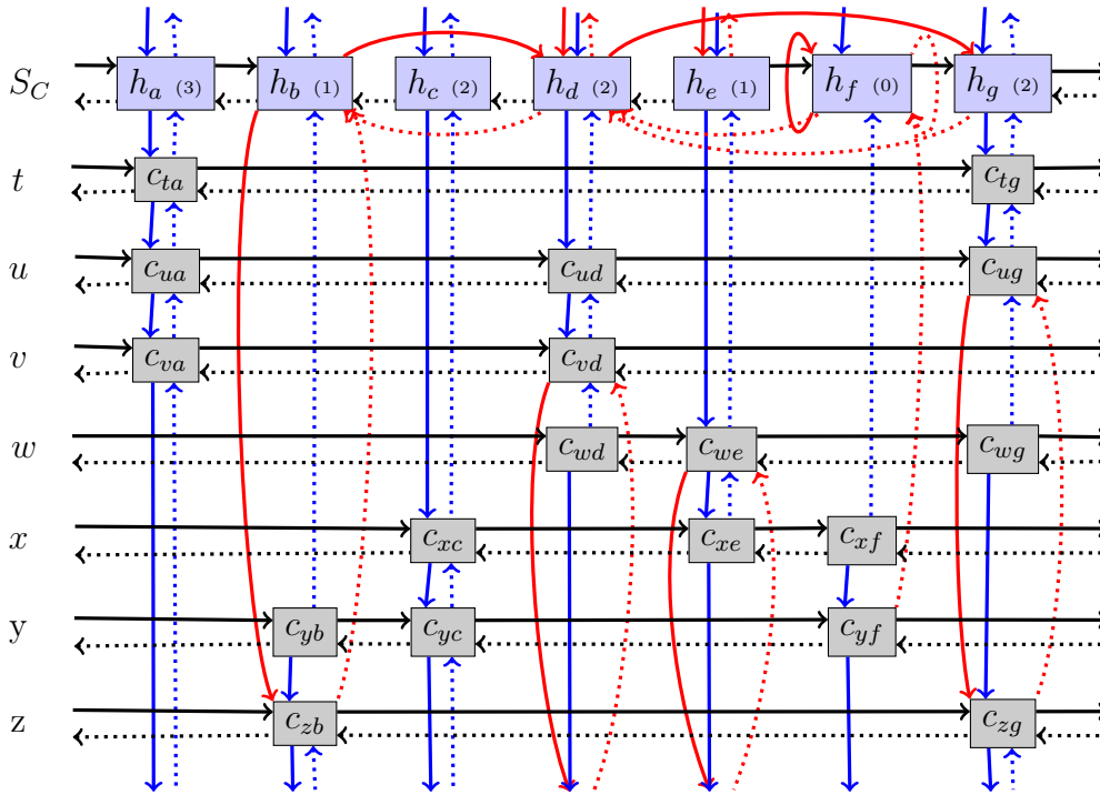
Figure 7.4 – Representation of the instance of Fig. 7.1 with Dancing Links when C = \{x\} . Links that have been modified are displayed in red.
