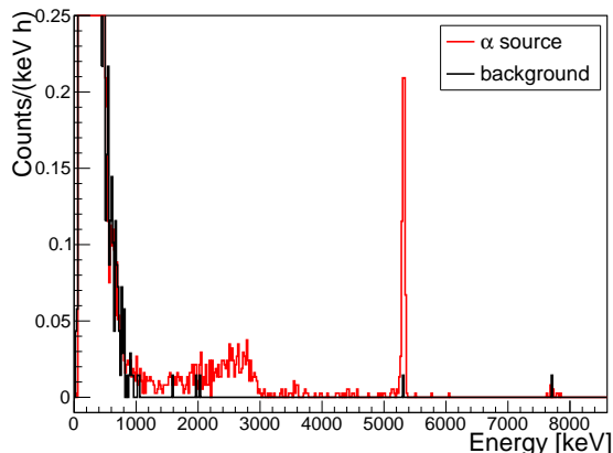
Fig. 9.3: Source ( red ) and background ( black ) spectra superimposed.
