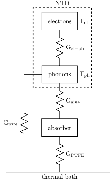
Fig. 2.4: Thermal scheme of a bolometer.
