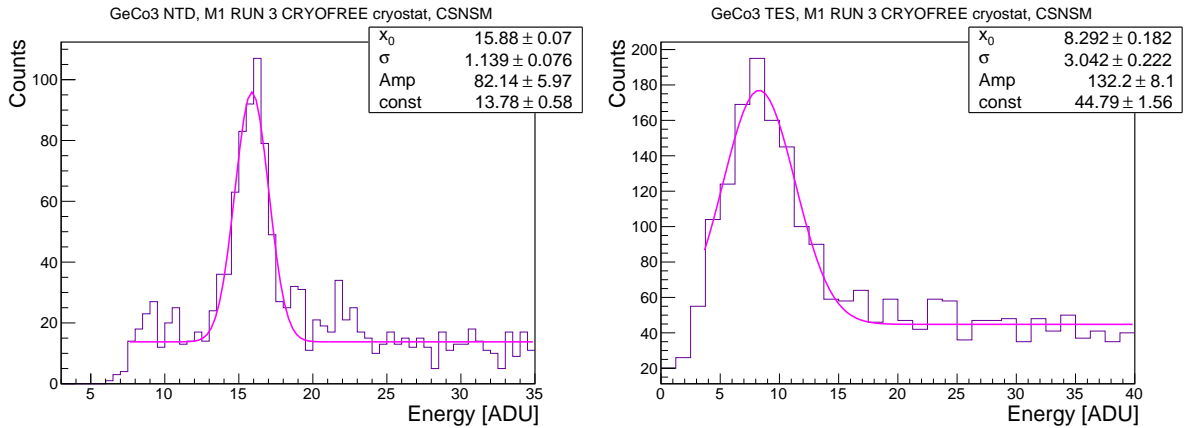
Fig. 7.4: ^{55}\text{Mn} X-ray line used for the detector calibration for the NTD ( left ) and for the TES ( right ). The line has been extracted from the TES data thanks to a trigger performed with the NTD.
