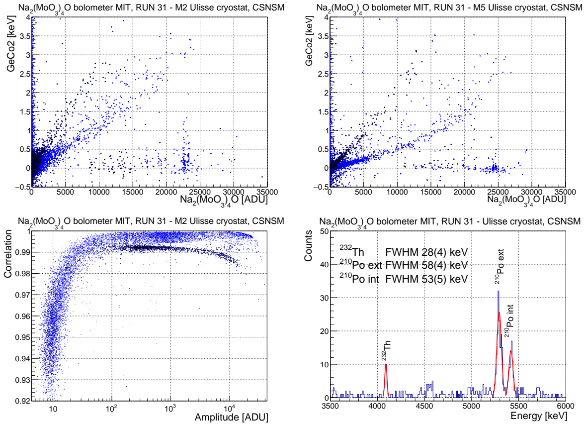
Fig. 6.22: Top panel: scatter plot of Na 2 (MoO 3 ) 4 O detector coupled to GeCo2 with grounded electrodes ( left ) and at 60 V ( right ). Bottom panel: correlation as a function of the energy ( left ) and \alpha spectrum ( right ) of Na 2 (MoO 3 ) 4 O detector.
