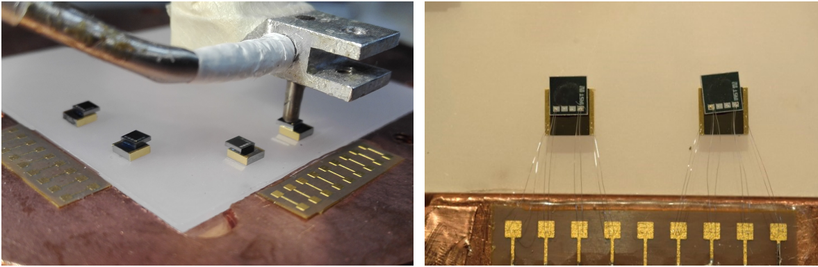
Fig. 5.5: Left panel: photograph of the last heater gluing on NTD4. Right panel: photograph of NTD3 and NTD4. The heaters are projected out of the corresponding NTDs. The chips are bonded with two aluminium wires for each pad. The external contacts have been selected for all the heaters of the mounting.
