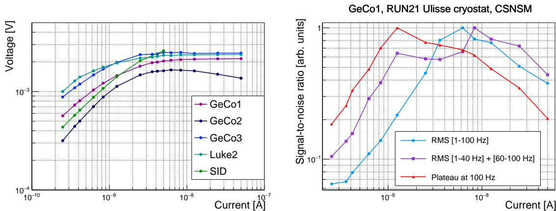
Fig. 6.2: Left panel: load curves of all the detectors measured at 18 mK. Right panel: signal-to-noise ratio renormalised for the light detector GeCo1 as a function of the bias current. Three different definitions of noise were considered: the baseline noise RMS in the frequency range 1 – 100 Hz, the baseline noise RMS in the same range excluding the 50-Hz peak and the plateau value at 100 Hz in the noise power spectra.
