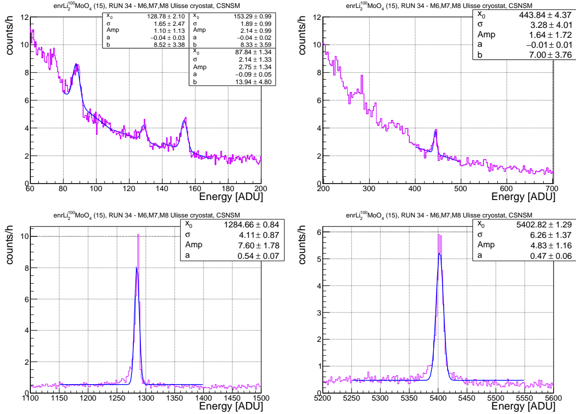
Fig. 6.29: Top panel: peaks used to calibrate the \beta region, the following peaks have been used: ^{214}\text{Pb} (351.9 keV), ^{214}\text{Bi} (609.3 keV), annihilation (511 keV), ^{214}\text{Bi} (1764.5 keV) ( left ) and ^{214}\text{Bi} (1764.5 keV) ( right ). Bottom panel: ^6\text{Li}(n,t)\alpha peak ( left ) and heater events ( right ). This measurement has been acquired at 15 mK with a bias of 1.25 nA on the NTD.
