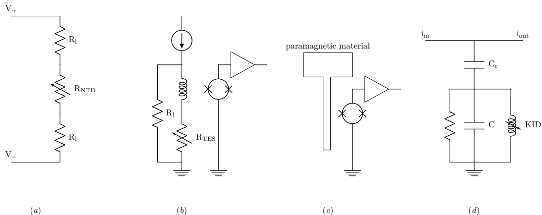
Fig. 2.2: From left: (a) A common bias circuit for NTDs is constituted by a differential circuit formed by only two load resistors ( R_1 ) crossed by a constant current. (b) TES bias circuit. The TES induces a variation in the inductance magnetic field that is read by a SQUID. (c) The magnetic field variation is read by a SQUID also in this case. (d) KID bias circuit is formed by a resonant circuit. Many circuits like this can be put in parallel on the same read-out line creating a multiplexed measurement.
