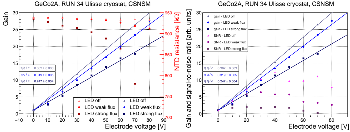
Fig. 6.32: Left panel: the gain of GeCo2A has been tested with and without a constant photon flux ( in blue ). For the same points the NTD resistance has been measured ( in red ). Right panel: the gain of GeCo2A has been tested with and without a constant photon flux ( in blue ) and for the same points the signal-to-noise ratio is reported ( in violet ).
