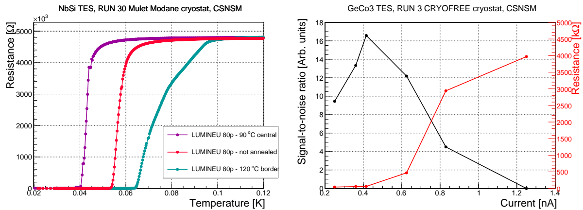
Fig. 7.2: Left panel: TES superconductive transitions of three NbSi samples. Right panel: signal-to-noise ratio and resistance as a function of the bias current for the TES glued on GeCo3.
