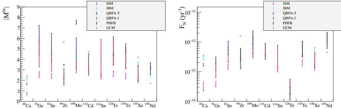
Fig. 1.5: Left panel: nuclear matrix elements for the main 0\nu 2\beta isotopes. Right panel: F_N term — from Eq. (1.17) — for the main 0\nu 2\beta isotopes. The error bands are due to the uncertainties on the nuclear matrix element and axial coupling constant g_A .
