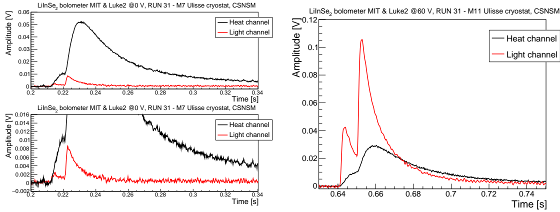
Fig. 6.17: Left panel: pile-up event in the heat channel compared to the light channel read with the grounded electrodes ( top ) with a zoom on the light event ( bottom ). Right panel: an equivalent-energy pile-up event in the heat channel compared to the light channel read with 60-V electrodes bias.
