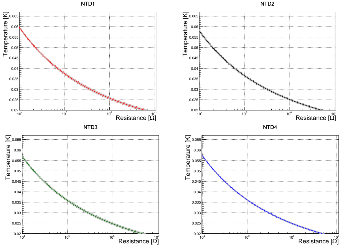
Fig. 5.24: The temperature as a function of the resistance calculated from the average R_0 and T_0 obtained with the analysis of systematic errors. Their systematic uncertainty is represented by a gray band.
