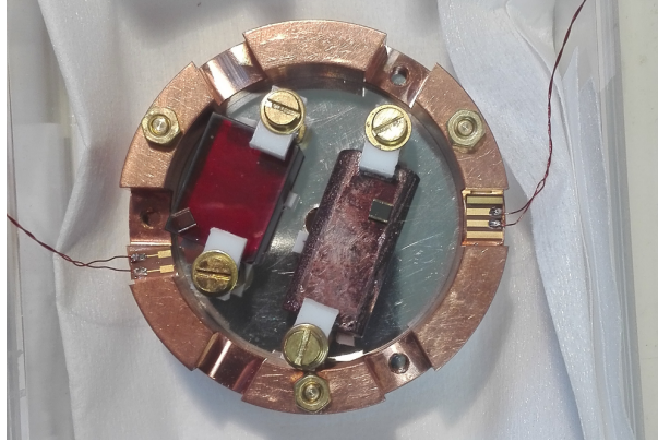
Fig. 6.16: Photograph of the mounting of LiInSe 2 ( left ) and GaSe ( right ) bolometers.
