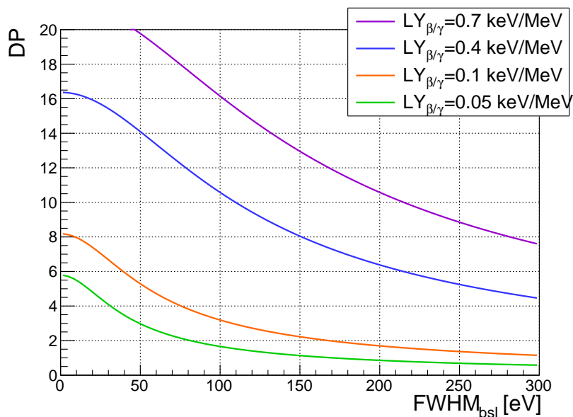
Fig. 2.7: Discrimination power at 2.6 MeV as a function of the light-detector FWHM baseline for different light yield.
