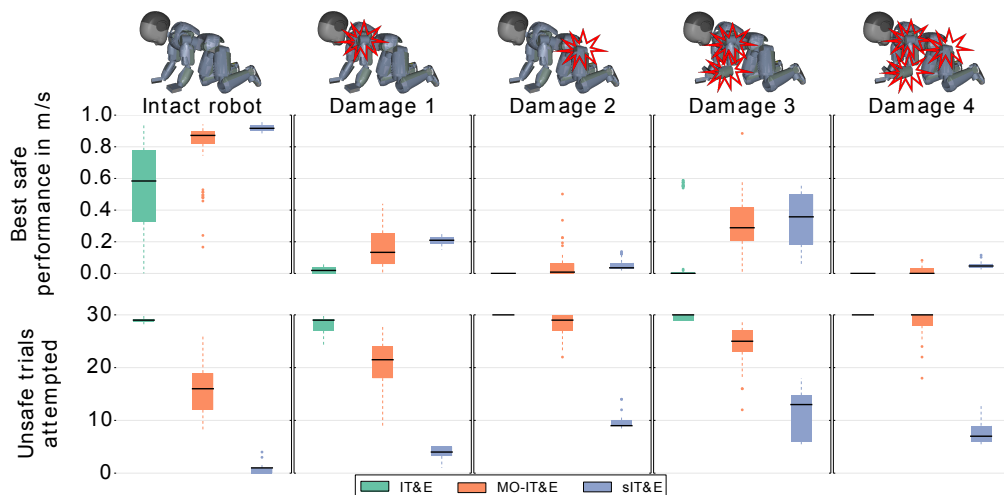
Figure 6.2: Comparison between IT&E, MO-IT&E and sIT&E. Each algorithm is ran 20 times for 4 different behavior-performance maps. We report the best safe performance ( i.e. , the fastest crawling speed within the safe region observed during the learning process) (upper row) and number of unsafe trials attempted (violating the constraints) (lower row). Horizontal black lines represent medians.
