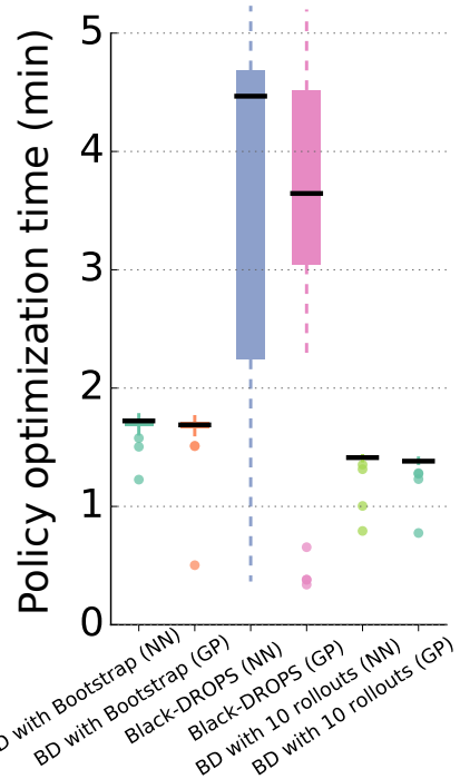
Figure 4.13: Policy optimization time for the very noisy pendulum task (20 replicates). Black-DROPS with bootstrap and races requires similar time to the expert number of rollouts and much less time than the vanilla Black-DROPS algorithm. See Fig. 4.2 for legend.
