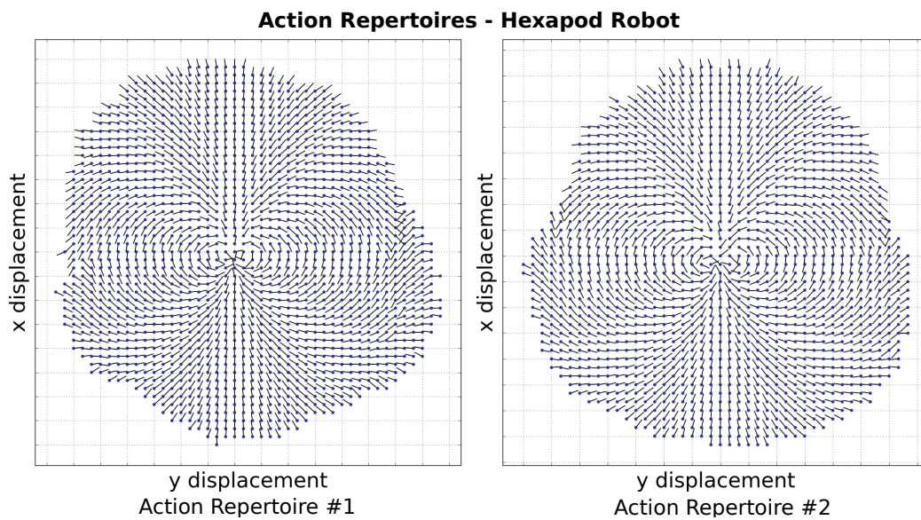
Figure 3.9: Repertoires for hexapod locomotion produced by the MAP-Elites algorithm. These repertoires map the 2-D action descriptor (of the 3-D task space) to the 36-D controller space. Each dot represents a different action (and its x, y position), while the lines indicate the orientation of the robot at the end of each behavior. All the behaviors are relative to the zero position that is located in the middle of the figures and relative to the forward orientation (line pointing up).
