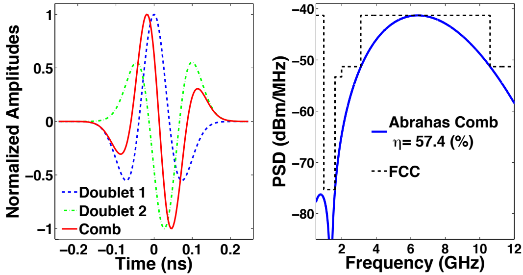
Figure 3.10: Abrahas proposed pulse based on a combination of Gaussian Doublets.
