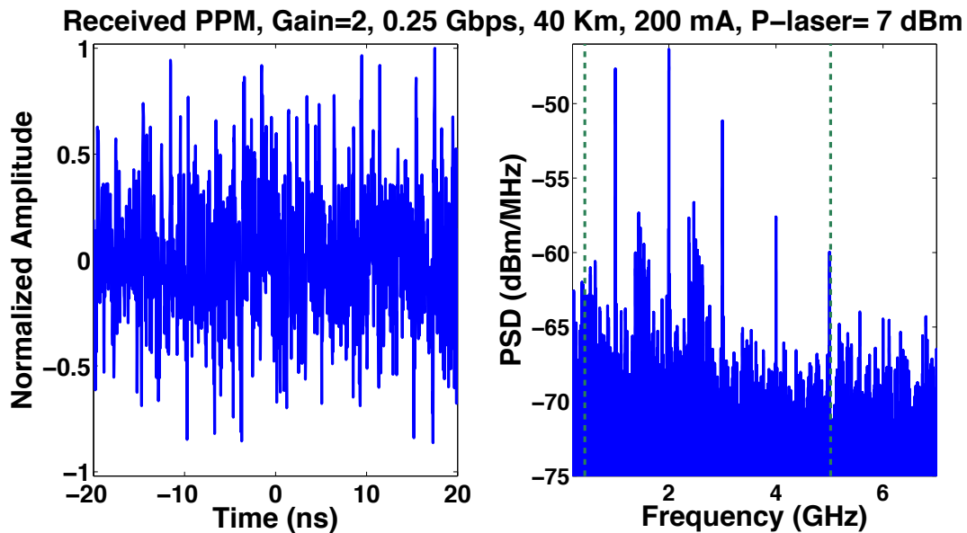
Figure 6.13: Time waveforms and corresponding power spectral density of PPM operating at 0.25 Gbps, where the laser output power is 7 dBm, I_{bias}= 200 mA, and SOA is placed at 40 km (the time waveform is a truncation of only 10 symbols).
