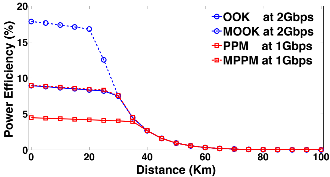
Figure 5.15: Power Efficiency versus Fiber Length, where MZM is injected by 15 dBm Laser Power.
