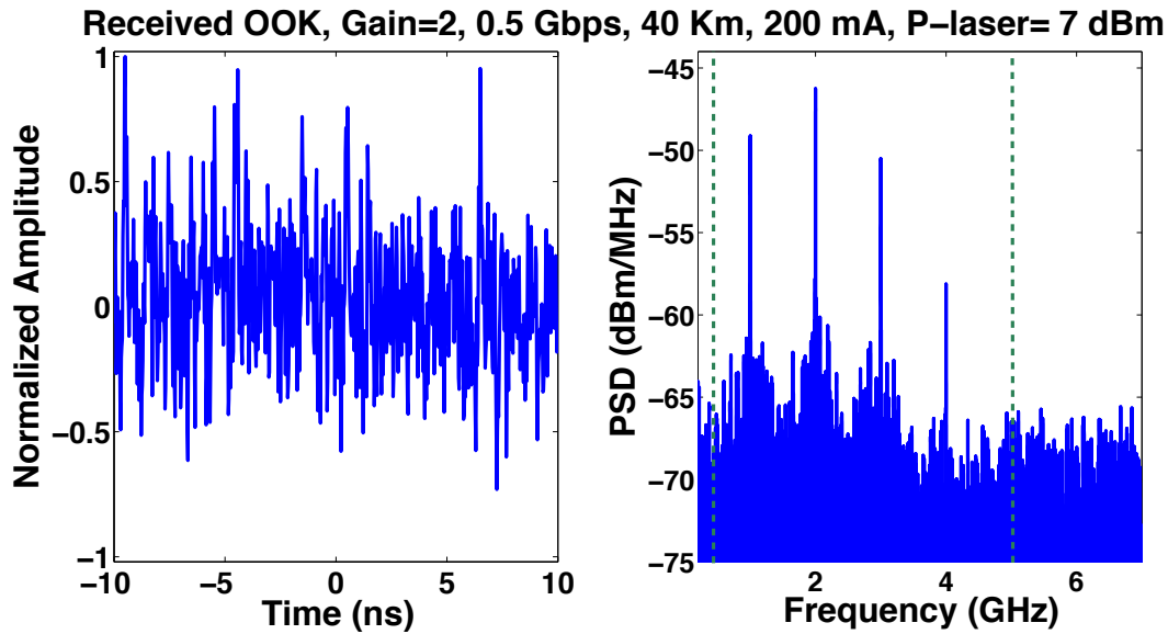
Figure 6.12: Time waveforms and corresponding power spectral density of OOK operating at 0.5 Gbps, where the laser output power is 7 dBm, I_{bias}= 200 mA, and SOA is placed at 40 km (the time waveform is a truncation of only 10 symbols).
