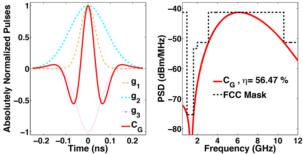
Figure 3.12: Our proposed combination C_G based on the pulses g_i , in time (left) and frequency (right) domain.
