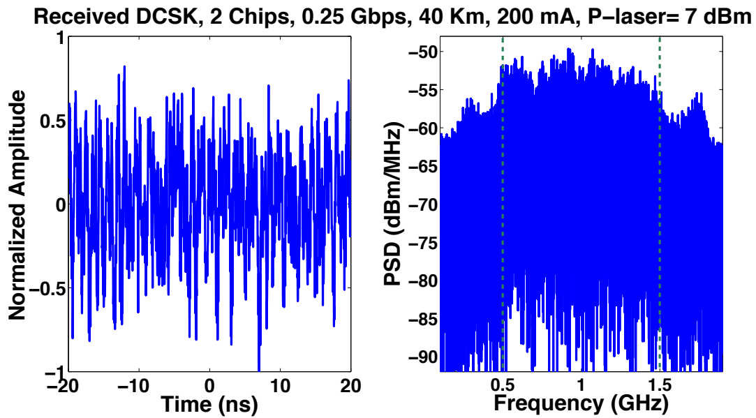
Figure 6.10: Time waveforms and corresponding power spectral density of 2-DCSK operating at 0.25 Gbps, where the laser output power is 7 dBm, I_{bias}= 200 mA, and SOA is placed at 40 km (the time waveform is a truncation of only 10 symbols).
