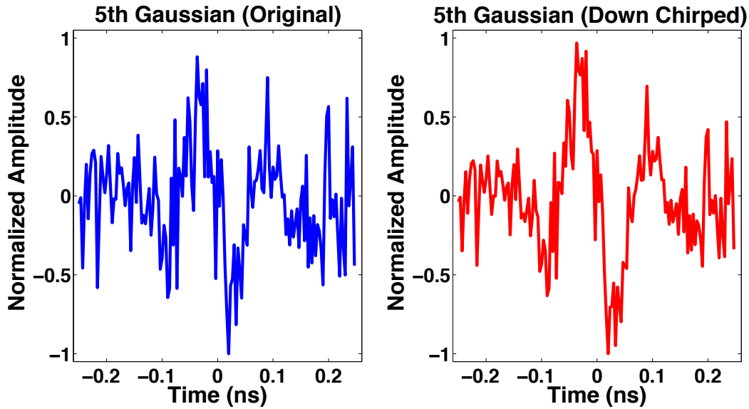
Figure 4.8: Time waveforms of the noisy 5th Gaussian obtained at SOA output, with (right) and without (left) chirping, P_{\text{SOA}} = -20 dBm, V_{pp} = 0.1V\pi , I_{bias} = 250 mA.
