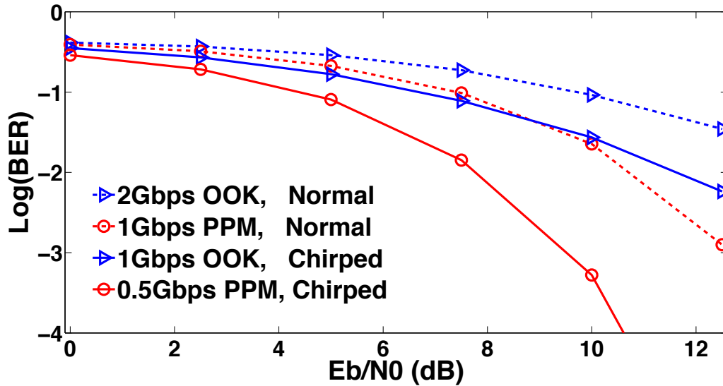
Figure 4.5: Bit error rate versus E_b/N_0 for normal and chirped (with a slope of 0.0472 ns/GHz) transmissions over AWGN channel, considering OOK and PPM modulations.
