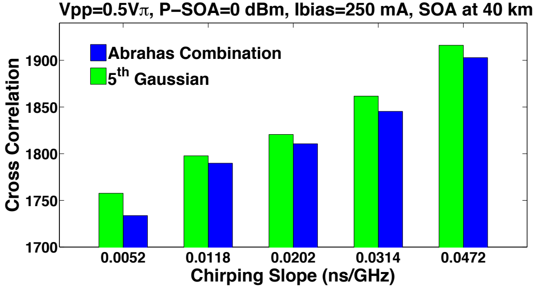
Figure 4.11: Cross Correlation between electrical and optical waveforms versus chirping slope, for the 5th Gaussian pulse and Abraha's combination, where V_{pp} = 0.5V\pi , I_{bias} = 250 mA, P-SOA=0 dBm.
