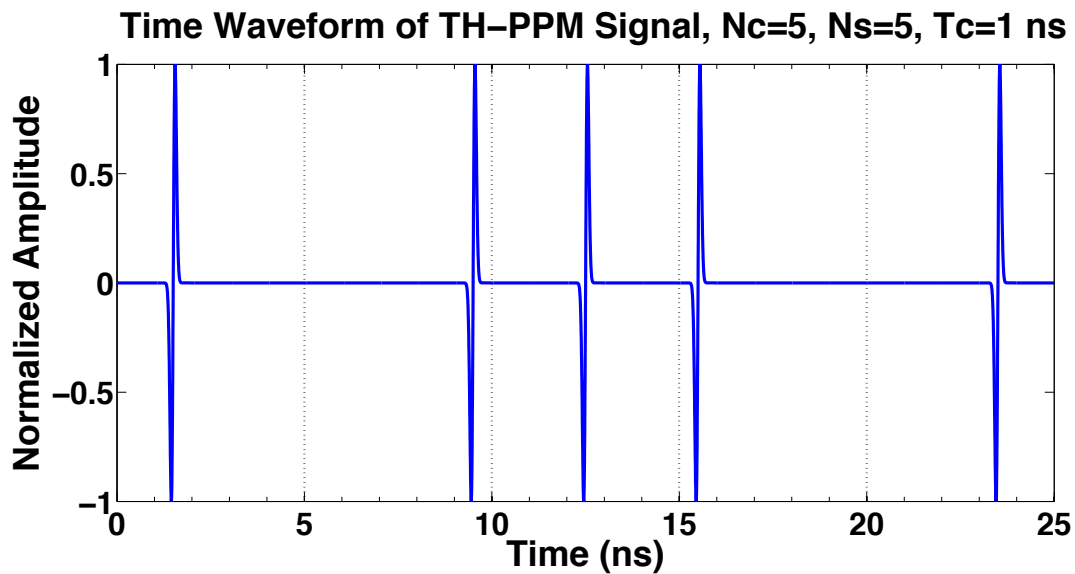
Figure 5.2: Time Representation for 1 symbol extracted from a TH-PPM signal, consisting of 5 frames/symbol, and 5 chips/frame, the TH code is [2 5 3 1 4] and T_c=1 ns, where the basic transmitted pulse is the Gaussian Monocycle.
