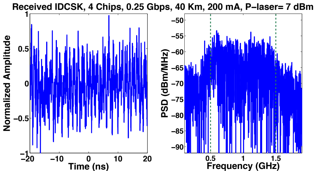
Figure 6.11: Time waveforms and corresponding power spectral density of 4-I-DCSK operating at 0.25 Gbps, where the laser output power is 7 dBm, I_{bias}= 200 mA, and SOA is placed at 40 km (the time waveform is a truncation of only 10 symbols).
