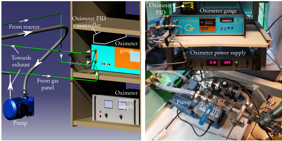
(a) – CAD view of the gas circuit instrumentation, i.e. the oximeter and the pump. (b) – Photograph of the gas circuit instrumentation. a): oximeter, b): pump.
