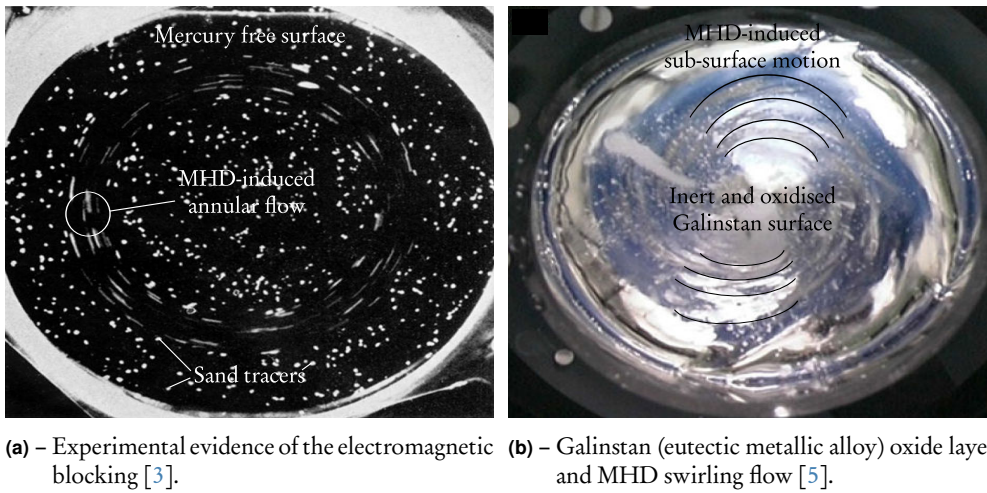
Figure I.A.2 – Fundamental stratified MHD flows.
