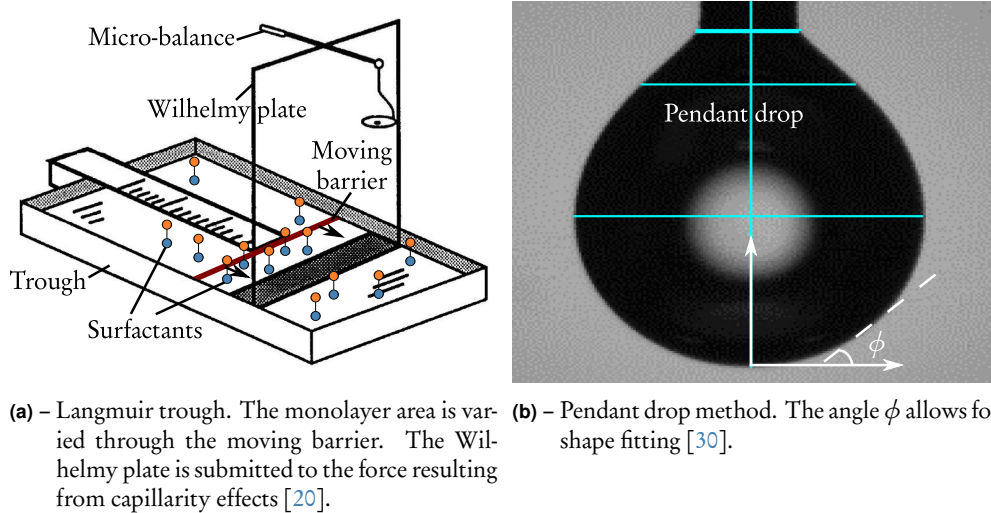
Figure I.B.4 – Experimental techniques for determining surface tension \gamma .
