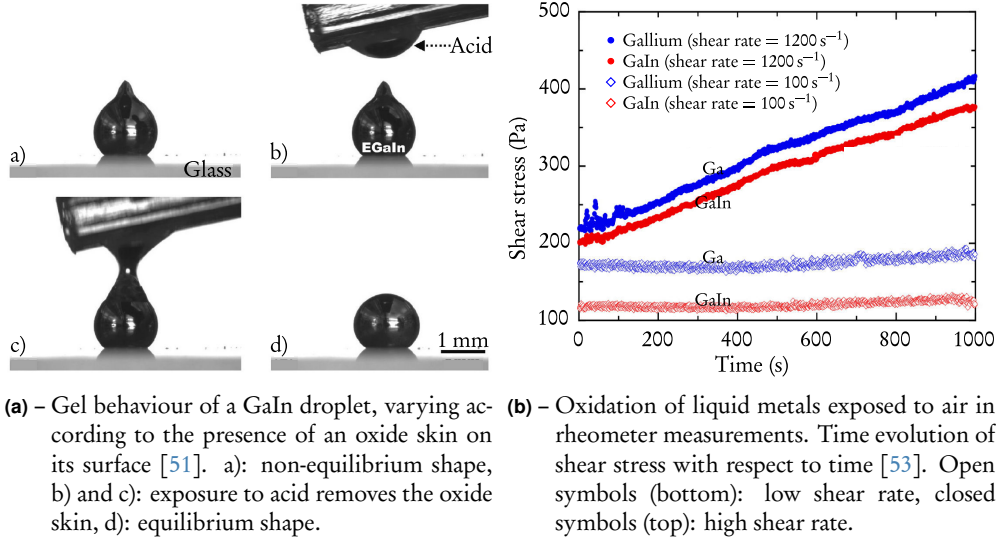
Figure I.B.9 – Gel behaviour and varying apparent bulk viscosity of gradually oxidising Galinstan.
