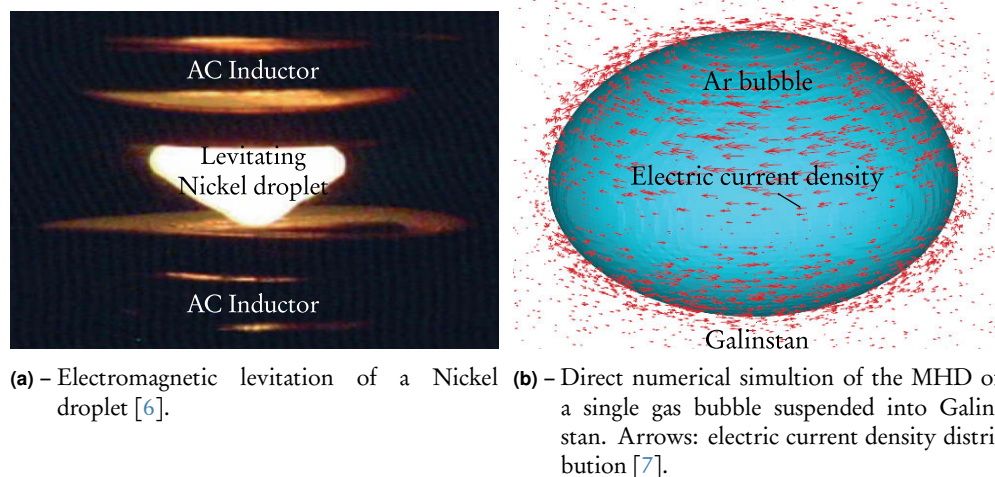
Figure I.A.4 – Fundamental dispersed MHD flows.
