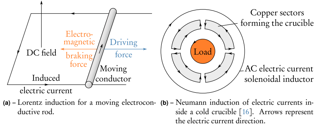
Figure I.B.1 – The induction principle.
