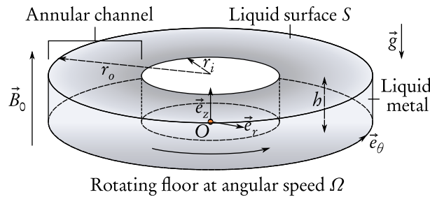
Figure III.A.4 – The annular MHD viscometer.
