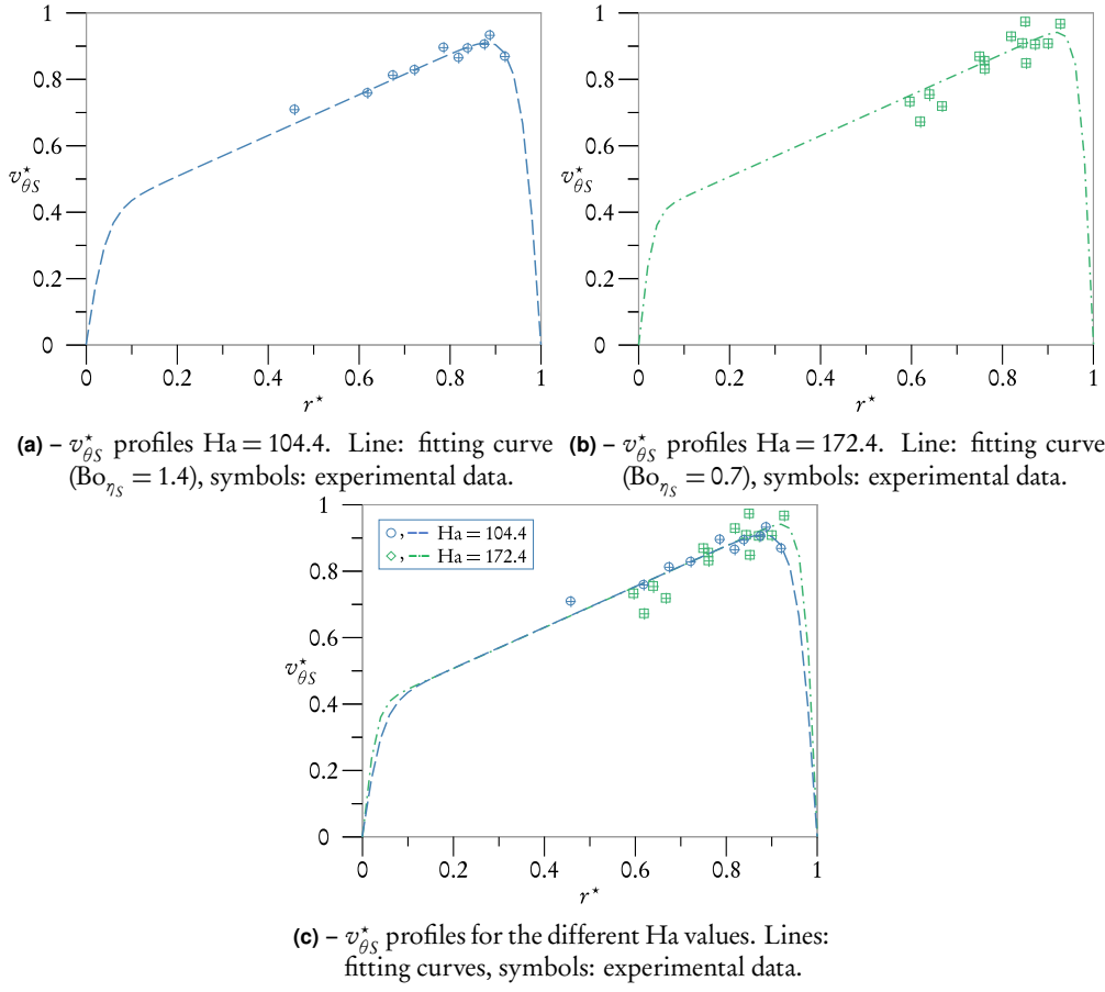
Figure III.D.21 – Experimental v_{\theta S}^* profiles and associated curve fittings, for \text{Re} = 4494 and various \text{Ha} .
