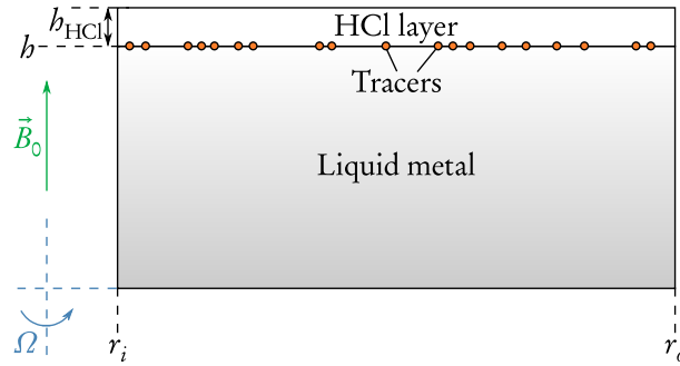
Figure III.D.16 – Experimental layout with the HCl layer.
