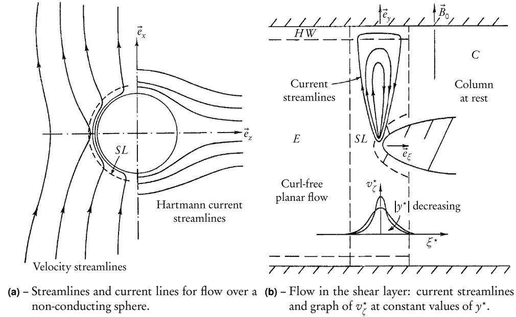
Figure D.12 – Typical flow patterns past a spherical obstacle when \text{Ha}, N \gg 1 [55].
