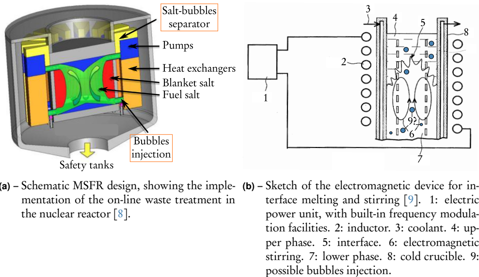
Figure I.A.5 – Industrial dispersed MHD flows: application to GEN-IV MSFR fission reactor.
