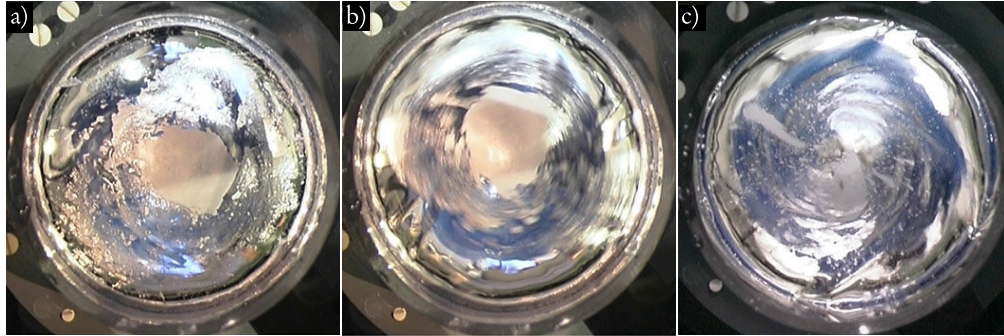
(a) – Intermittent behaviour caused by surface oxidation in a Galinstan (eutectic Ga-In-Sn) flow driven by a rotating magnetic field [5]. a): oxide layer at rest, b) oxide layer in motion, c) closed oxide layer at rest in presence of an intense swirling motion of the fluid beneath.
