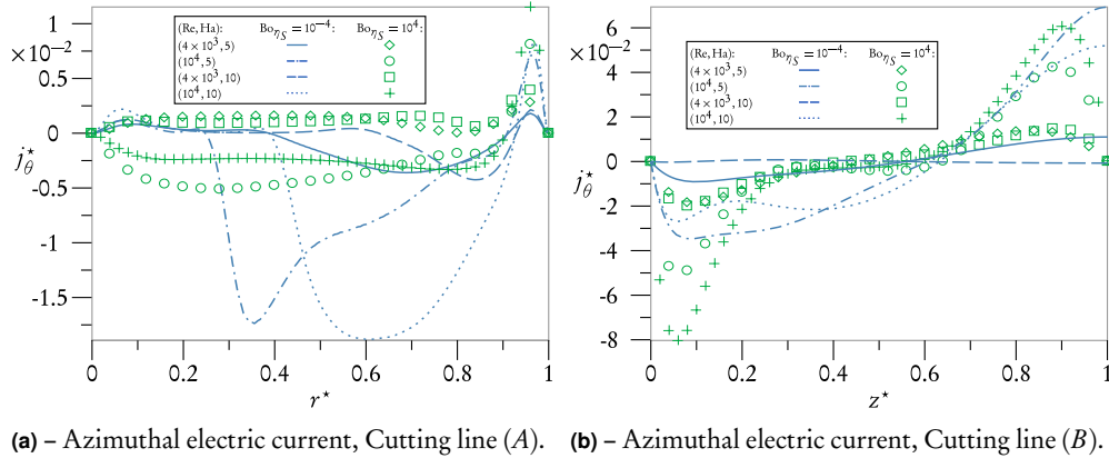
Figure III.C.7 – Azimuthal electric current density j_\theta^* , along cutting lines (A) for a) and B for b), for various Re, Ha and Bo_{\eta_S} values. j_\theta^* is normalized by J_{\max} = 3.96 \times 10^3 \text{ A}\cdot\text{m}^{-2} , i.e. the maximum electric current reached in all cases, for the highest (Re, Ha) = (10^4, 10) values.
