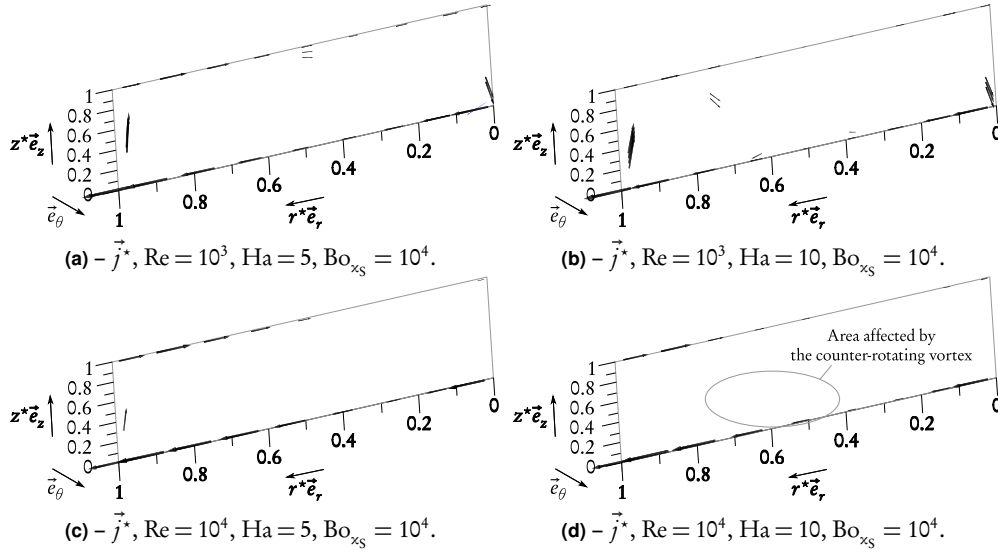
Figure III.C.13 – \vec{j}^* for Ha = 5 (left part), or Ha = 10 (right part). \vec{j}^* is log-scaled by the magnitude \exp((\ln(\|\vec{j}^*\|/\|\vec{j}^*\|_{\max}))/ (1 + p)) ; p = 2 for a , b , and 1.5 for c , d . Black (greyscale: darkest) arrows are essentially meridian, while beige (greyscale: lightest) and blue (greyscale: intermediate) arrows correspond to significantly (\|\vec{j}_\theta^*\|/\|\vec{j}^*\| \geq 0.01) positive and negative azimuthal components, respectively.
