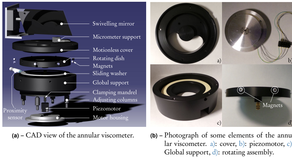
Figure III.D.3 – Working area ①: the annular channel viscometer.
