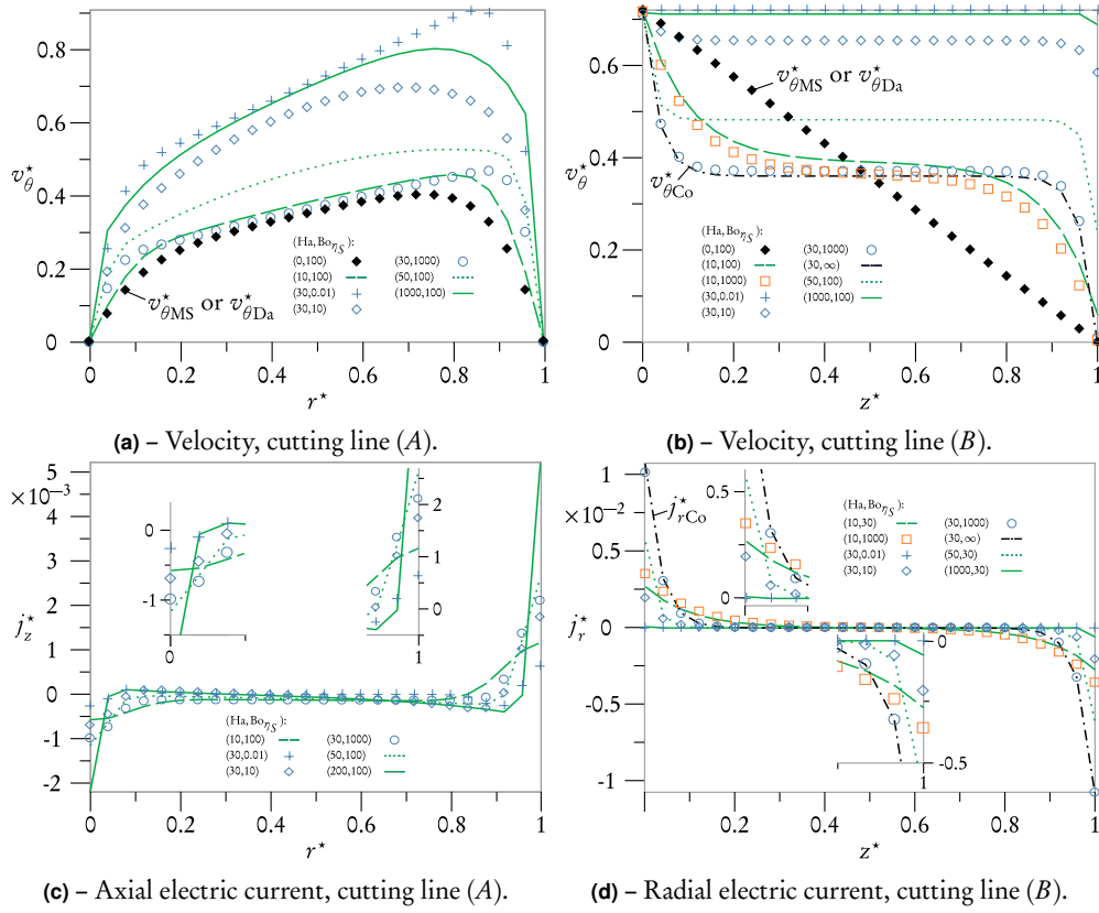
Figure III.B.6 – Velocity and electric current with respect to various (\text{Ha}, \text{Bo}_{\eta_s}) values, along cutting lines (A) (left-hand column) or (B) (right-hand column). MS, Da and Co refer to Mannheimer and Schechter (Eq. (III.A.2)), Davoust (Eq. (III.A.4)) or Couette asymptotic solutions (Eq. (III.B.13)), respectively. The electric current densities are normalised with respect to the maximum electric current J_{\max} = 1.36 \times 10^4 \text{ A} \cdot \text{m}^{-2} (reached for \text{Ha} = 10^3 ).
