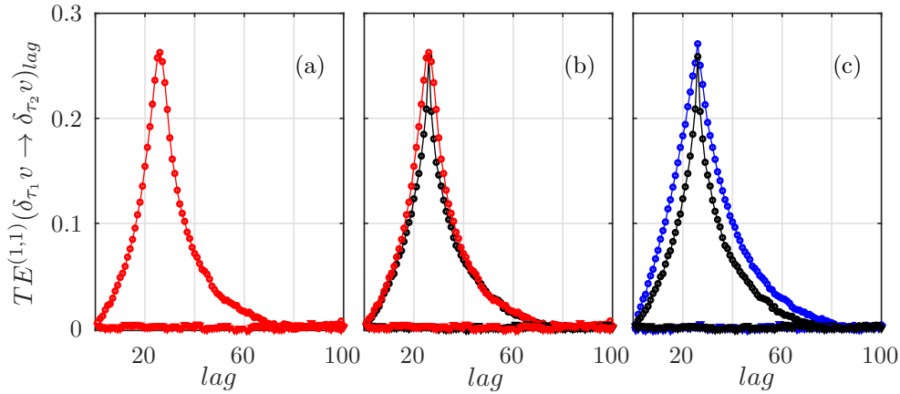
Figure 8.2: Transfer entropy between scales \delta_{\tau_l} and \delta_{\tau_s} , with \tau_l = 92 and \tau_s = 66 m for turbulence (red), fBm with \mathcal{H} = 0.3 (black), and fBm with \mathcal{H} = 0.5 (blue). Circles indicate the TE from the small to the large scale, and triangles indicate the TE from the large to the small scale. a) Turbulence b) Comparison between turbulence and fBm with \mathcal{H} = 0.3 c) Comparison between fBm with \mathcal{H} = 0.3 and fBm with \mathcal{H} = 0.5
