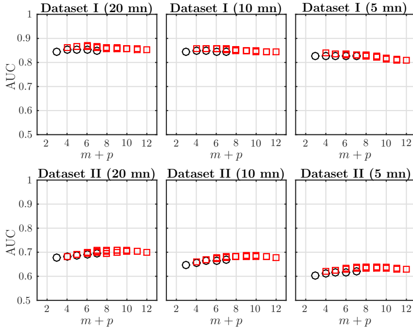
Figure 9.3: AUC of ROC for \hat{I}^{(m,p)} as a function of the total embedding dimension m+p , with m \geq p , for time windows of size T = 20, 10, 5 mn, for data in Dataset I (first line) and Dataset II (second line). Black circles indicate the special case p = 1 corresponding to the classical definition of Shannon entropy rate (see eq.(1.25)). Red squares correspond to p \geq 2 .
