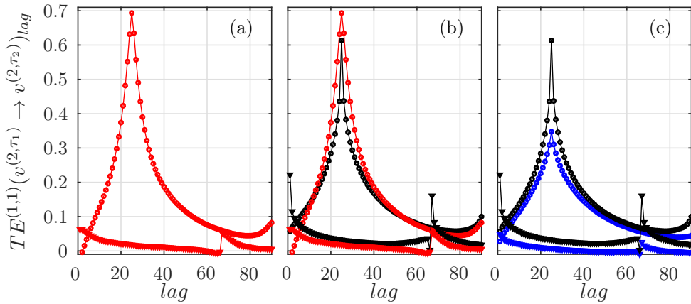
Figure 8.7: Transfer entropy between scales v^{(2,\tau_1)} and v^{(2,\tau_s)} , with \tau_l = 92 and \tau_s = 66\text{m} for turbulence (red), fBm with \mathcal{H} = 0.3 (black), and fBm with \mathcal{H} = 0.5 (blue). Circles indicate the TE from the small to the large scale, and triangles indicate the TE from the large to the small scale. a) Turbulence b) Comparison between turbulence and fBm with \mathcal{H} = 0.3 c) Comparison between fBm with \mathcal{H} = 0.3 and fBm with \mathcal{H} = 0.5
