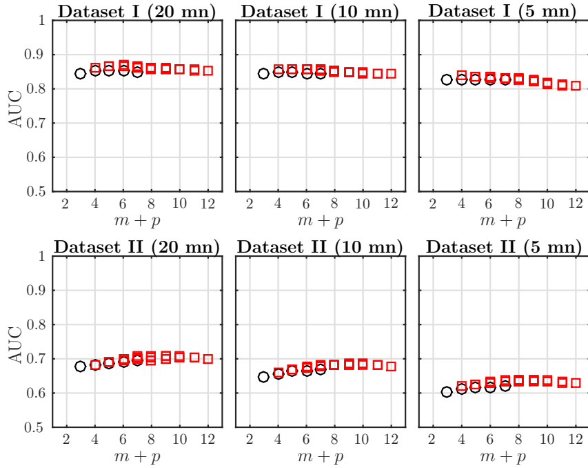
Figure 9.3: AUC of ROC for \hat{I}^{(m,p)} as a function of the total embedding dimension m+p , with m \geq p , for time windows of size T = 20, 10, 5 mn, for data in Dataset I (first line) and Dataset II (second line). Black circles indicate the special case p = 1 corresponding to the classical definition of Shannon entropy rate (see eq.(1.25)). Red squares correspond to p \geq 2 .
