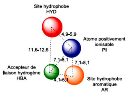
Figure 7-Pharmacophore de Lopez-Rodriguez 153
