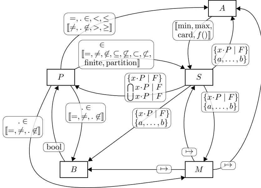
Figure 4: The different syntactic categories and the symbols relating them: A for arithmetic expressions, P for predicates, S for set expressions, B for Boolean expressions and M for maplet expressions. ppTrans removes all occurrences of the constructs delimited by double-brackets.
