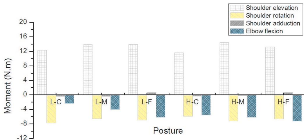
Figure VI.4 – The shoulder rotation moment is considerable beside of the elevation moment
