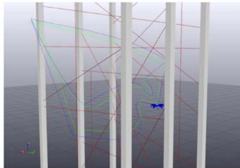
Figure 5.3 – Agile path tracking with a micro quadrotor in a heavily cluttered environment of strings and poles. The algorithm takes about 10 minutes to return a solution, from [29].
