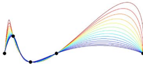
Figure 5.6 – Shape of a trajectory passing through waypoints with different flying times, from [73].
