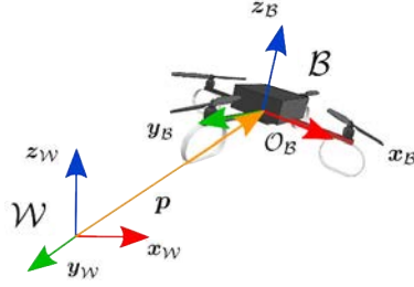
Figure 2.1 – Quadrotor model
