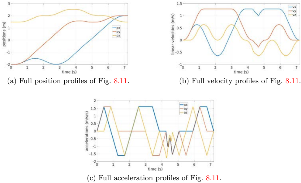
Figure 8.12 – Connection of the position, velocity and acceleration profiles
