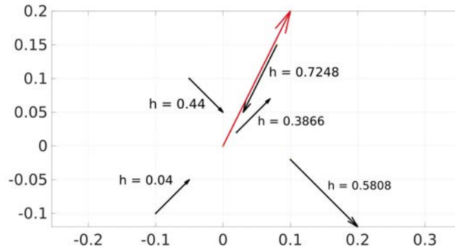
Figure 8.6 – Computation of the heuristic cost h(\mathbf{s}_1, \mathbf{s}_2) between multiple vertices \mathbf{s}_1 and a goal vertex \mathbf{s}_2 at the origin. The arrows represent the vertices linear velocity. As we can see the vertex with the lowest cost is the one whose velocity vector is the most “aligned” with the goal velocity vector. Vertices that are closer to the goal have a higher cost.
