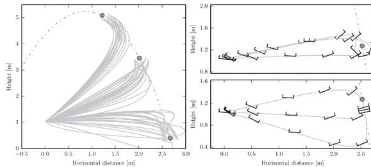
Figure 5.1 – Sampled motion primitives for a catching manoeuvre. The presented algorithm is able to generate about 6700 feasible motion primitives per second, from [33].
