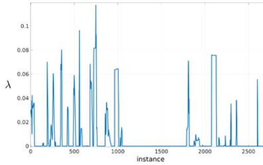
Figure 7.4 – Evolution of \lambda for the simulation. The peaks reveal the presence of sudden occlusions. The flat section (from around instance 1100 to instance 1700) represents a flight period when the target is far from the obstacles. Therefore, \lambda is very close to 0. Here \lambda did not hit the upper limit R_{occ} = 0.15m .
