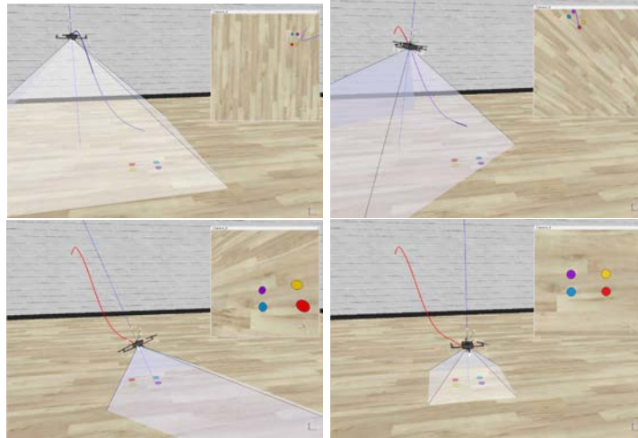
Figure 6.5 – Successive snapshots taken from V-Rep at different time instants. The straight line represents the vertical axis of the camera, the blue line is the planned trajectory and the red line is the actual system trajectory. The camera view is shown in the upper right corner.
