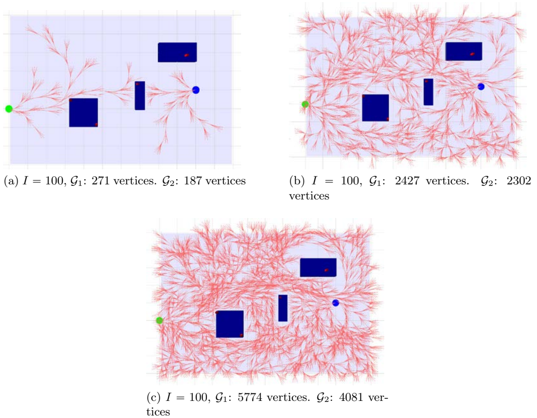
Figure 8.4 – Planner performance in exploring a 2D environment. When the graphs are hollow and no near vertices are found, both graphs propagate vertices toward each other (Fig. 8.4a). This helps finding a direct path that may be the optimal solution in case of low process noise. \mathcal{G}_2 extends fewer vertices in this environment because of the obstacles that are slightly cutting down its expansion. One can see that the free space is explored in a reasonable uniform way.
