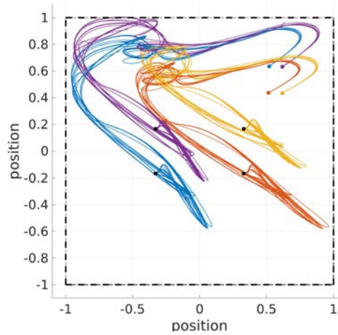
Figure 6.6 – Image feature trajectories planned at different planning steps. Four dashed segments represent the boundaries of the image domain. The image features are initially in the upper right corner.
