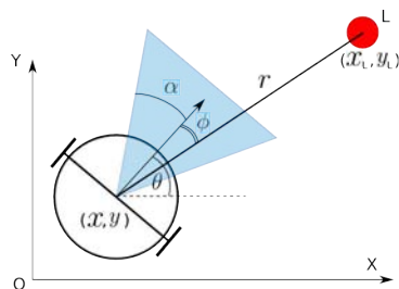
Figure 8.3 – Unicycle and landmark notation.
