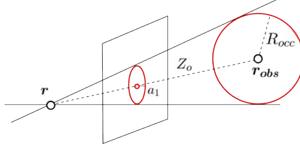
Figure 7.2 – The projection of a sphere on the image plane of a camera at position \mathbf{r} is an ellipse of semi-minor axis a_1 .
