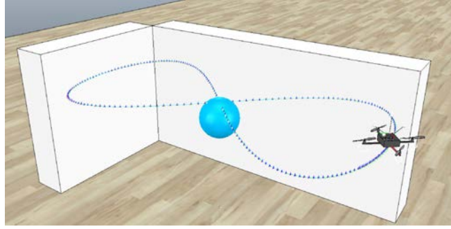
Figure 4.2 – Simulated environment. The blue line represents the lemniscate path to track. The quadrotor has to avoid collisions with a sphere and two walls while keeping a minimal distance with the reference path.
