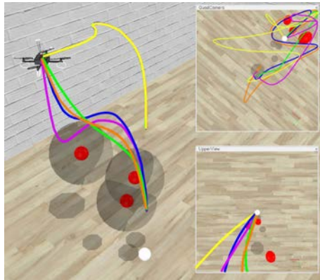
Figure 7.6 – Different solution trajectories returned with different sets of weights (in Table 7.3) in our simulation environment. The camera view is shown in the upper right corner with the image trajectories and a view from above the target is shown below. The orange trajectory uses the chosen values (in Table 7.2) with a higher w_3 . One can observe a faster convergence towards the image center (with an overshoot). The blue one has a higher w_1 resulting in a smoother trajectory than the orange one. The green one is even smoother and is more compliant to occlusions (less jerky) since w_5 is lower. The yellow trajectory is very sharp (low w_1 ) because the occlusion constraints are more respected (high w_5 ) and the final height is less penalized (low w_4 ). The pink solution gives a different and smoother path (high w_1 ) that benefits less from the constraints relaxation (since w_5 is high).
