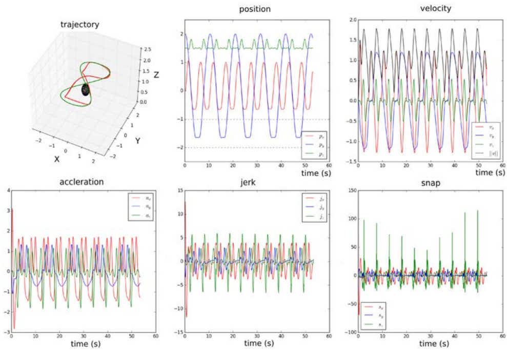
Figure 4.3 – The upper left figure shows the robot path (in red) and the reference path (in green). The obstacles are represented with the black volumes. The other figures show the derivatives of the flat outputs x, y, z .
