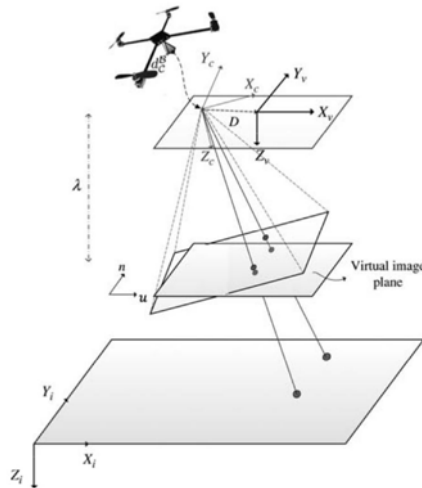
Figure 5.7 – Virtual image plane always parallel to the ground, from [157].
