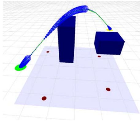
(c) An optimal trajectory exploiting the height of the room to increase the field of view of the camera.
