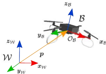
Figure 6.1 – Quadrotor model
