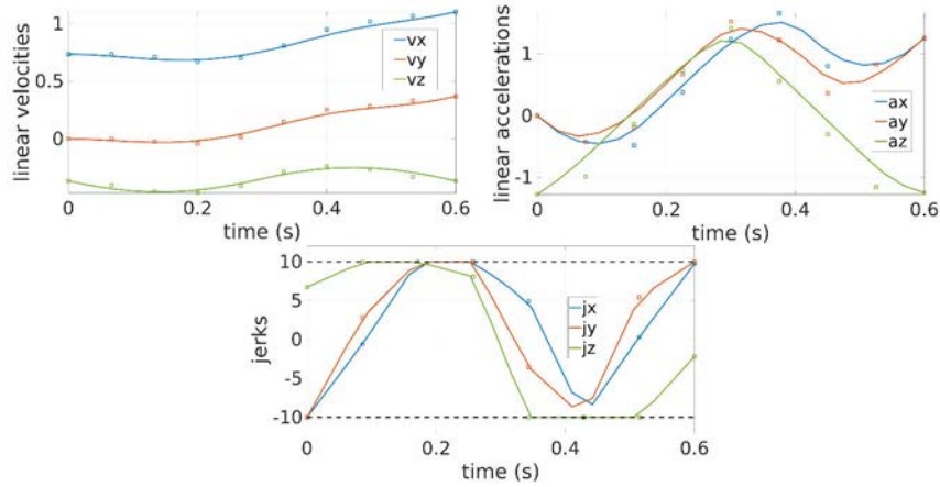
Figure 8.10 – Velocity, acceleration and jerk constraints along the connection trajectory with bounds \bar{v} = 2m.s^{-1} , \bar{a} = 4m.s^{-2} and \bar{j} = 10m.s^{-3} . The small squares represent the B-spline control points.
