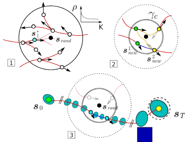
Figure 8.5 – Inside a ball of radius \rho centered at s_{rand} (black dot), picture 1 shows how the vertex with lowest h cost is chosen for expansion (in cyan). The black arrows represent the vertex velocity vector. If vertices from graph \mathcal{G}_1 (in green) and from graph \mathcal{G}_2 (in yellow) are found inside a ball region of fixed radius \gamma_c , connections trials are performed except for connections with a high h cost (orange lines). Note that we consider the opposite velocity (and acceleration) vectors for vertices coming from graph \mathcal{G}_2 . If a candidate connection is found (blue line) the uncertainty is propagated along \mathcal{G}_2 starting from s_0 (picture 3). If no collisions are found between the obstacles (blue box) and the uncertain robot's occupancy (turquoise circles) and if the final constraint (8.9d) is satisfied on \mathbf{P}_N^\eta , a solution trajectory is reconstructed from the initial vertex s_0 (green dot) to the goal vertex s_T (yellow dot) and its total cost is evaluated.
