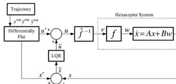
Figure 2.4 – System architecture for LQR control of a hexacopter. A function ( \hat{f}^{-1} ) converts the inputs u to the actual commands \nu fed to the real system (commanded in acceleration with w ) from [28].
