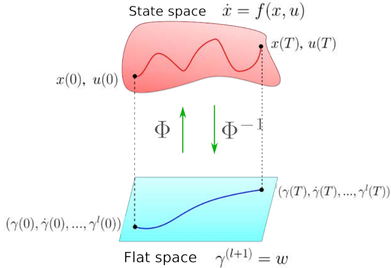
Figure 2.3 – Trajectories in the state space can be mapped in the static flat space (i.e., without dynamics) of lower dimension. Any smooth enough curve in the flat space will be feasible in the state space.
