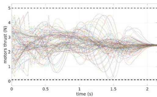
(a) Optimal motor thrusts profiles constrained between 0.1N and 5N.
