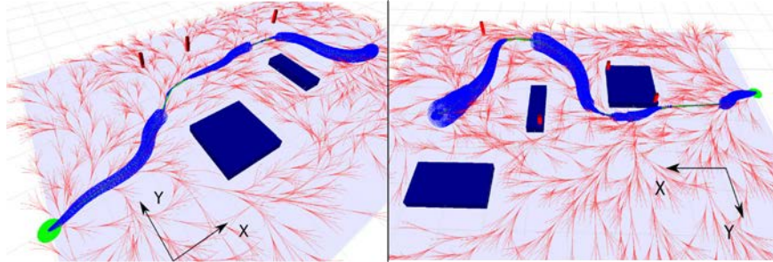
Figure 8.8 – Example trajectories for the unicycle with \tau = 0.3s and u_{max} = 3m.s^{-2} in a 12x8m operating region. The figure on the left shows an optimal trajectory that moves past the landmarks to sufficiently reduce the uncertainty. On the right figure different initial and final states are chosen.
