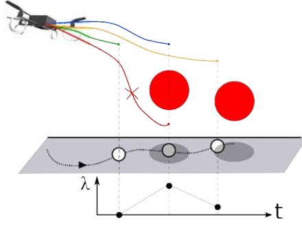
Figure 7.3 – In case of strong and sudden occlusions when the target is below an obstacle, the red trajectory cannot be a viable solution since it may violate actuation and/or spatial constraints. We instead allow minimal constraint violations to keep the solver efficient. The blue trajectory is then a relaxed solution where \lambda hits its limit value R_{occ} (obstacle radius). The orange trajectory represents the case of a less relaxed occlusion constraint where \lambda eventually reaches a smaller value and is zero when there are no occlusions (green trajectory)
