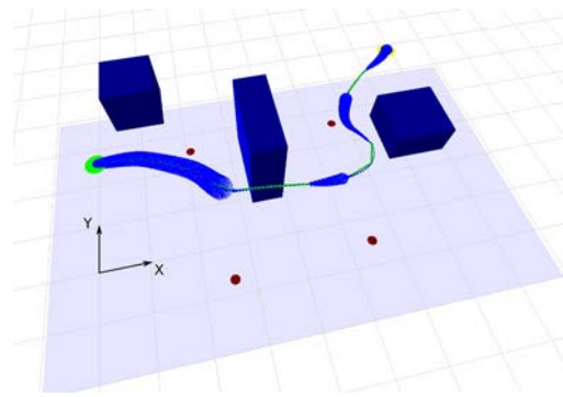
(b) An optimal trajectory starting with a significant uncertainty. A path is found to reduce the uncertainty by collecting visual measurements from three targets.
