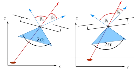
Figure 8.7 – The quadrotor in the vertical planes X-Z and Y-Z with \psi = 0 . Having uncertainties on the state affects the perception. To evaluate if a landmark (red blob) is visible under the state uncertainty we check that condition (8.28) is satisfied on both planes. These conditions allow an exact and fast evaluation of the visibility and only rely on the flat state.
