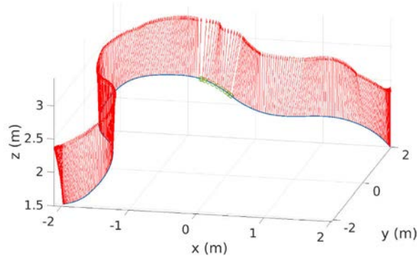
Figure 8.11 – Full trajectory found by the planner. The red arrows represent the total thrust direction and the green circles represent the B-spline coefficients used for connecting the two trajectories.
