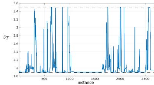
Figure 7.5 – Evolution of z_T for the simulation. The final height was bounded between 1.9m and 3.5m. Again, z_T reaches its minimum value when no collisions and occlusions occur.
