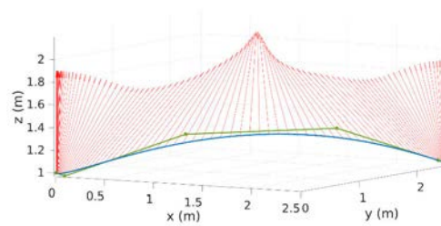
(b) Trajectory (blue line) and total thrust direction (red arrows). The green line represents the convex hull of the spline control points (green dots).
