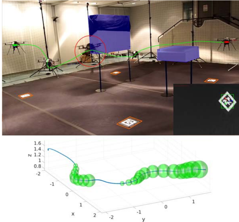
Figure 8.14 – Snapshots of the quadrotor during the experiment. The quadrotor is tracked with a Vicon system and follows an optimal trajectory (in green) along which landmarks (the AprilTags in orange) are visible on some portions. The lower right figure shows an Apriltag tracked using ViSP when the quadrotor is at the configuration circled in red. The evolution of the uncertainty is shown below after running the Kalman filter on the recorded data and using the AprilTags detection. The landmark at the goal is not taken into account in the planning and is used to check that the quadrotor arrives at the goal state within the expected confidence region.
