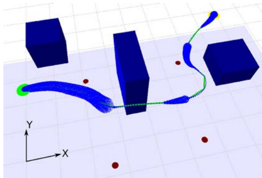
Figure 8.9 – An optimal trajectory for the 3D quadrotor with \tau = 0.35s and u_{max} = 10m.s^{-3} in a 12x8x5m operating region. The initial and final states are chosen such that no landmark is visible (red blobs on the ground) so the quadrotor starts with some uncertainty and is able to reach the goal with a bounded uncertainty by observing the landmarks during its motion. Note that we do not consider occlusions due to the obstacles and the motion primitives are not shown.
