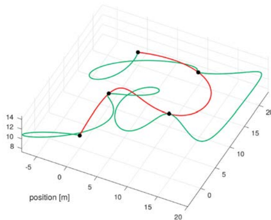
Figure 8.2 – A minimum snap (red) passing through waypoints and a trajectory (green) yielding well-observable states. This trajectory is much longer and much more complex, from [206].
