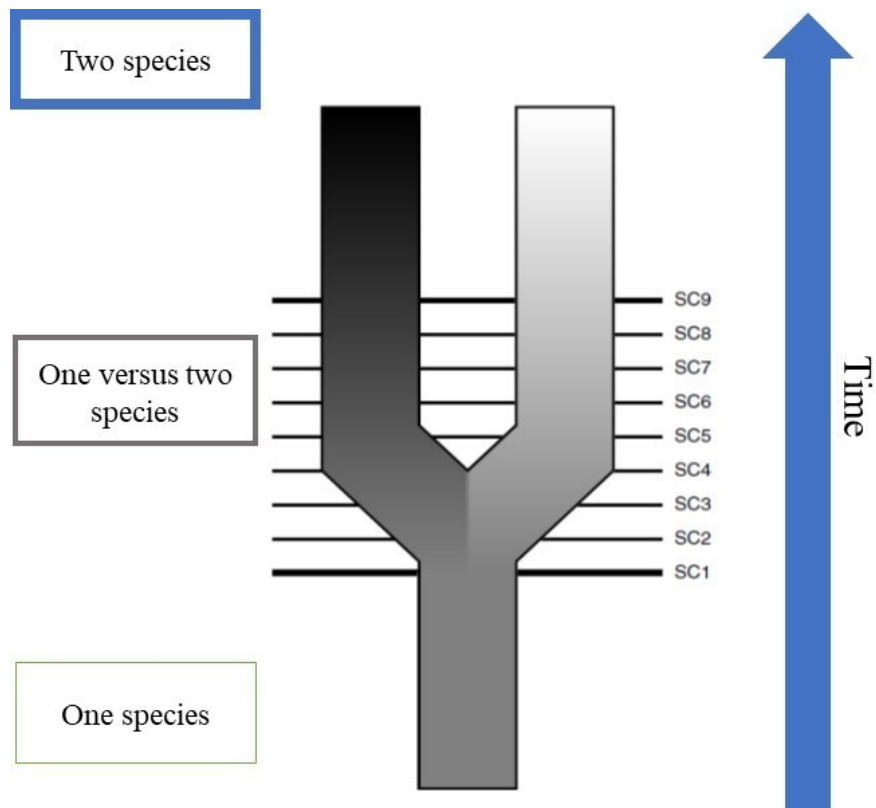
Figure 2 : A simple illustration of speciation process after De Queiroz (2007). At first one species exists and with time it splits into two species. The SC1 to SC9 correspond to the progression of time.
