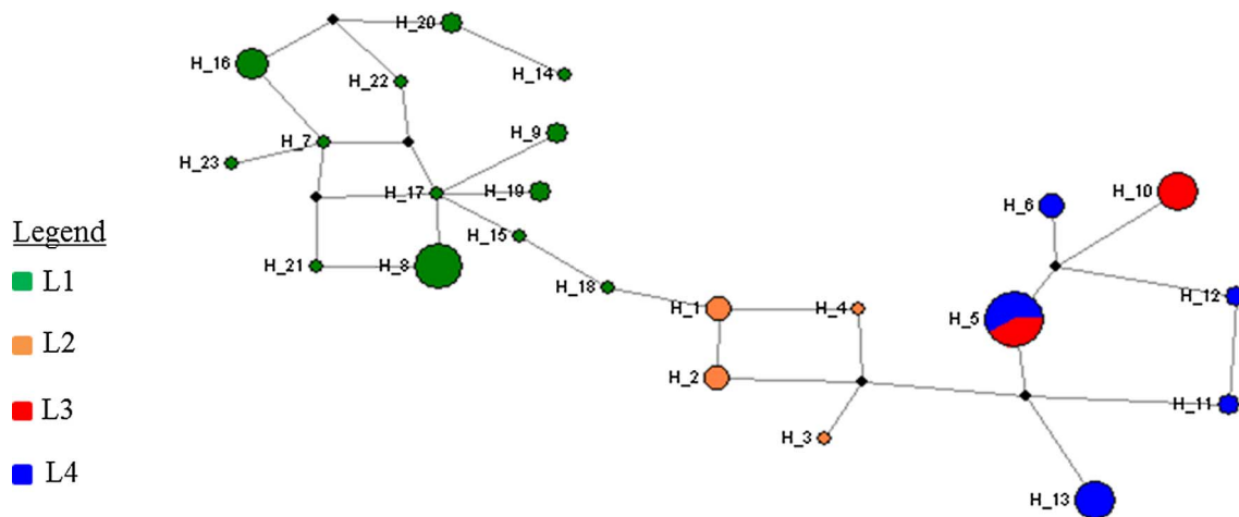
Fig. 4. ITS2 marker haplotype network of the four main P. corethrurus lineages after phasing. Color codes for lineages are the same as in Fig. 3. (For interpretation of the references to color in this figure legend, the reader is referred to the web version of this article.)
