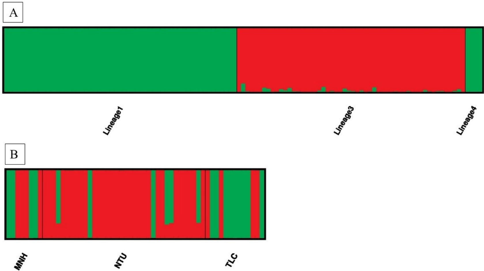
Figure C 2: Structure results on AFLP profiles: A) unknown individuals assignment based on 'reference' data in Taheri et. al. (in revision), colors are selected based on the previous study; Lineage 1 green and L3 red, B) mixture model results for three populations where sympatry of cryptic species were found; MNH, NTU and TLC.
