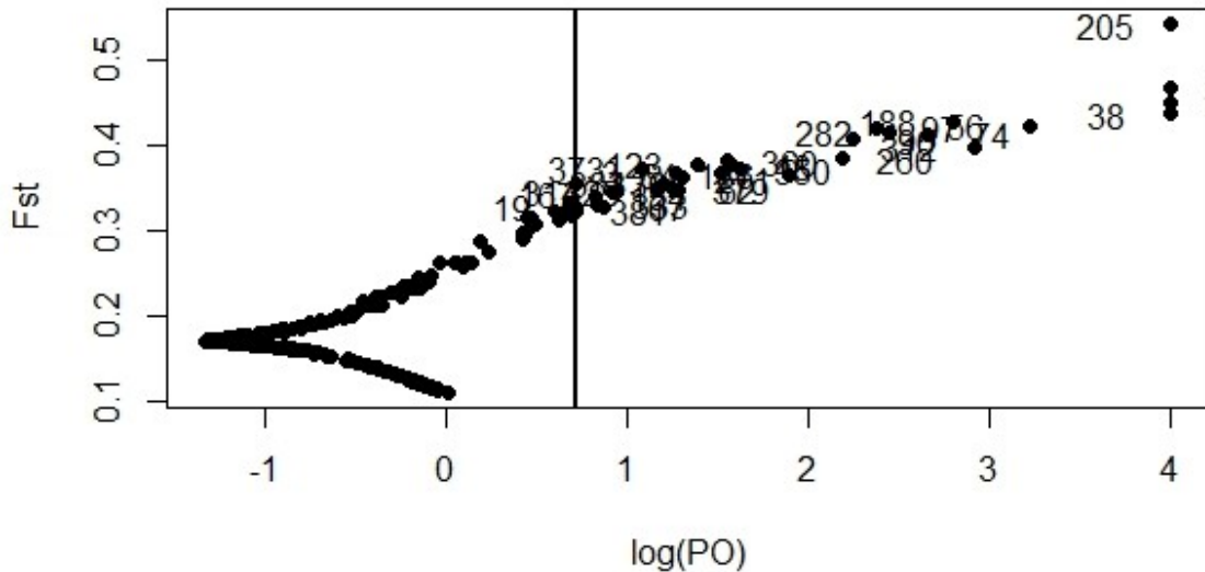
Figure C 4: Bayescan results done on AFLP profiles. F_{ST} is plotted against the \log_{10} of the posterior odds (PO). The vertical line shows the critical PO used for identifying outlier markers. The 33 markers (out of 394) on the right side of the vertical line are candidates for being under selection for P. corethrus L1 specimens.
