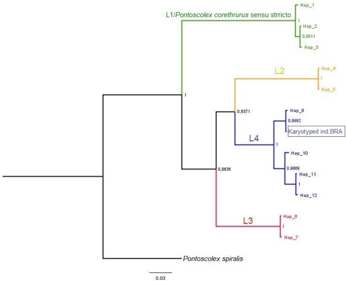
Figure D 5: Bayesian tree for COI gene of Pontoscolex corethrus complex. The karyotyped individual ( 2n=70 ) from Embrapa's garden in Brazil, corresponded to L4 of this complex.
