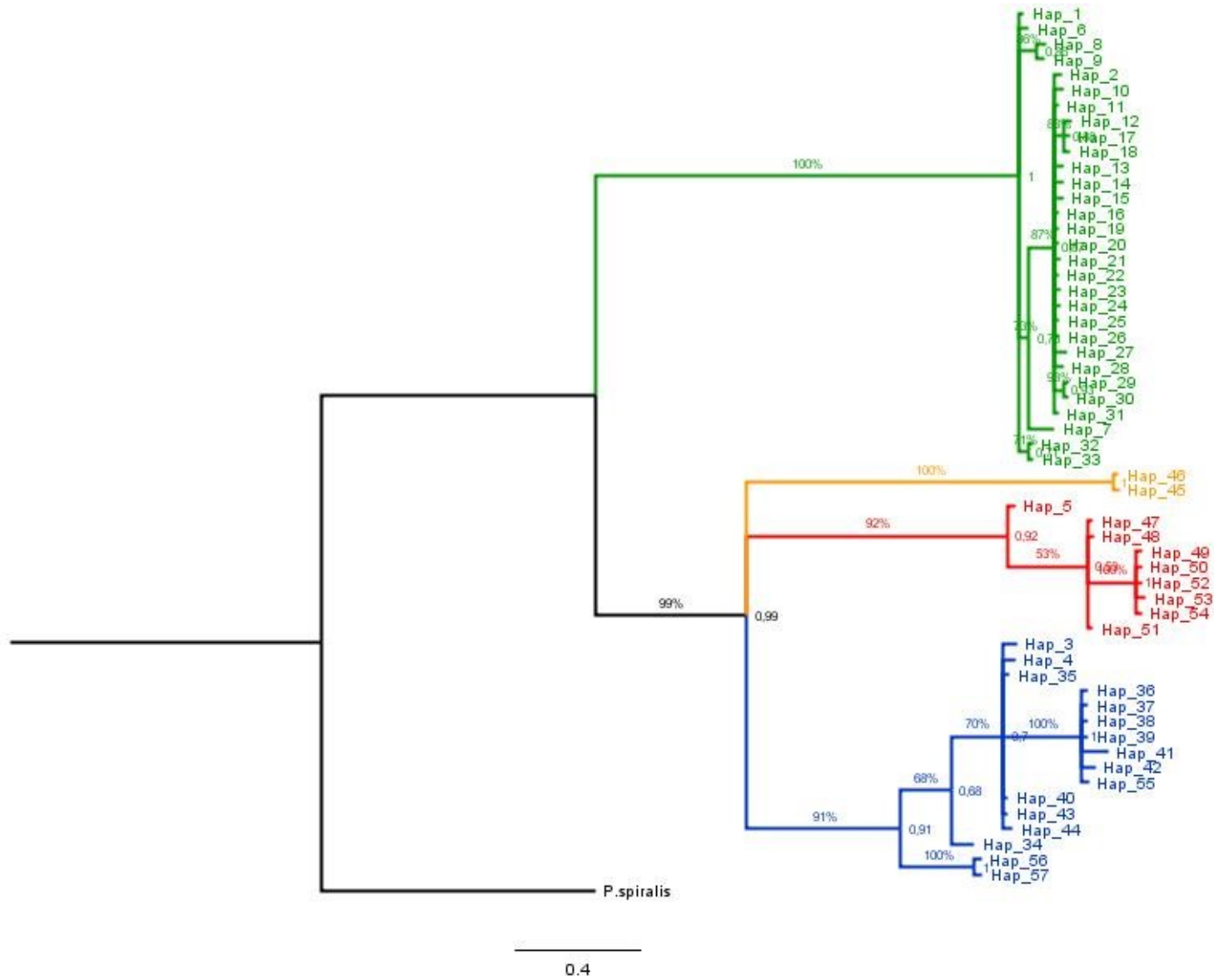
Figure C 6: Maximum-Likelihood tree based on HKY+G substitution model, with 662 COI sequences of P. corethrurus complex specimens.
