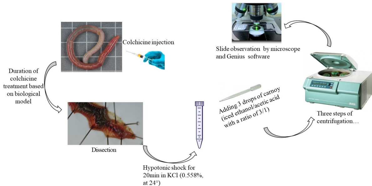
Figure D 3: The steps of protocol 3. The first step is colchicine injection (image on top left), the volume of injected colchicine depends on animal's weight i.e., 0.3 ml of 0.04% colchicine for 100 grams. Duration of colchicine treatment depends on the biological model used. KCl 0.558% at 24°C was used as hypotonic shock. Carnoy was added to stop the shock and to fix the chromosomes, then three steps of centrifugations were run. At the end, slides were observed under microscope to investigate chromosomes at metaphase stage.
