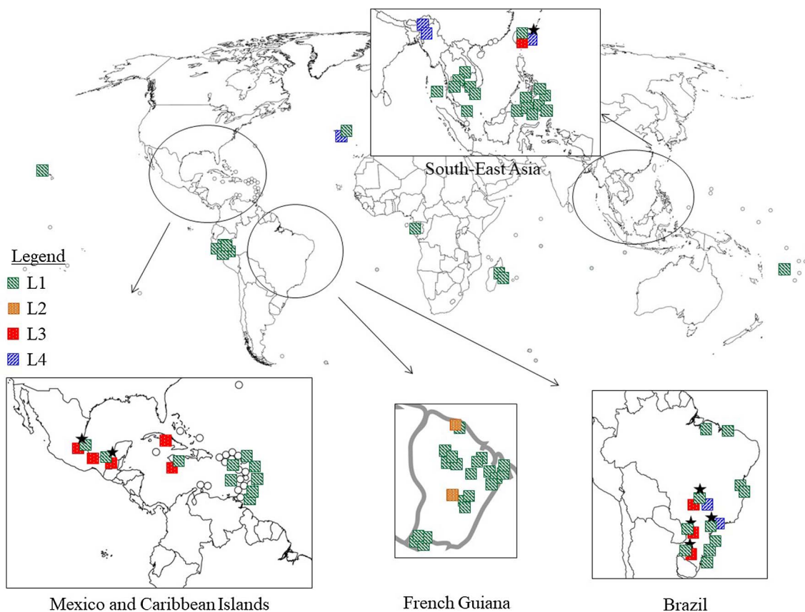
Fig. 2. Cryptic lineages in Pontoscolex corethrurus . Mexico and Caribbean islands, French Guiana, Brazil and South-East Asia are magnified in the squares. Cryptic lineages are shown by different colors: L1 (green lineage), L2 (orange), L3 (red) and L4 (blue). L1 is the most widespread lineage. Sites with sympatry of cryptic lineages are marked by a star. Refer to Appendix for more information on the sampled sites within each country. (For interpretation of the references to color in this figure legend, the reader is referred to the web version of this article.)
