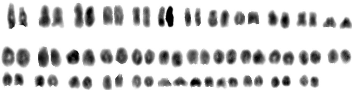
Figure D 6: First karyotype obtained based on protocol 3, from seminal vesicles of an adult specimen in L4 of Pontoscolex corethrus complex within Embrapa population. The ploidy degree is diploid; 2n=70 .
