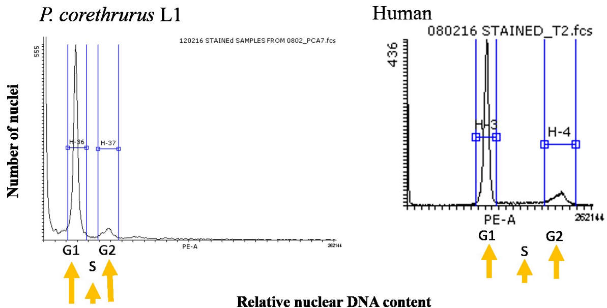
Figure 4: Flow cytometry results obtained by Luis Cunha, for pineapple plantation individuals of P. corethrurus L1, from Azores Island. Analyses were done based on coelomocytes cavity of specimens. Results suggested that P. corethrurus L1 is diploid.
