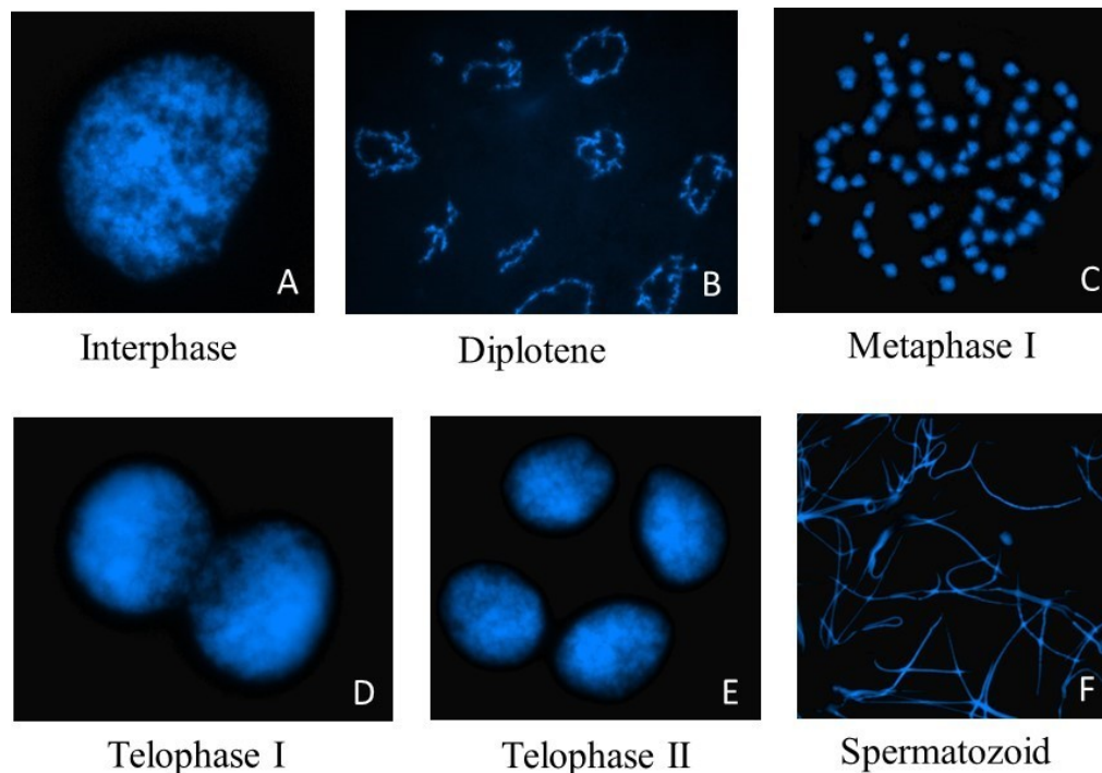
Figure D 7: Meiosis stages of two individuals in Pontoscolex corethrurus complex, one individual in L4 and the other one is unknown due to sequencing problem. These results were obtained on seminal vesicles organ (slide colorations are done by DAPI).
