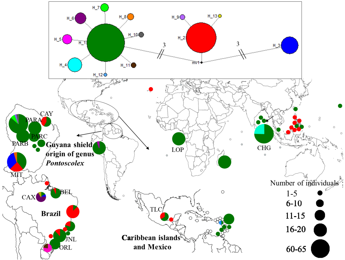
Figure C 3: P. corethrurus L1 COI haplotype network based on 479 sequences in 49 locations, throughout the tropical zone. 72% of specimens have the same haplotype (H1). Twelve populations for which population genetic analyses based on COI and AFLP profiles are done, are indicated with abbreviations under the related haplotypes. The intensity of each haplotype is related to the number of individuals within a location. Each line represents one mutation among haplotypes, unless they are indicated.
