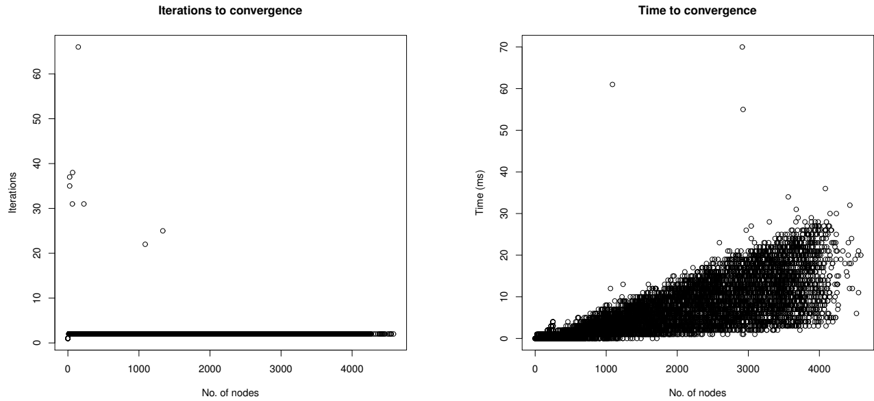
Figure 3.20: The benchmark consisting of the KR + ECAI dataset with all weights equal to 1.0.
