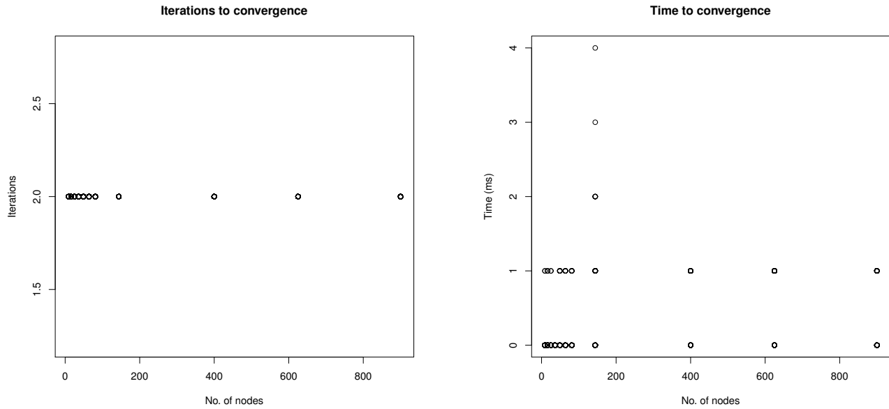
Figure 3.18: The Kleinberg dataset of the Perugia benchmark with all weights equal to 1.0.
