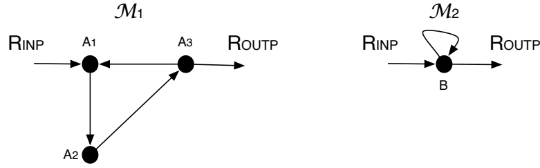
Figure 2.16: Two multipoles that can be safely interchanged under ideal semantics (Example 20).
