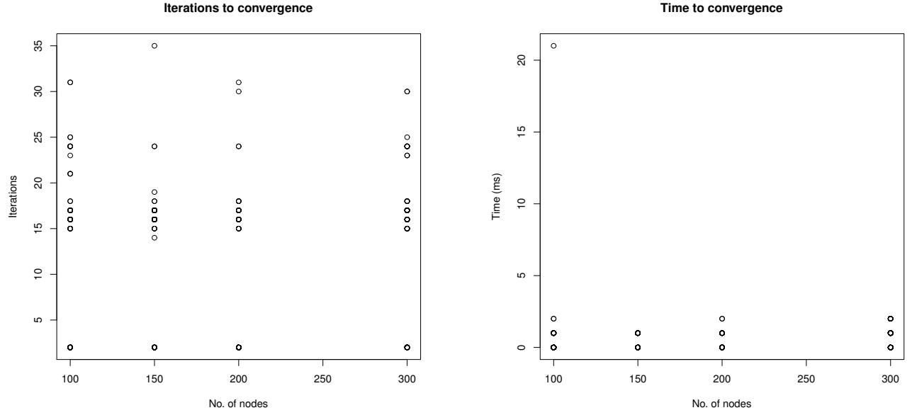
Figure 3.16: The Erdős-Rényi dataset of the Perugia benchmark with all weights equal to 1.0.
