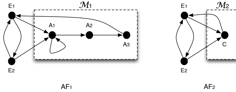
Figure 2.13: A contextually PR -legitimate replacement (Examples 15 and 17).
