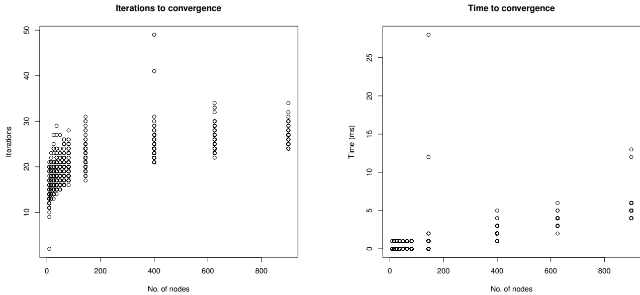
Figure 3.19: The Kleinberg dataset of the Perugia benchmark with random weights.
