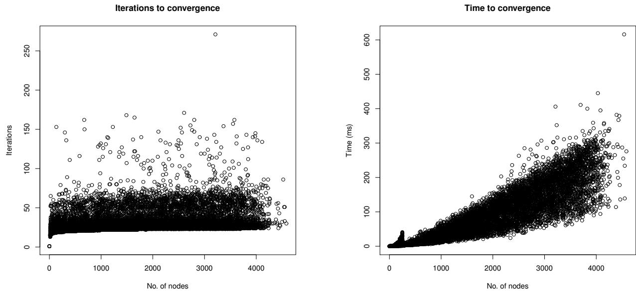
Figure 3.21: The benchmark consisting of the KR + ECAI dataset with random weights.
