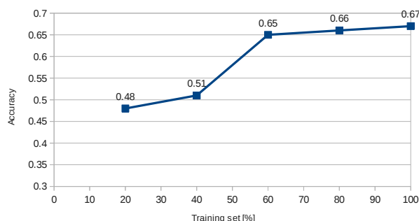
Figure 5.3: EDITS learning curve on Debatepedia data set
