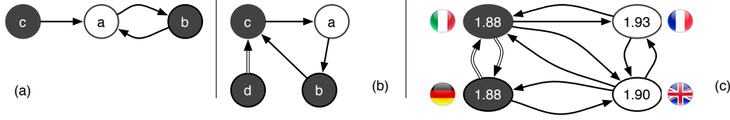
Figure 4.2: Example of (a) an AF , (b) a bipolar AF , and (c) example provided in the introduction modeled as a bipolar AF , where single lines represent attacks and double lines represent support.
