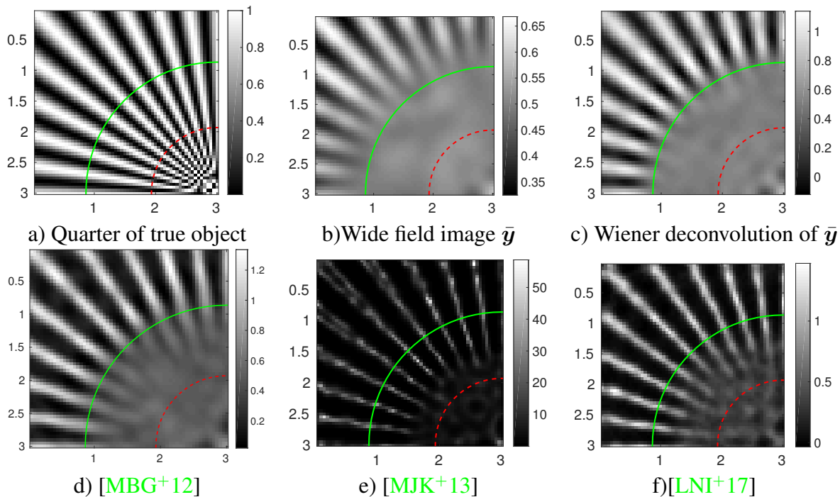
Figure 2.2 – Joint reconstruction approach in blind-speckle-SIM using different regularizers with 300 speckle patterns and 40dB Gaussian noise. d) is obtained using positivity constraint as shown in [MBG + 12], e) is obtained with \ell_{2,0} norm regularizer using M-SBL algorithm as in [MJK + 13] and f) is obtained with \ell_1 + \ell_2 norm regularizer plus positivity constraint using PPDS algorithm shown in [LNI + 17].
