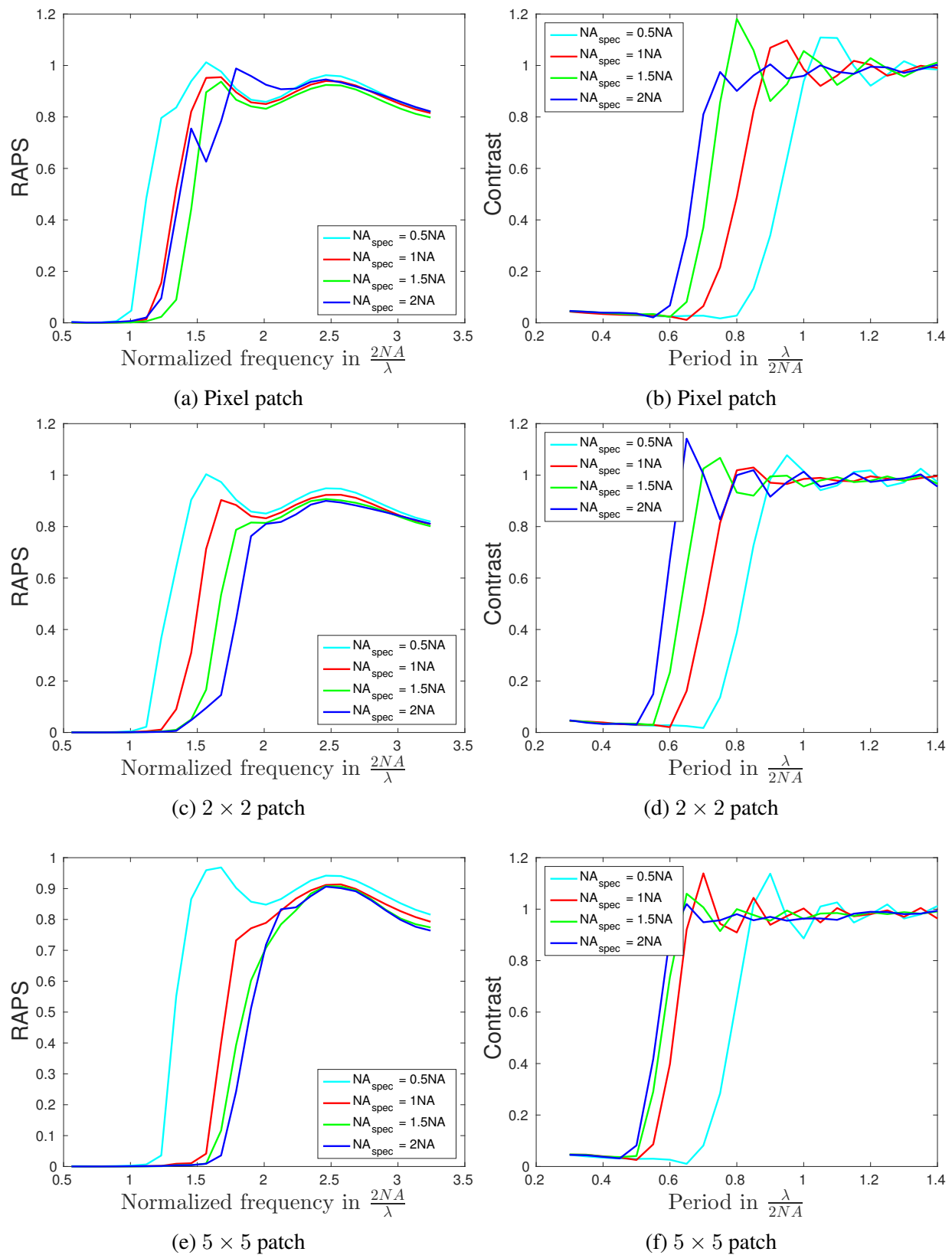
Figure 4.7 – Normalized RAPS curves for error images as a function of the frequency (first column) and MCF of the reconstructed objects as a function of the period (second column) with varying support of speckle patterns.
