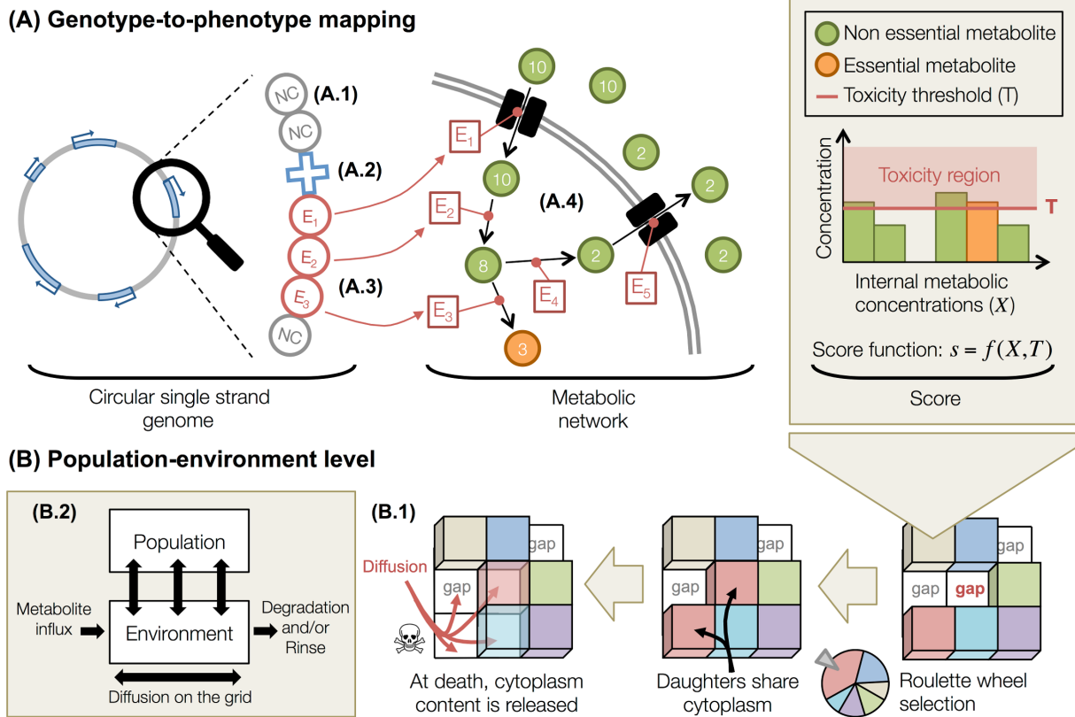
Figure IV.1 – Presentation of the model. The genotype-to-phenotype mapping, as well as the population and environment, are schematized here. (A) Description of the genotype-to-phenotype mapping. Organisms own a coarse-grained genome that contains genomic units. (A.1) Non-coding units (NC, grey circles) are not functional. The arrangement of the genomic units on the circular single strand defines functional regions, where a promoter (P, blue cross, A.2 ) controls the expression of all contiguous enzyme units (E, red circles), thereby allowing for operons. (A.3) When enzyme units are expressed, they contribute to the metabolic network. (A.4) Enzymes perform metabolic reactions in the cytoplasm, or pump metabolites in or out (see the description of the metabolic network below). The score of an organism is computed from its “essential metabolites” (see the description of the score function below). Lethal toxicity thresholds are applied to each metabolic concentration and preclude organisms to accumulate resources. (B) Description of the population and environment levels. Organisms are placed on a 2D toroidal grid, and compete for resources and space. (B.1) When an organism dies, it leaves its grid spot empty and organisms in the Moore neighborhood (if any) compete to divide in the available spot. The competition is based on scores, a minimal threshold being applied on scores to preclude worst organisms to divide. At division, daughters share cytoplasm content (enzymes and metabolites). At death, metabolites from the cytoplasm are released in the local environment and diffuse on the grid. (B.2) At the largest scale, the population evolves in the environment by uptaking, transforming and releasing metabolites. Metabolites then diffuse and are optionally degraded. This interaction between the population and its environment allows for the evolution of complex ecological situations.
