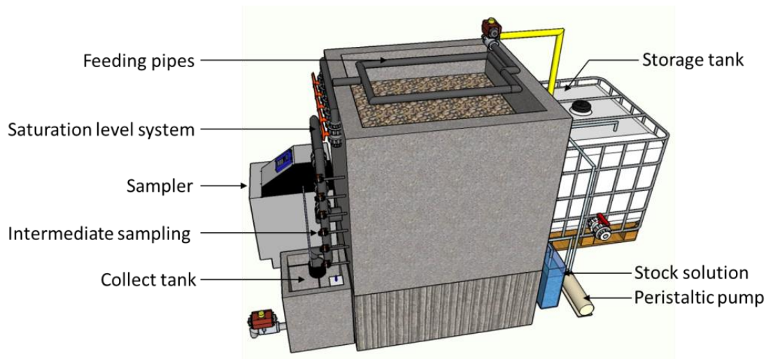
Figure 31 Experimental setup
