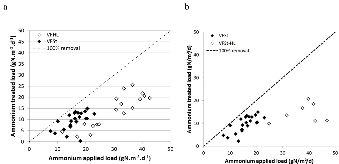
Figure 20 Ammonium treated loads according to the ammonium applied loads for pilots receiving the same average concentration of ammonium but operating under different hydraulic loads (VFHL: 0.64 \text{ cm.d}^{-1} and VFSt: 0.36 \text{ cm.d}^{-1} ) (a) and for pilots receiving different average concentration of ammonium (VFSt: 43.6 \text{ mgN.L}^{-1} and VFSt-HL: 103.7 \text{ mgN.L}^{-1} ) but operating under identical hydraulic loads (b).
