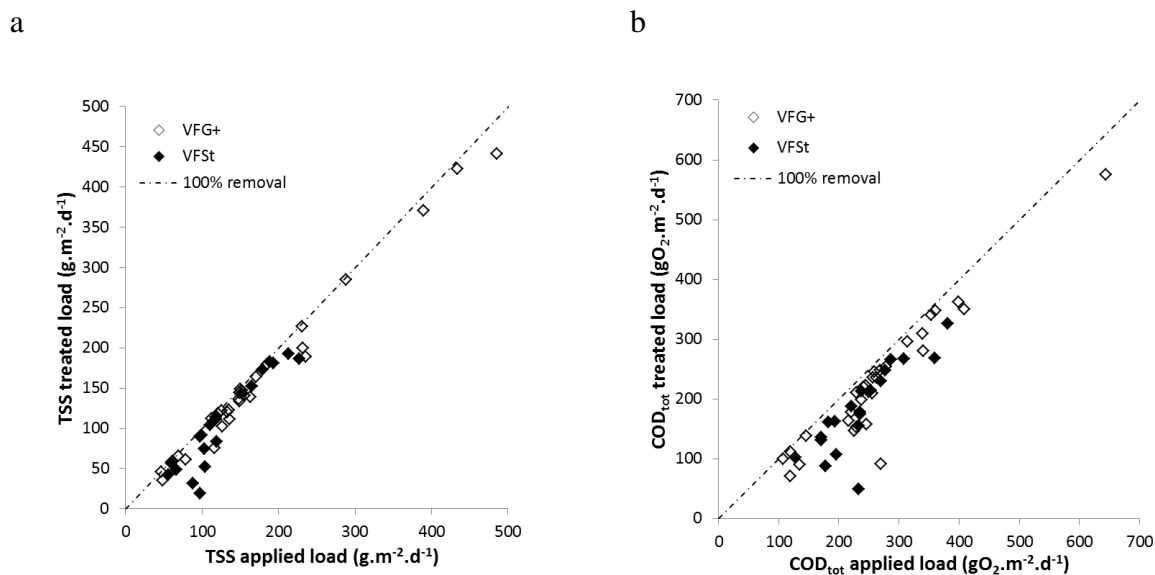
Figure 16 Treated TSS (a) and COD tot (b) loads according to the applied TSS and COD tot loads, respectively
