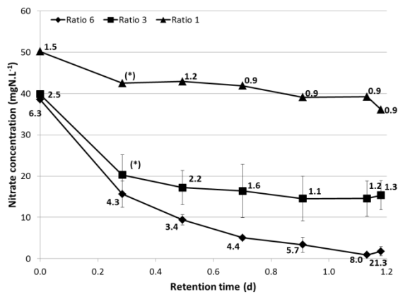
Figure 29 Nitrate (a) and COD_{tot} (b) SVFP outlet concentration in relation to retention time for different COD_{tot}:N ratio ( C_{in} = 40mgNO_3-N.L^{-1} ). Note that COD_{tot}:N ratios are presented for each retention time in front of each data (* means that the ratio cannot be determined).
