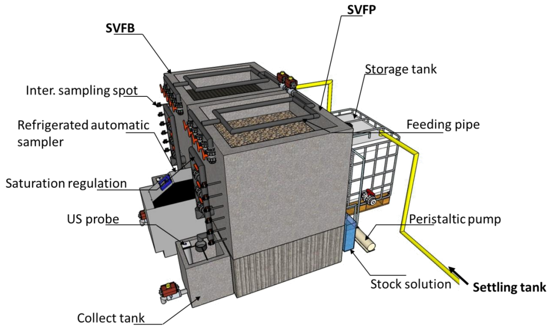
Figure 24 Experimental setup
