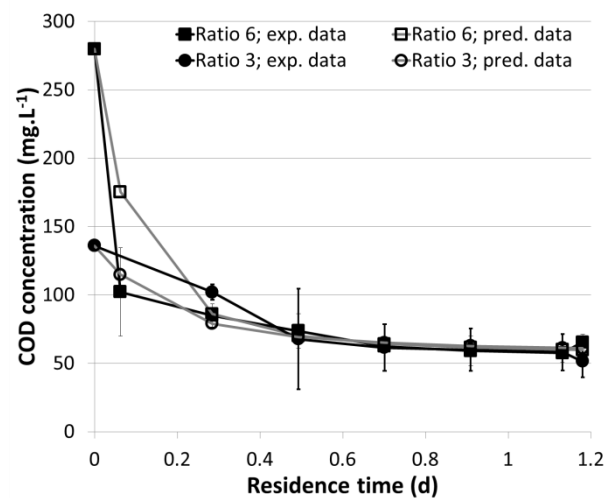
Figure 36 Experimental and predicted values of nitrate (a) and COD (b) concentrations against residence time at COD:N = 6 and 3
