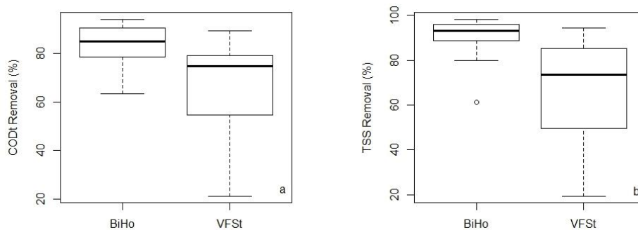
Figure 62 CODt (a) and TSS (b) removal performances
