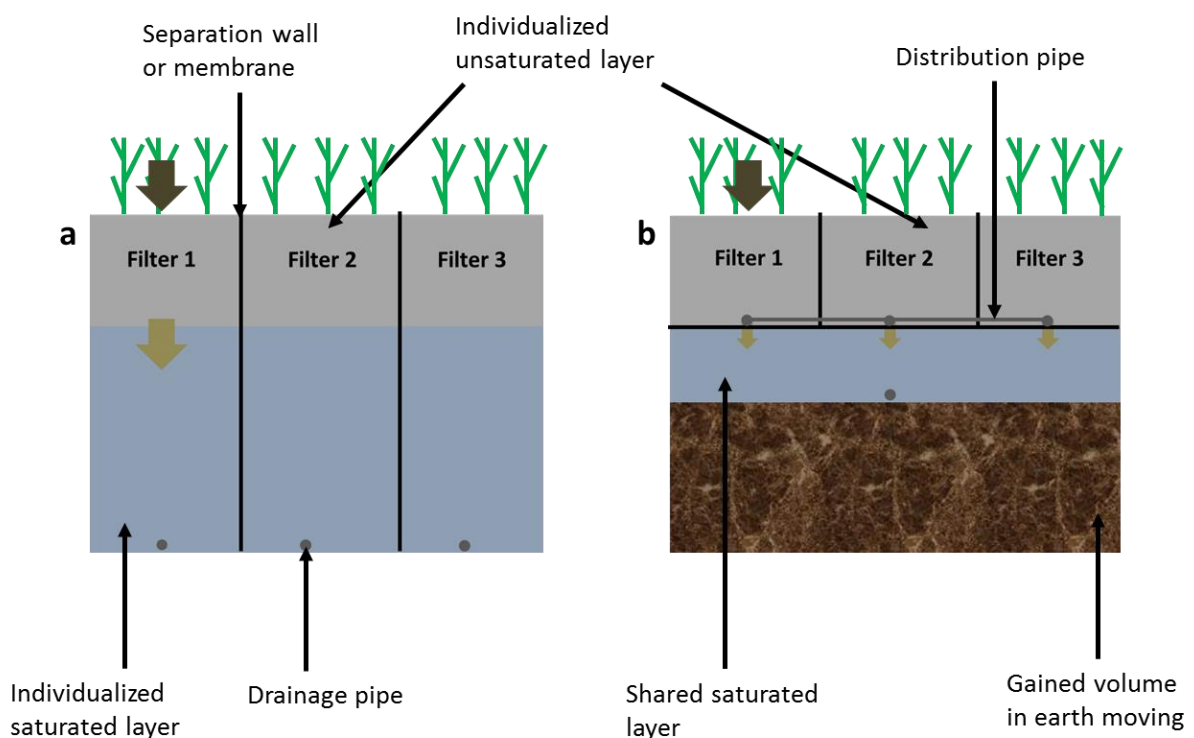
Figure 58 Schematic description of usual design (a) and proposed design (b) of partially saturated filters
