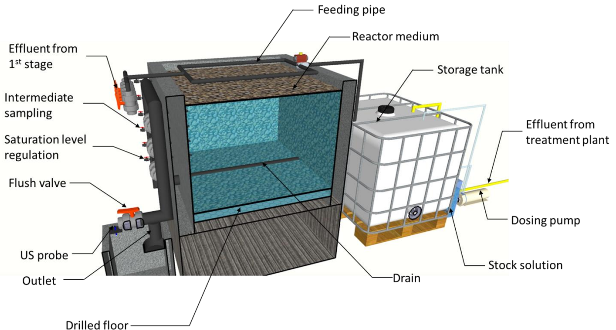
Figure 68 Schematic cross section of a saturated vertical pilot
