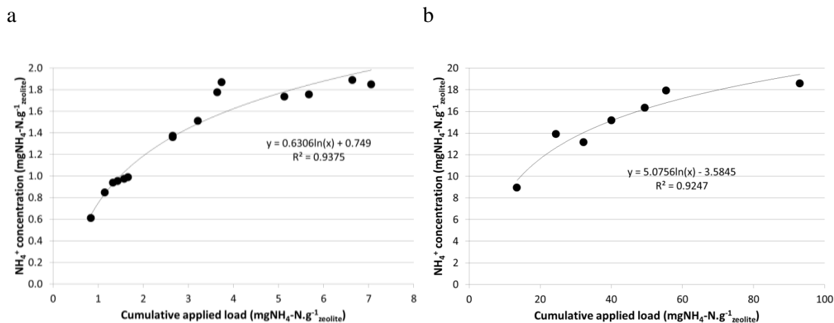
Figure 56 Ammonium concentration in solid phase regarding to the cumulative applied load for columns treating ammonium influent concentration of 100mgNH 4 -N.L -1 (a) and 2000mgNH 4 -N.L -1 (b)
