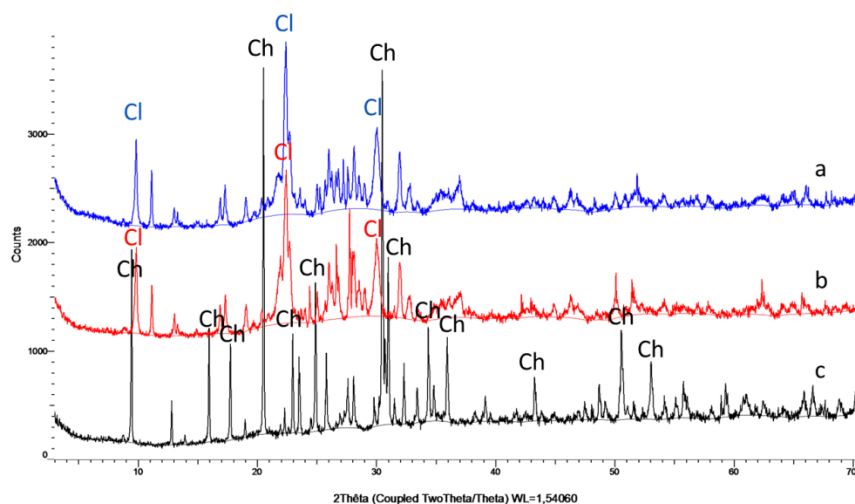
Figure 41 XRD patterns of Turkish clinoptilolite (a), Spanish clinoptilolite (b) and Italian chabazite (c)
