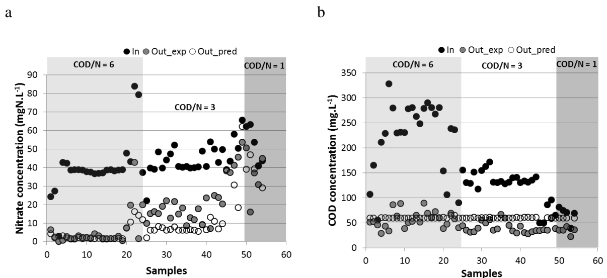
Figure 38 Nitrate (a) and COD (b) measured and predicted concentrations for residence time of 1.18d
