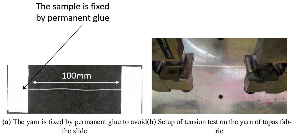
FIGURE 1.8 – Tension test on the yarn of tapas fabric
