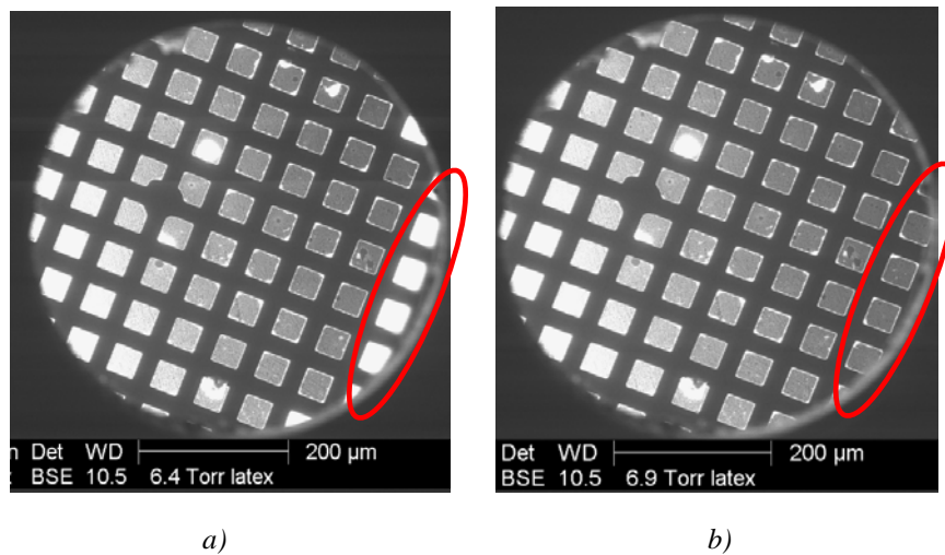
Figure 7. Images of latex SBA-PMMA acquired with setting temperature at 5 °C, under different chamber pressure: a) 6.4 Torr, b) 6.9 Torr
