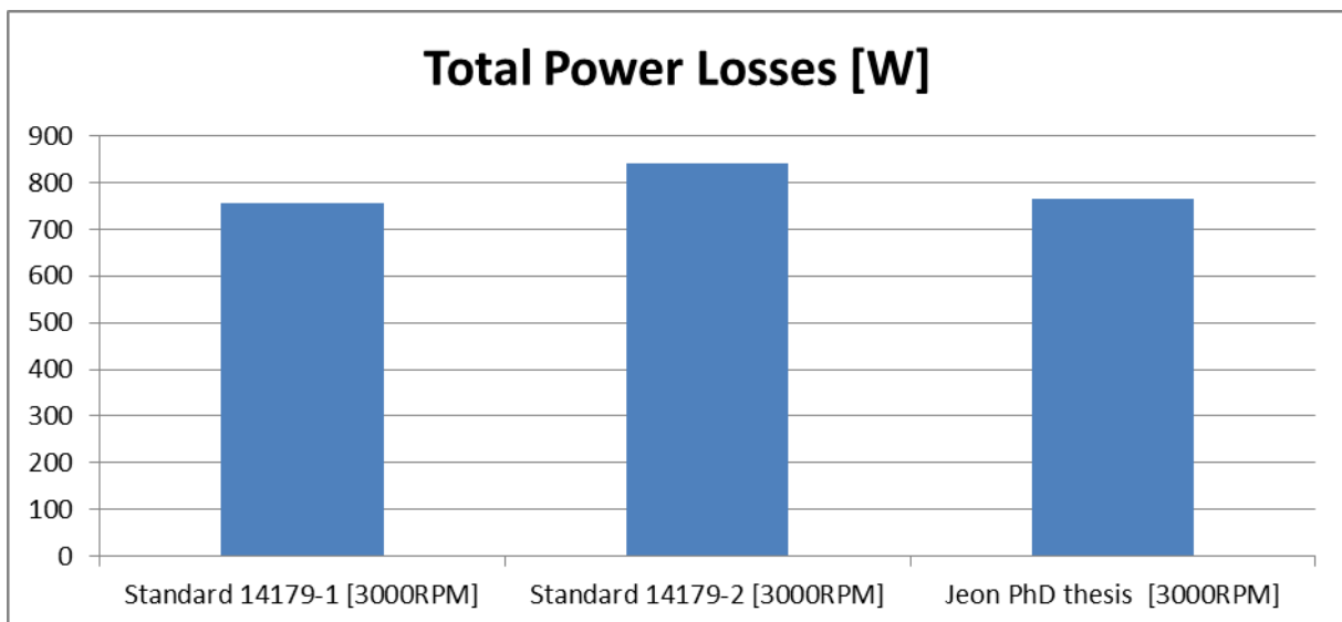
Figure 17: total power losses for various churning formula from 14179-1, 14179-2 and Jeon PhD thesis
