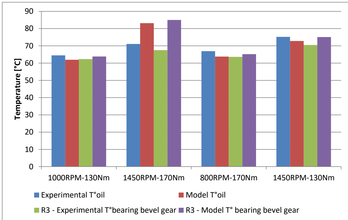
Figure 63: comparison between experimental and model temperature
