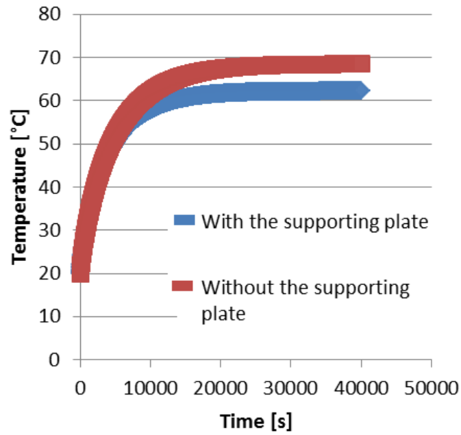
Figure 75: oil temperature evolution – 1000 RPM and 130 Nm
