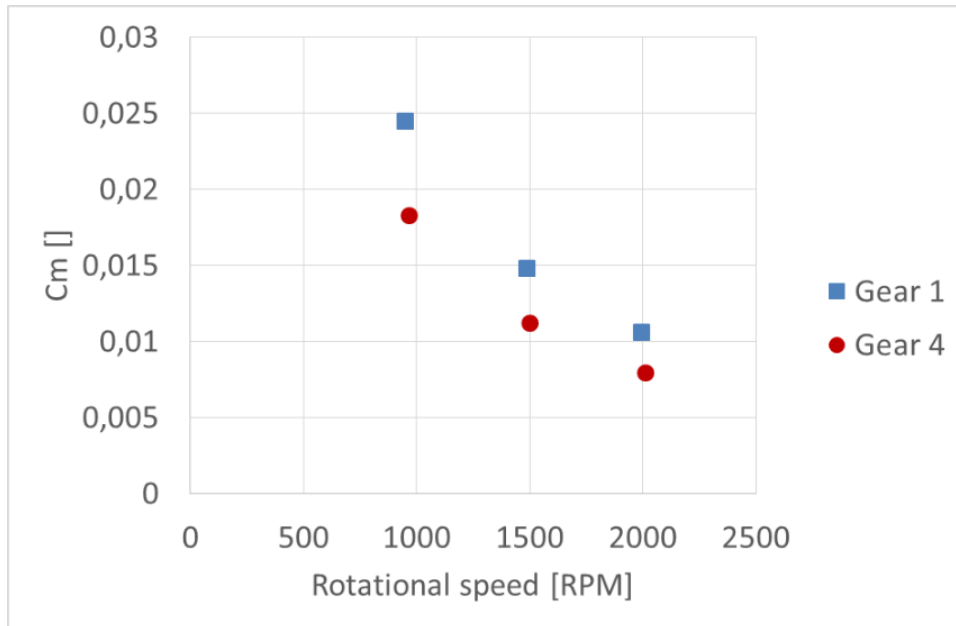
Figure 33: C_m for gears 1 and 4 according to equation II.1 (oil B, 70°C, h/h_0=0.5 )
