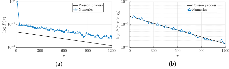
Figure 7.2: PDF of waiting times between two consecutive fluctuations of amplitude a = 2.5 , estimated from a timeseries of length T_d = 10^6 of the Ornstein–Uhlenbeck process (7.1) with \alpha = 1 and \epsilon = 1/2 (blue triangles), and assuming the events follow a Poisson process with rate 1/r(a) , P(\tau) = e^{-\tau/r(a)}/r(a) (black solid line), where r(a) is computed from the timeseries. The correlation time of the Ornstein–Uhlenbeck process is \tau_c = 1/\alpha = 1 . (a) Taking all intervals into account, including those corresponding to oscillations around the threshold. (b) Discarding small intervals ( \tau < \tau_c ) linked to oscillations around the threshold.
