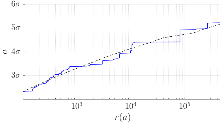
Figure 7.8: Illustration of the computation of return times for the averaged drag over the square obstacle in test flow (2). The averaging window is 5 correlation times. The dashed black line represents the reference return times computed from a timeseries spanning 10^6 correlation times, using (7.8). The solid blue line represents the return times obtained using the CKTL algorithm.
