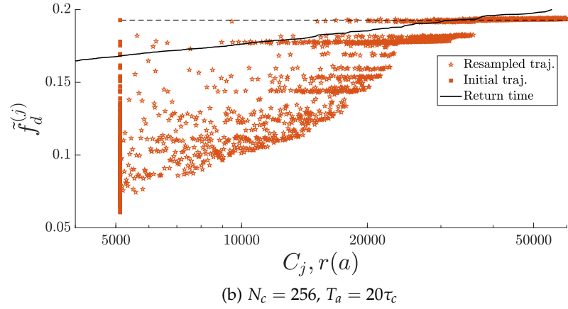
Figure 6.8: Maximum of the instantaneous drag along the resampled trajectories, denoted by \tilde{f}_d^{(j)} , as a function of the corresponding computational cost C_j , defined in (6.17). In both figures, the TAMS is iterated until extinction. The solid black line indicates the typical fluctuation amplitude a as a function of the corresponding return time r(a) . It is the typical timescale of occurrence of fluctuations above a . Furthermore, the square markers depict the maximum \tilde{f}_{d,n}^{(0)} , 1 \leq n \leq N_c over the initial trajectories. This figure illustrates that in both experiments the TAMS does not improve the sampling of rare fluctuations. One can see that the maximum values among the resampled trajectories concentrates on values already sampled over the initial trajectories. Eventually, extinction is reached as the algorithm is unable to generate a fluctuation higher than the maximum fluctuation in the initial ensemble of trajectories. This behaviour is illustrated in figure 6.9 on the basis of the drag timeseries involved in the experiment of figure 6.8a.
