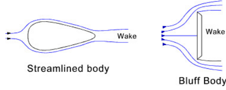
Figure 3.1: Typical examples of streamlined and bluff bodies. Blue lines represent the trajectory of fluid particles, referred to as streamlines (see note 3). In the case of the streamlined body, streamlines stay attached to the surface of the obstacle. As a result, the spatial extent of the wake is diminished, and a high pressure is recovered at the downstream point of the body. By contrast, the important cross flow section of bluff bodies entails a flow separation, as the trajectory of fluid particles detach from the surface of the body. As a result, the pressure near the downstream surface of the obstacle is considerably lower than the pressure near the upstream surface, resulting in a large drag.
