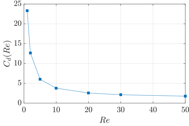
Figure A.2: Drag coefficient as a function of the Reynolds number. The estimate from pipeLBM is compared to reference values from [20], showing good agreement. Re = 50 , U_0 = 0.01 , D_y = 129 , D_x = 385 , R = 16 .
