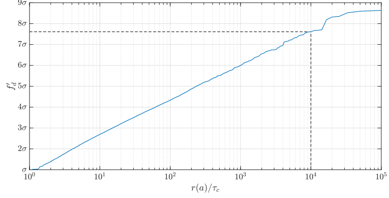
Figure 3.3: Return time plot for the instantaneous drag fluctuations based on a timeseries of duration T_{tot} = 10^5 \tau_c for test flow (2). The fluctuation is defined as f'_d = (f_d - \bar{f}_d)/\sigma with \bar{f}_d the average and \sigma the standard deviation computed over the timeseries. It illustrates that a return time r(a) = 10^4 \tau_c corresponds to fluctuations of order a \approx 7.6\sigma . The computation of such plot is described in chapter 7.
