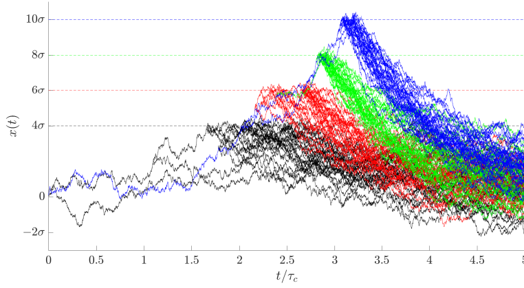
Figure 6.6: Ensemble of N_c = 32 trajectories at four different iterations j , for which \mathcal{Q}_j^* > a with a = 4\sigma, 6\sigma, 8\sigma and 10\sigma .
