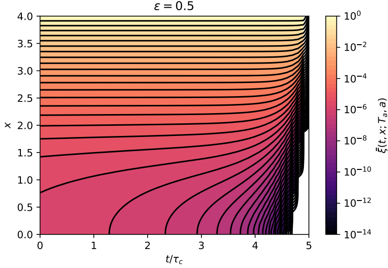
Figure D.1: Contour lines of the time-dependent committor \bar{\xi}(t, x; T_a, a) for the Ornstein-Uhlenbeck process (with \alpha = 1, \epsilon = 1/2 ; in particular \tau_c = 1 ), obtained by solving numerically the backward Fokker-Planck equation (D.2), with a = 4, T_a = 5 .
