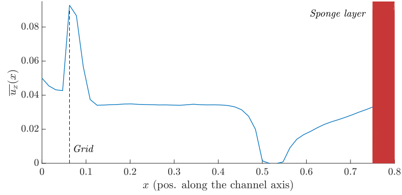
(a) Average velocity profile along the channel axis
