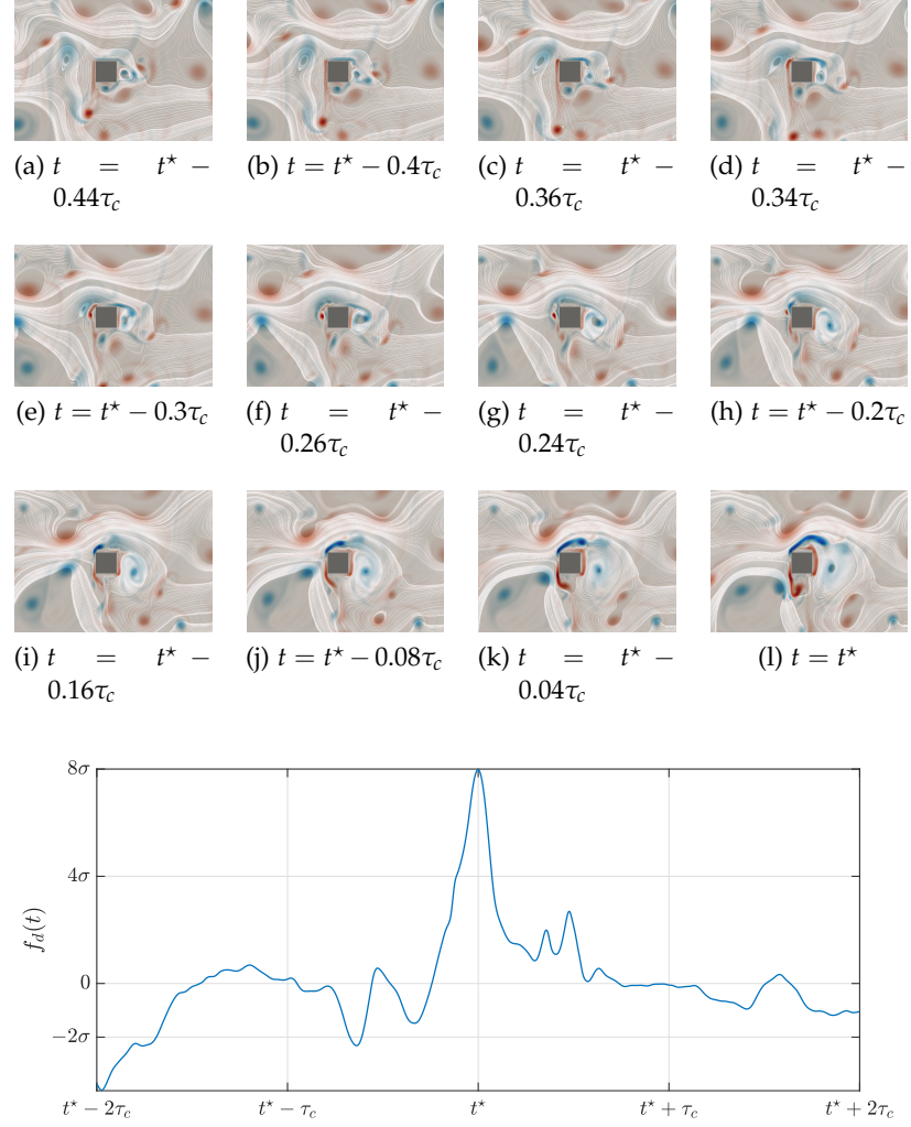
(m) Evolution of the drag f_d over time, centred on the extreme fluctuation at t = t^*
