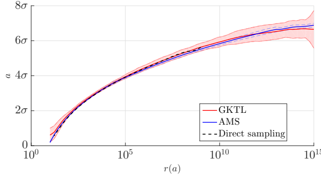
Figure 7.6: Return time plot for the time-averaged Ornstein-Uhlenbeck process \bar{X}_T (7.15) with \alpha = 1 and \epsilon = 1/2 ( \sigma = 1/\sqrt{2} is the standard deviation), estimated from the GKTL algorithm (solid red line) and AMS algorithm (solid blue line). The GKTL algorithm was used with N_c = 500 replica, T_a = 20\tau_c and k = 0.9 . It was repeated K = 100 times. The TAMS algorithm was used with N_c = 100 replicas, T_a = 50 and a = 6.5\sigma_T . It was repeated K = 10 times. Finally, the dashed black line represents the result of a direct sampling over a timeseries of length T_d = 10^9\tau_c . Parameters of both the GKTL and AMS algorithms were chosen so that 100 realisations of the algorithms amount to a computational cost of \mathcal{O}(10^6\tau_c) . The cost of the direct sampling is 10^9\tau_c . The shaded area represents the confidence interval on the estimation of the fluctuation amplitude a , for a fixed value for the return time r(a) . It is computed as the empirical mean over the 100 interpolated return time plots originating from the 100 independent realisations of the algorithm.
