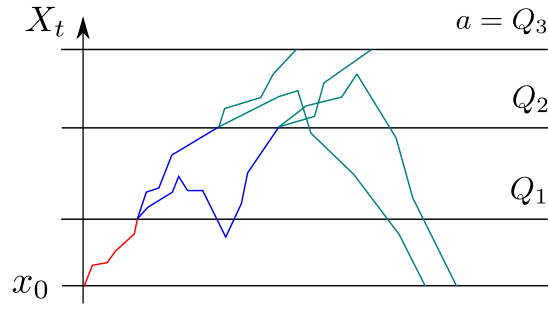
Figure 6.1: Illustration of the multilevel splitting strategy. From initial condition x_0 , there is a very little probability that the process X_t will reach the level a before falling back to the typical region around x_0 . A straightforward way of computing such a probability is to compute many realisations and count how many succeed to reach a . Naturally, as the event X \geq a is very rare, this would require a tremendous amount of realisations. Instead, splitting methods suggest to decompose the fluctuation into a finite number of intermediate fluctuations. First X \geq Q_1 , then X \geq Q_2 | X \geq Q_1 and finally X \geq Q_3 | X \geq Q_2 , where A|B denote the realisation of A conditioned on the realisation of B . In this way, each intermediate event is much more likely to occur and its probability easier to compute. Generally, the process is duplicated upon reaching a given level Q_i . The choice of the levels and the number of replicas depends on the specific splitting method in use.
