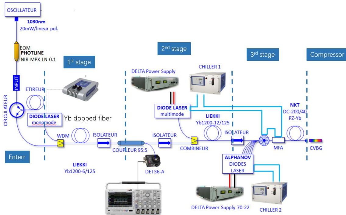
Figure 4.5 Amplifier for the S-Box cavity from CELIA [134] . There are three amplification stages.
