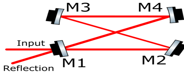
Figure 4.1 Schematic illustration of the S-Box cavity (prototype cavity for ThomX).
