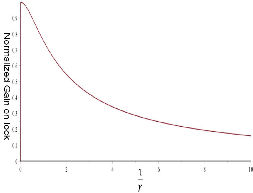
Figure 2.10 Normalized gain under locking as a function of 1/\gamma .
