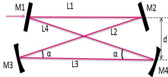
Figure 5.3 Schematic diagram of a 4M 2D bow-tie cavity.
