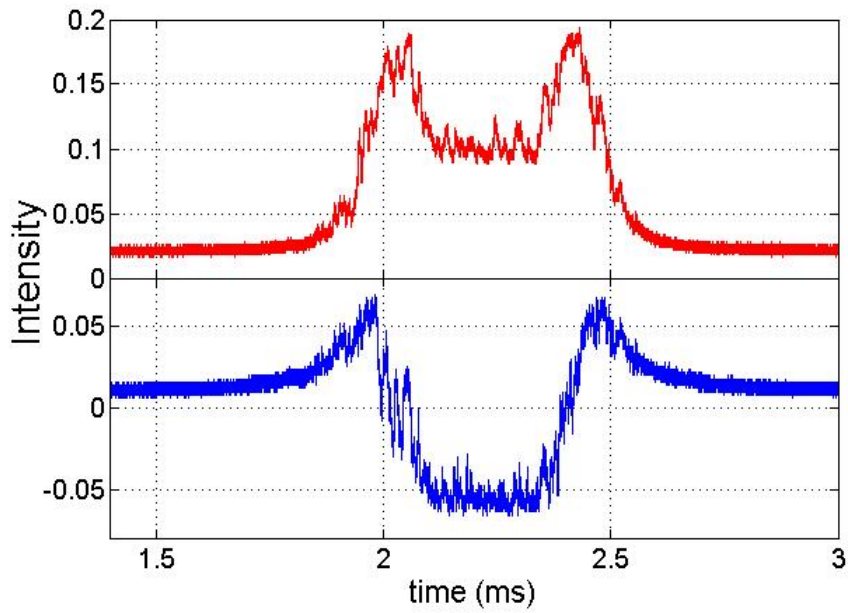
Figure 3.15 Experimental measurement. When PZT of the laser is adjusting the frequency, the intensity of transmission (top red curve) and error signal (bottom blue curve) are obtained.
