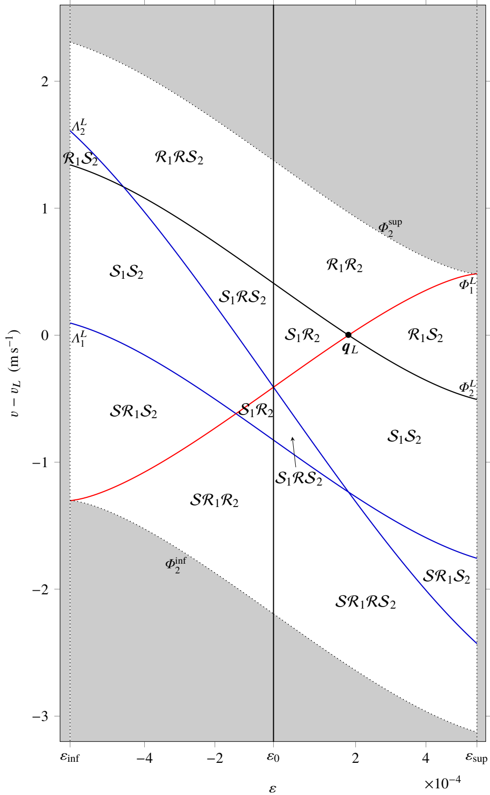
Figure 3.7. Case \epsilon_L > \epsilon_0 . Admissibility regions and hyperbolicity domain (white) for the polynomial law (2.22) with a cubic nonlinearity and the parameters from Table 2.1. Here, \epsilon_L = 1.8 \times 10^{-4} .
