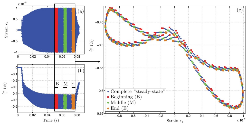
Figure 1.2. Dynamic acousto-elastic testing of Berea sandstone. (a) Evolution of the axial strain \varepsilon at the location of the probe over time. (b) Relative variation \Delta c/c of the sound speed with respect to its initial value over time. (c) Hysteresis loop: \Delta c/c versus \varepsilon in steady state. Reproduced from [118] (Fig. 12), with permission of AIP Publishing.
