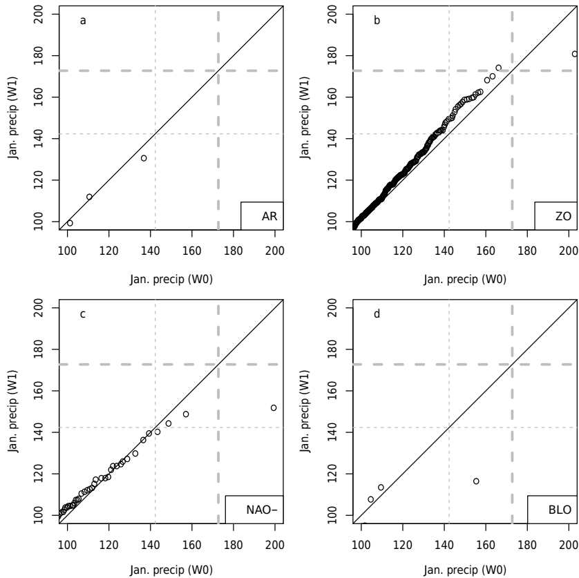
Figure 6. Quantile–quantile plots of January precipitation (in mm month −1 ) probability distributions between counterfactual ( \mathcal{W}_0 ) and factual ( \mathcal{W}_1 ) worlds in Weather@Home simulations, for each weather regime ( a : Atlantic Ridge; b : zonal; c : NAO−; d : Scandinavian blocking). The continuous line is the first diagonal. The thick dashed lines indicate the observation in January 2014. The thin dashed line indicates the 99th quantile of observed January precipitation.
