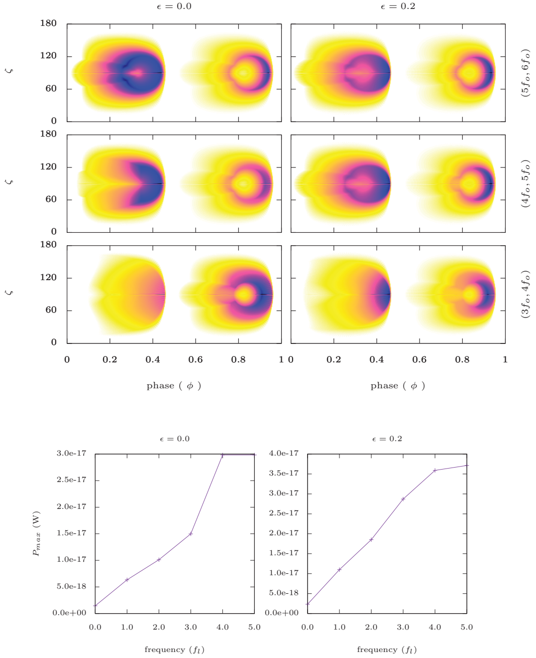
Figure B-17: Top : Frequency resolved radio emission for (\alpha, \beta, \delta) = (90^\circ, 45^\circ, 90^\circ) . The x -axis and y -axis represent phase ( \phi ) and line of sight angle ( \zeta ) respectively with the former being normalized to one. The panels on left and right are for the centred case \epsilon = 0 and for the off centred case \epsilon = 0.2 respectively. The lowest plot is for frequency range (f_l, f_u) = (3f_o, 4f_o) and top most is for (5f_o, 6f_o) ; each increasing in steps of f_o (value in Table. B.2). The white region corresponds to region with no emission and moving towards blue-black via yellow-orange signifies an increase in the power emitted. Bottom : The x -axis represent the lower frequency f_l of the frequency range increasing in steps of f_o and the y -axis shows the power radiated corresponding to the unit with highest power, P_{max} (in W), which is chosen to normalize the power emitted in phase plots in top panels.
