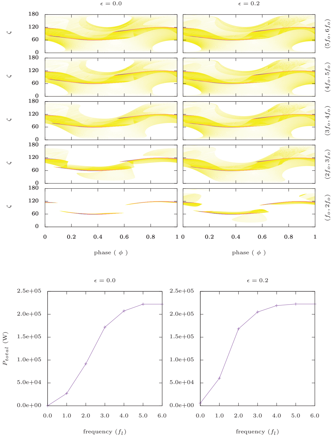
Figure 4-17: Top :Frequency resolved radio emission for (\alpha, \beta, \delta) = (30^\circ, 0^\circ, 0^\circ) for \gamma = 10^5 - 10^7 . The x -axis and y -axis represent phase ( \phi ) and line of sight angle ( \zeta ) respectively with the former being normalized to one. The panels on left and right are for the centred case \epsilon = 0 and for the off centred case \epsilon = 0.2 respectively. The lowest plot is for frequency range (f_l, f_u) = (f_o, 2f_o) and top most is for (5f_o, 6f_o) each divided in equal intervals f_o . The white region corresponds to region with no emission and moving towards blue-black via yellow-orange signifies an increase in the power emitted. Bottom : The x -axis represent the lower frequency f_l of the frequency range increasing in steps of f_o and the y -axis shows the total power emitted summed up for each individual emission diagram in the top panel, P_{total} (in W).
