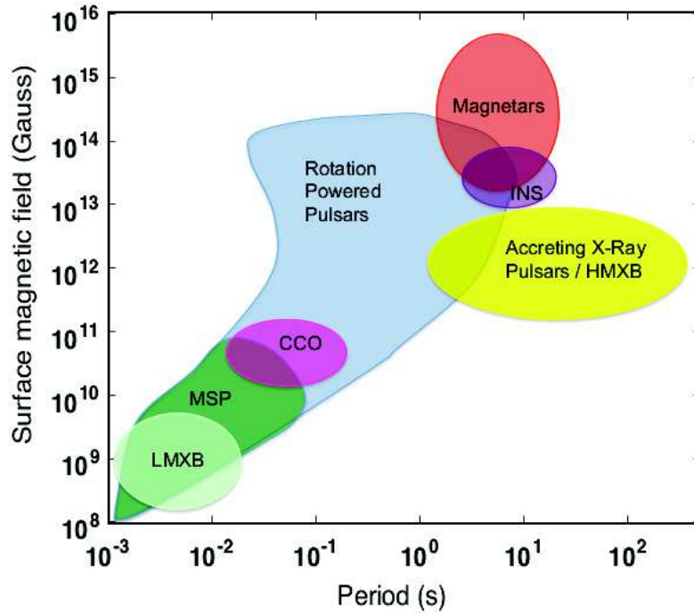
Figure 1-5: Schematic diagram of neutron star populations with respect to their periods and derived surface magnetic field strengths (Harding, 2013).
