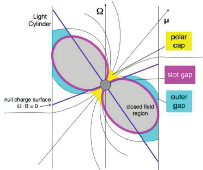
Figure 1-11: A schematic representation of the different geometric pulsar models (Harding (2005))
