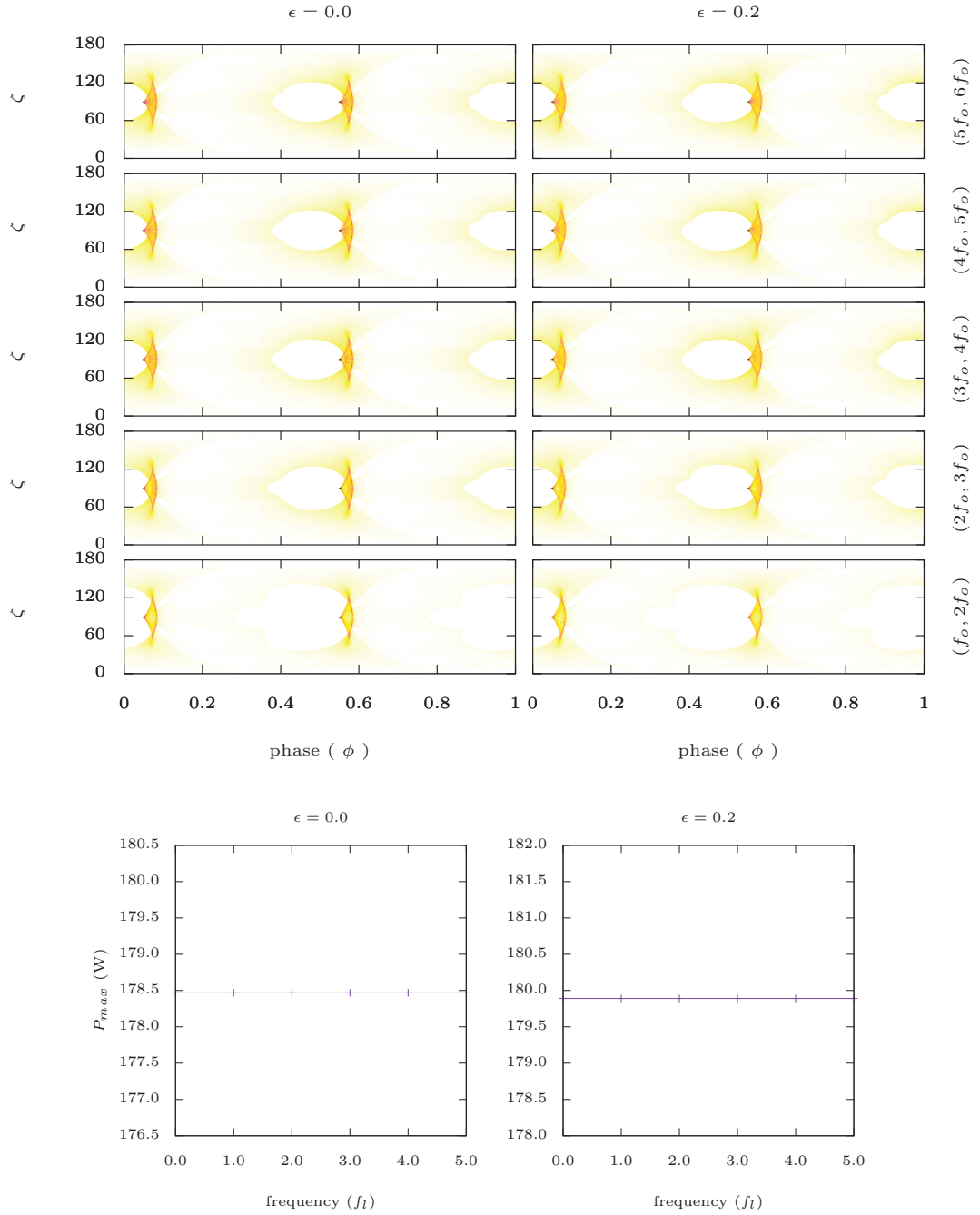
Figure B-3: Top : Frequency resolved high energy emission for (\alpha, \beta, \delta) = (90^\circ, 0^\circ, 0^\circ) . The x -axis and y -axis represent phase ( \phi ) and line of sight angle ( \zeta ) respectively with the former being normalized to one. The panels on left and right are for the centred case \epsilon = 0 and for the off centred case \epsilon = 0.2 respectively. The lowest plot is for frequency range (f_l, f_u) = (f_o, 2f_o) and top most is for (5f_o, 6f_o) ; each increasing in steps of f_o (corresponding energy values in Table. B.1). The white region corresponds to region with no emission and moving towards blue-black via yellow-orange signifies an increase in the power emitted. Bottom : The x -axis represent the lower frequency f_l of the frequency range increasing in steps of f_o and the y -axis shows the power radiated corresponding to the unit with highest power, P_{max} (in W), which is chosen to normalize the power emitted in phase plots in top panels.
