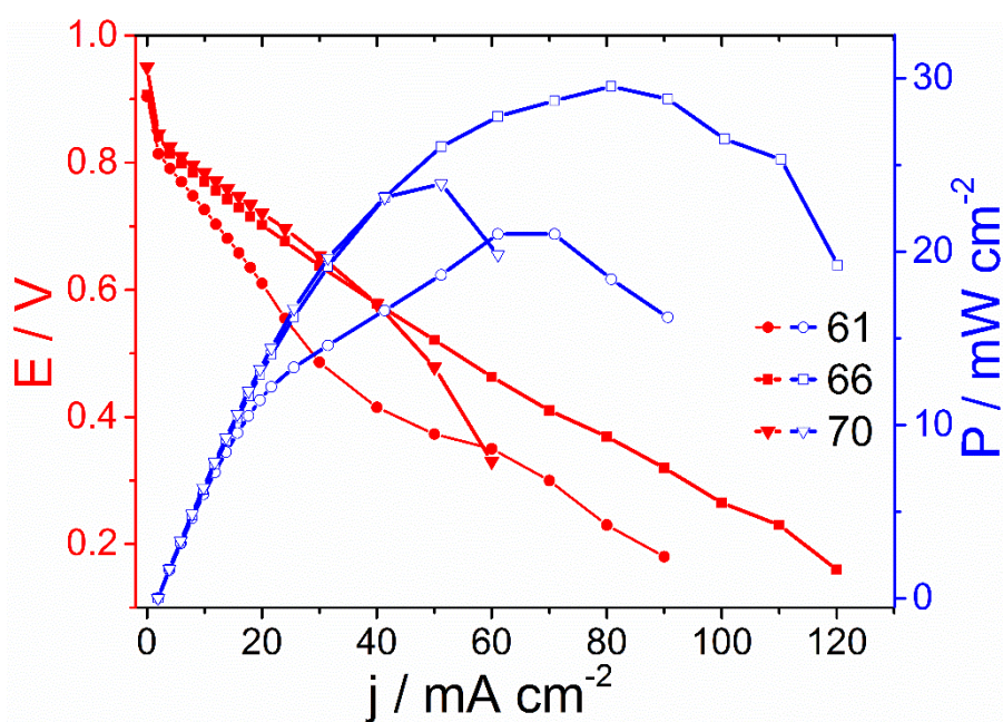
Figure V.5 Polarization and power density curves of SAFC obtained using CCM-3 as MEA at different working temperatures. Temperature of anode and cathode humidifiers: 56 \text{ }^\circ\text{C} , flow rate of \text{H}_2 and \text{O}_2 : 100 \text{ mL min}^{-1} , back pressure at the anode and the cathode: 30 psi
