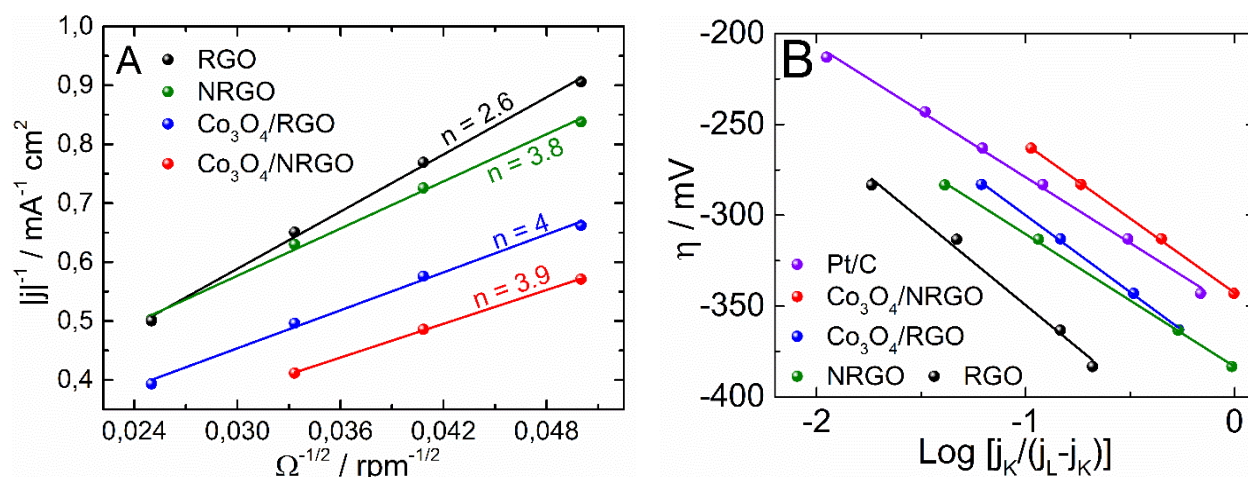
Figure III.10 A) Koutecky-Levich plots obtained from ORR polarization curves recorded using RGO, NRGO, Co 3 O 4 /RGO and Co 3 O 4 /NRGO materials as catalysts; B) Plot of the electrode overpotential as a function of \log [j_k/(j_L-j_k)] for the oxygen reduction on the different catalysts.
