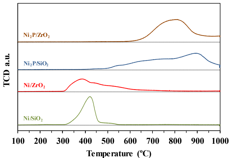
Figure 6-3 : H 2 -TPR profiles of nickel and nickel phosphide supported catalysts. Reduction conditions: 20 ml min -1 10% of H 2 in Ar with heating rate of 5°C min -1 .
