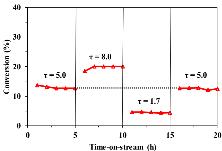
Figure 5-5 : Conversion of m-cresol under 4 MPa and 340 °C over Ni 2 P/SiO 2 as function of time-on-stream ( \tau in \text{g h mol}^{-1} ).
