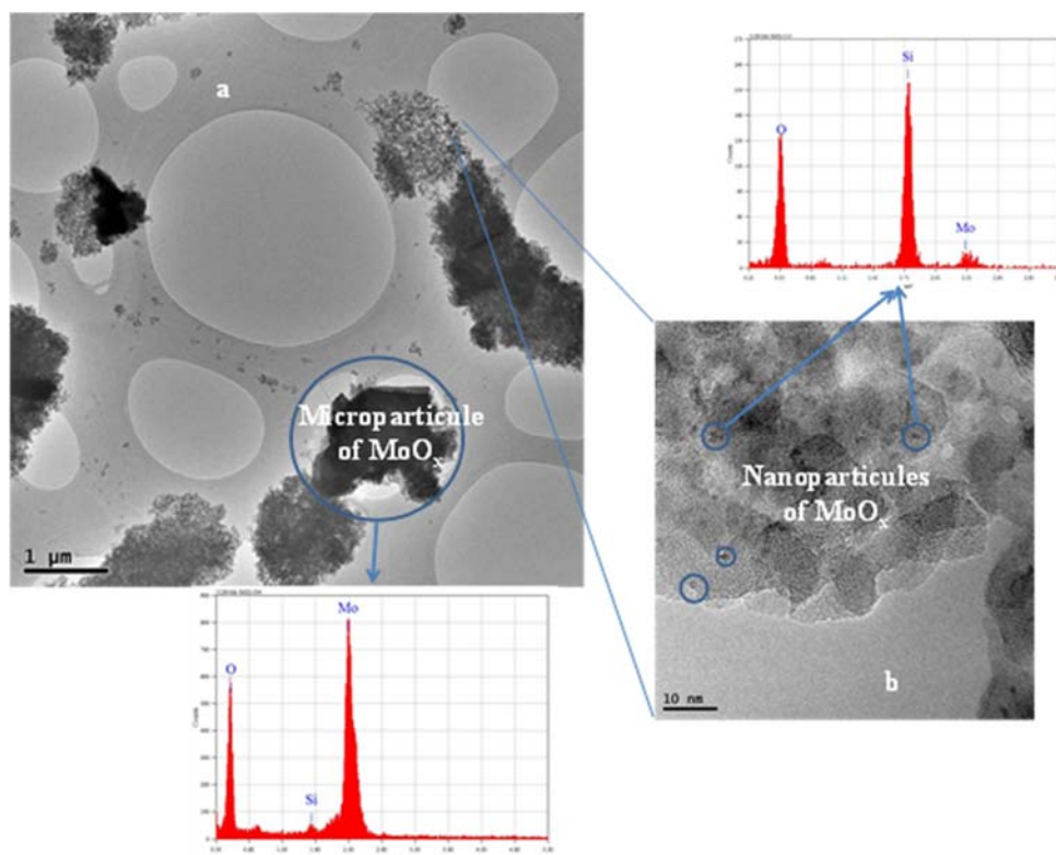
Figure 4-4 : TEM images and EDX analysis of \text{MoO}_x/\text{SiO}_2 at low (a) and high (b) magnification.
