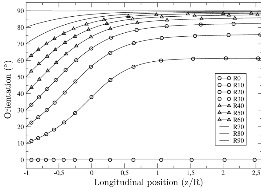
Figure 4.22: Instantaneous orientation versus position along the axis of the blood analyzer, for different initial orientations. The cases are labeled as RX , with X the value for \theta_0 .
