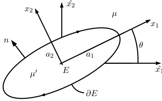
Figure 3.1: Schematic of an ellipsoidal membrane filled with fluid of viscosity \mu' suspended in a fluid of viscosity \mu , with the definition of the coordinate frames used in the analytical developments.
