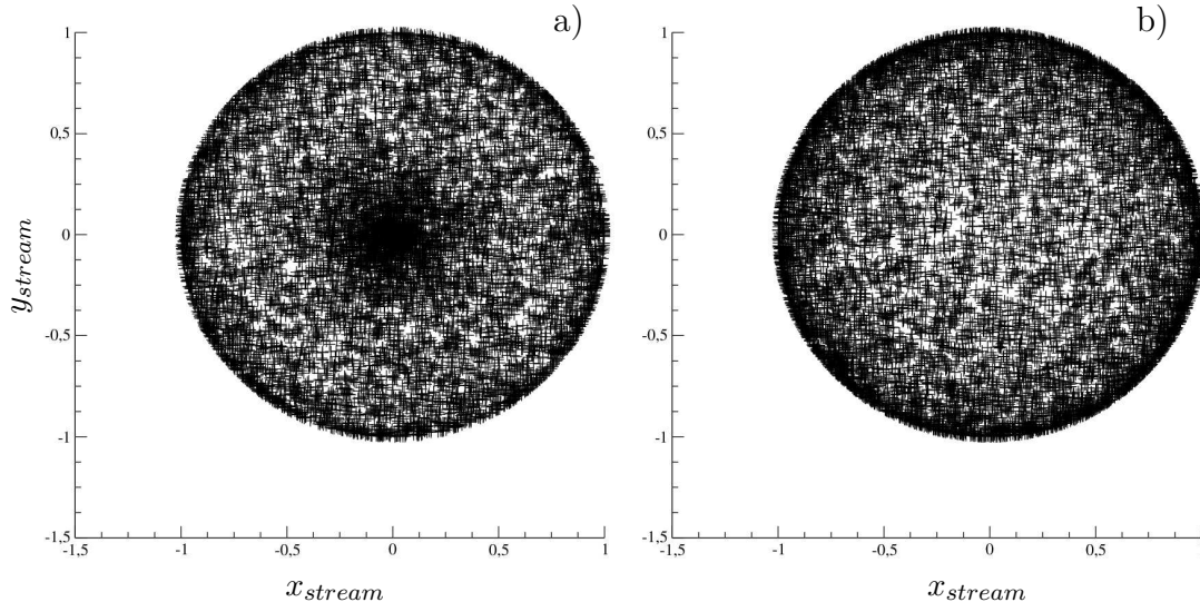
Figure 5.24: z_{RBC} vectors tips on the surface of the half-sphere, top-view for a ) A random selection of \theta' and \varphi' , b ) A random selection following Eq. (5.39) for \theta' and uniformly random for \varphi' .
