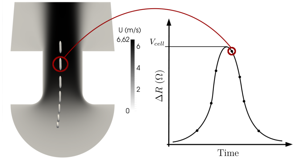
Figure 5.16: Resistive pulse schematic representation ( right ) and successive positions of a red blood cells in flow. ( left )
