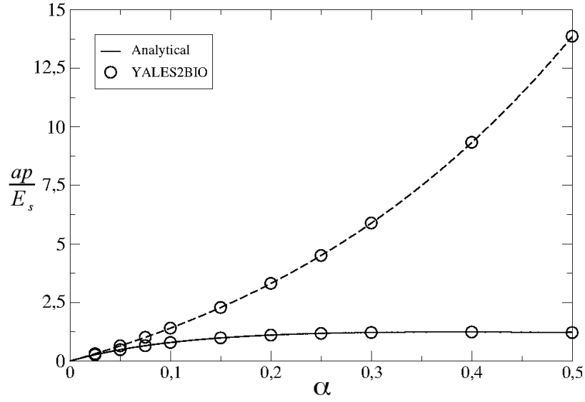
Figure 2.6: Non-dimensional pressure difference across the membrane for different values of the inflation factor \alpha in the cases of the Skalak law ( dashed ) and the Neo-Hookean law ( solid ).
