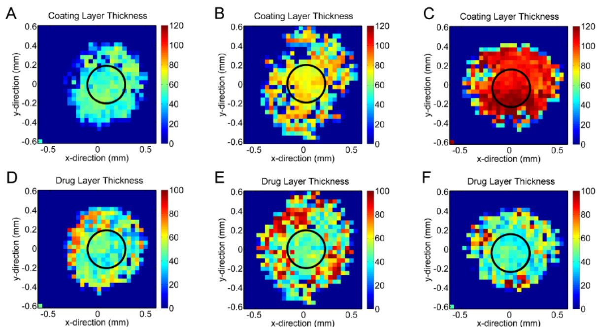
Figure39: Coating (top) and drug layer (bottom) thickness, 2D maps of a pellet from batch I (A and D), Batch II (B and E) and batch III (C and F). The black circles indicate the areas used for coating and drug layer thickness calculation. Dark blue pixels shown in the CT 2D maps correlate with measurement failure and do not comprise a signal related to the coating/drug layer interface thus, they were excluded from the CT and DLT calculation. The colour scale bars are in \mu\text{m} .
