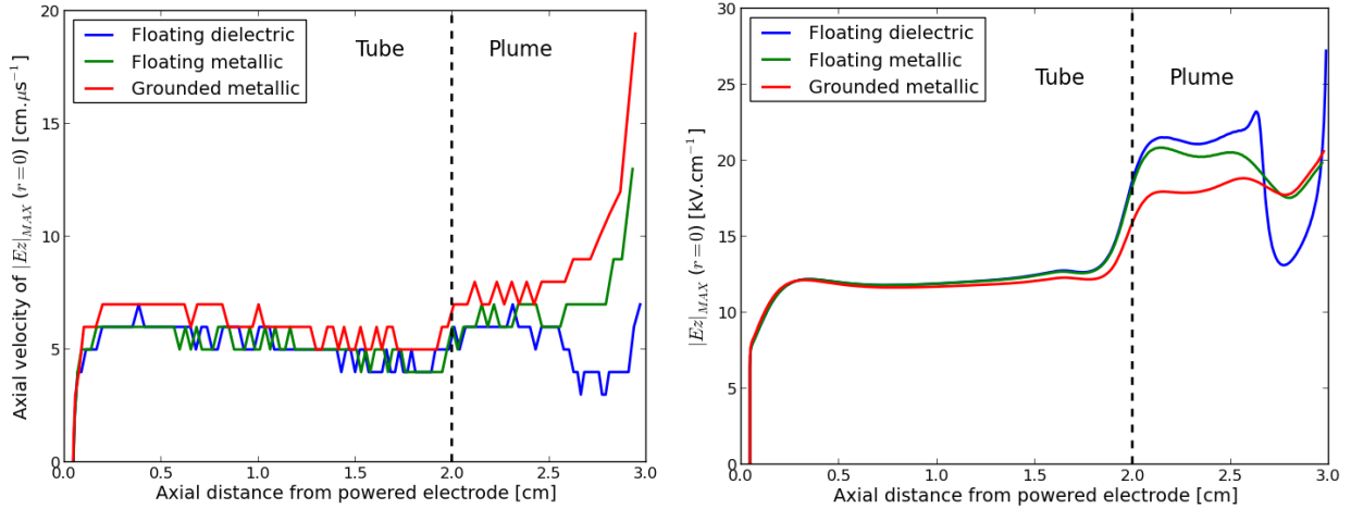
Figure V.10: Axial velocity of propagation of |E_z|_{MAX} (on the left) and |E_z|_{MAX} (on the right) at r = 0 between the powered electrode and the target, with 5 ns temporal resolution, for floating dielectric, floating metallic and grounded metallic targets, with V_P = +4 kV.
