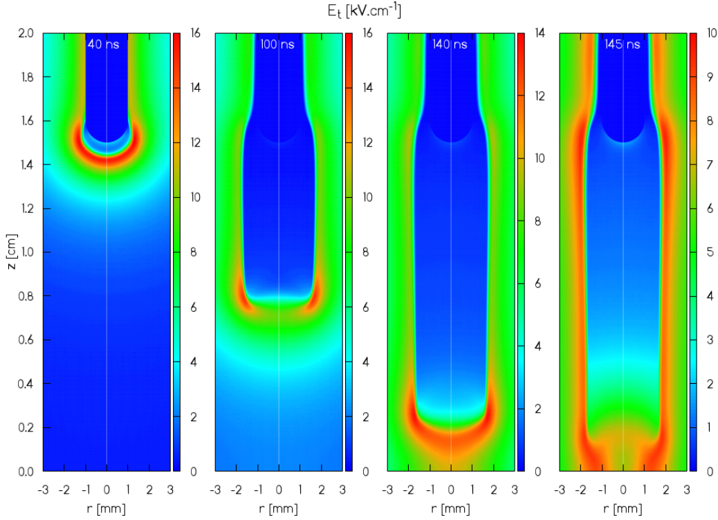
Figure III.8: Cross sectional views of the magnitude of the electric field at t = 40, 100, 140 and 145 ns, for a 2 cm long tube with r_{in} = 2 mm, r_{out} = 3 mm and \epsilon_r = 1 , closed by a grounded target for V_P = +4 kV.
