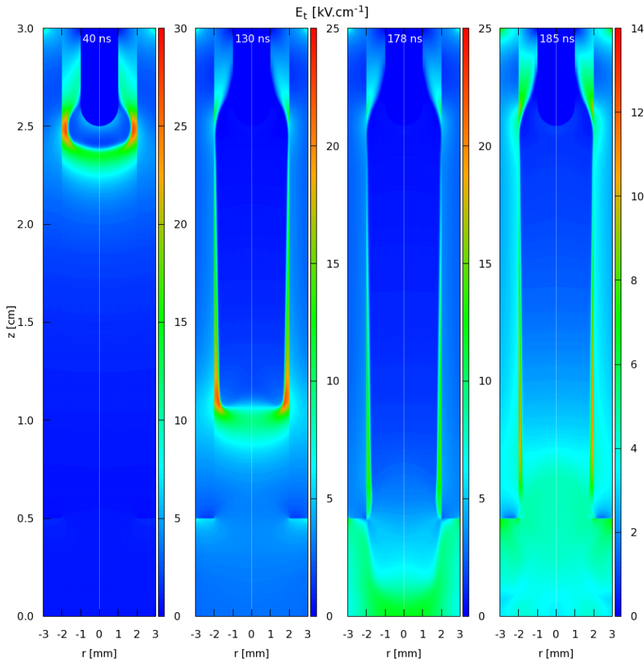
Figure IV.20: Cross sectional views of the magnitude of the electric field at t = 40, 130, 178 and 185 ns, for a 2.5 cm long tube and a 0.5 cm tube-target distance, for V_P = +6 kV.
