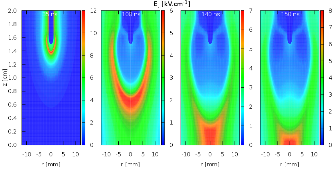
Figure III.3: Cross sectional views of the magnitude of the electric field at t = 35, 100, 140 and 150 ns, for a 2 cm long domain without tube with a grounded target for V_P = -4 kV.
