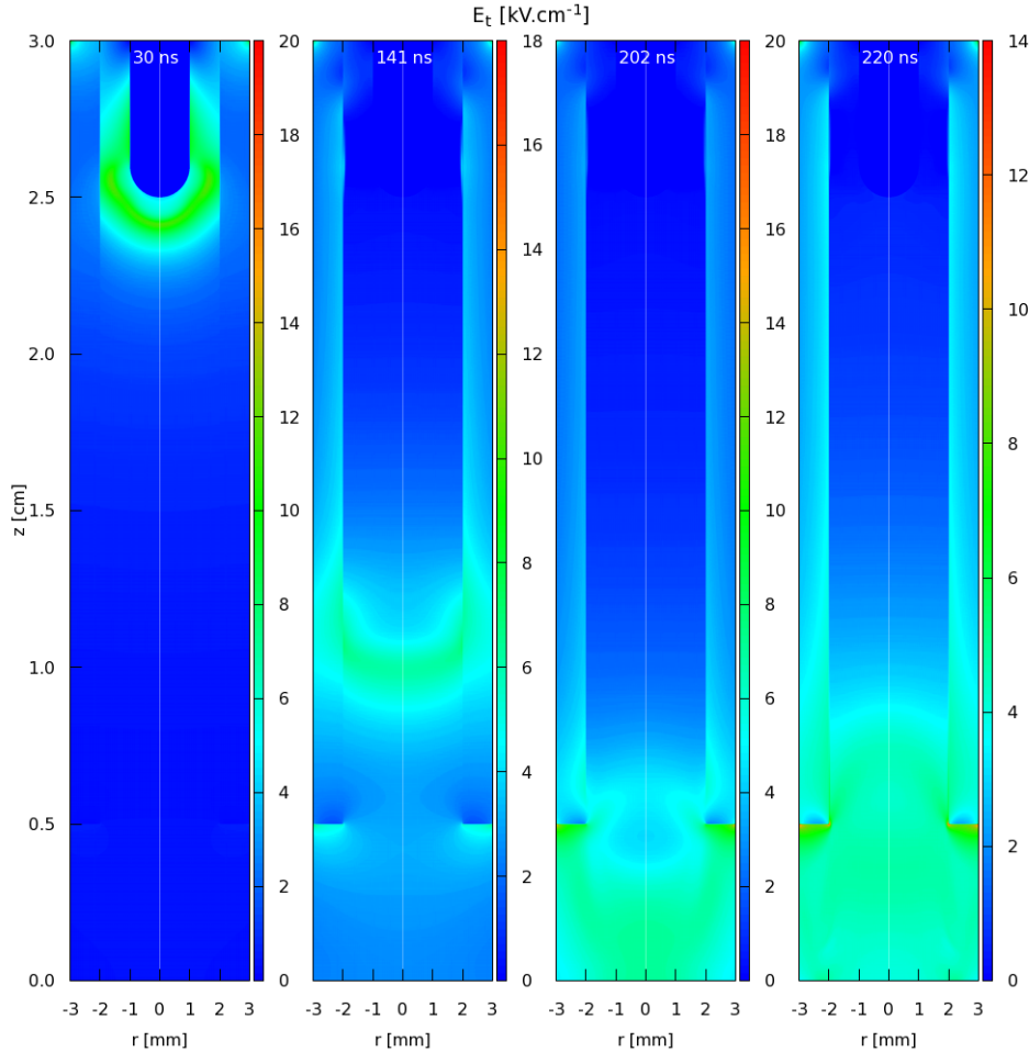
Figure IV.21: Cross sectional views of the magnitude of the electric field at t = 30, 141, 202 and 220 ns, for a 2.5 cm long tube and a 0.5 cm tube-target distance, for V_P = -6 kV.
