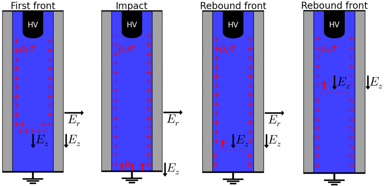
Figure IV.14: Side view schematics of the temporal sequence representing the dynamics of the rebound discharge and of the electric field evolution described in this chapter, aimed at describing the case with positive polarity of applied voltage. Charges and charge movement are represented in red. ‘n’ stands for charge neutrality. Axial and radial components of electric field are represented in black.
