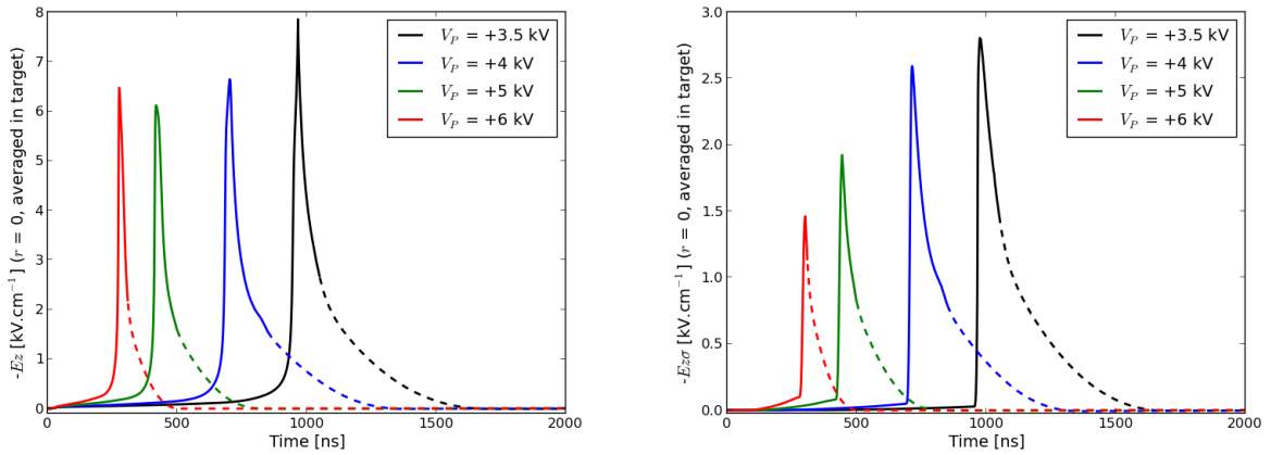
Figure G.4: Temporal evolutions of E_z at r = 0 averaged through the thickness of the dielectric target ( \epsilon_r = 4 ) of 0.5 mm, with different applied voltages, with 1 ns resolution. In the figure on the left, the total E_z(t) . In the figure on the right, the surface charge contribution E_{z\sigma}(t) . Dashed lines are used when the applied voltage becomes zero.
