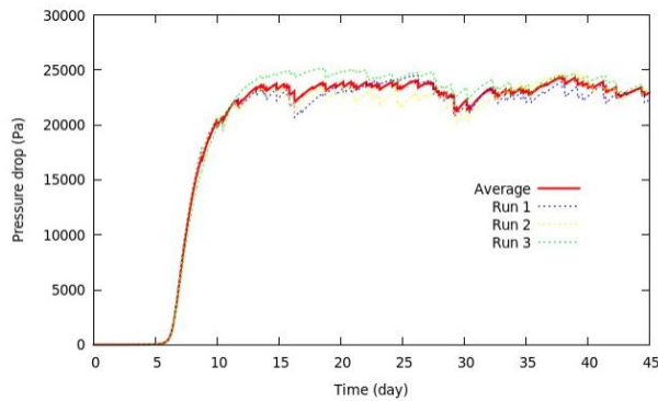
Figure 6.14c: k_{r \max}=500 , k_{r \min}= 80 , \mu_{\max}=5.10^{-5} \text{ s}^{-1} , \Delta t=18000\text{s} , C_s=0.2 \text{ kg/m}^3
