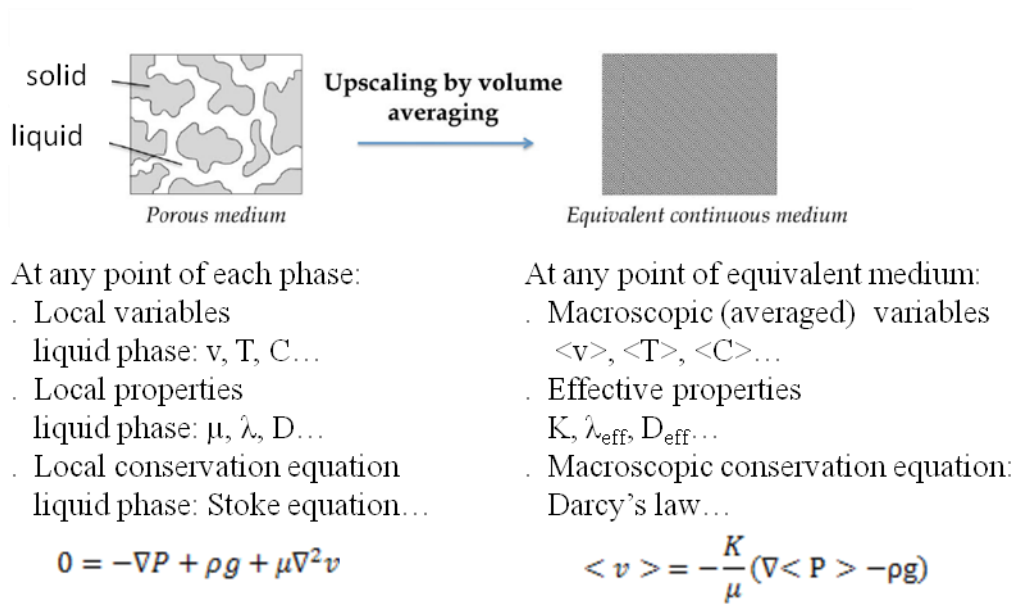
Figure 2.18: Example of upscaling from volume averaging (taken from Habibi, 2014)
