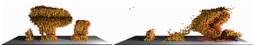
Figure 2.15: Biofilm deformed and detached under the fluid flow (Alpkvist and Klapper, 2007a)
