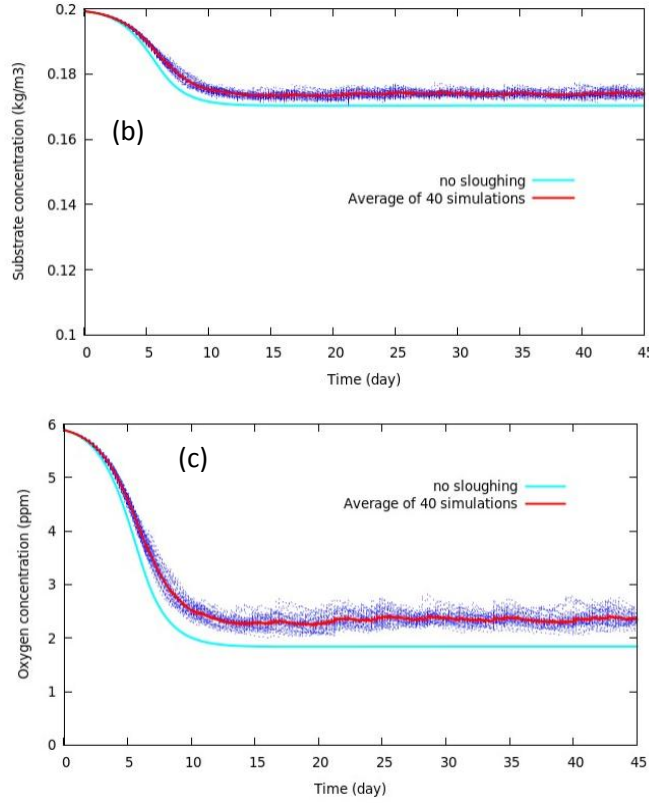
Figure 6. 15. The mean value of stochastic process (a) pressure loss, (b) substrate concentration and (c) oxygen concentration . The sloughing parameters in the simulation were , \Delta t = 18000s , k_t=80 , \mu_{max}= 5 \times 10^{-5} s^{-1}
