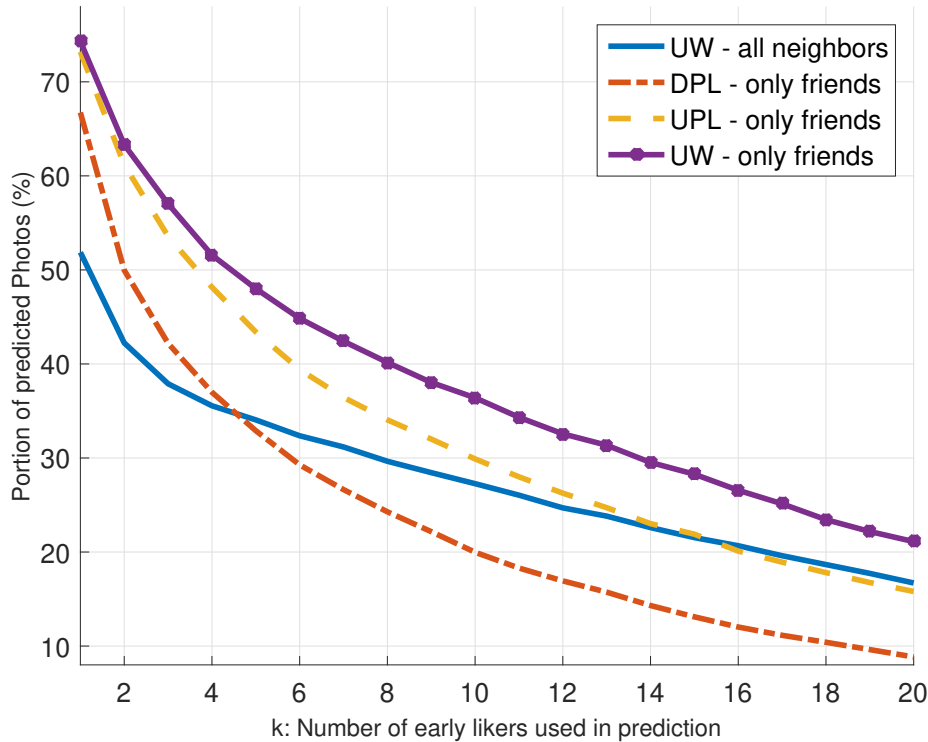
Figure 4.2 – The portion of photos with at least one correct prediction in their future likers for different k numbers of early likers. Choosing likers from friendships improves the prediction results.
