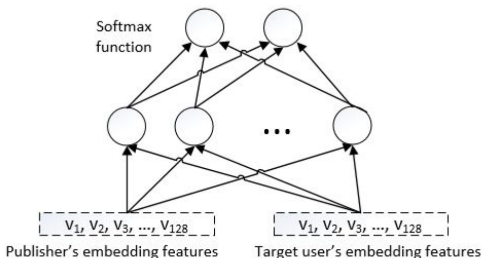
Figure 5.2 – One-hidden layer neural network with softmax function in the final layer to predict the target user’s reaction probability.
