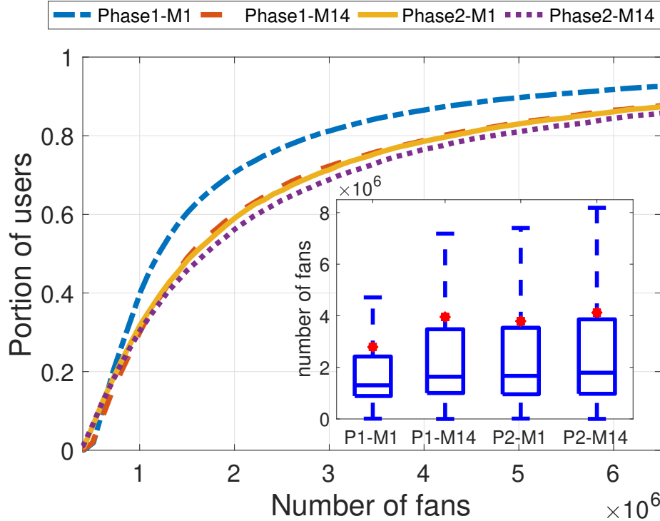
Figure 3.8 – users’ CDF with the box-plots of #fans ( N_f ) distributions including two phases of M1 and M14. Red dots represent the mean values of N_f in particular month.
