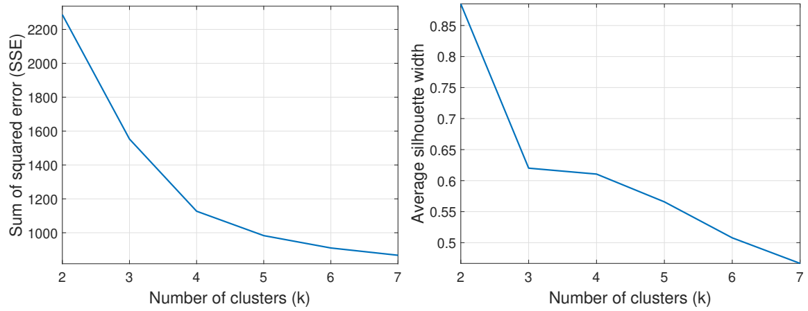
(a) SSE for different cluster numbers
