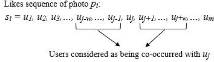
Figure 4.1 – Co-occurrences are computed for each user in the like sequences with her surrounded users, placed in a window of size w from two directions.
