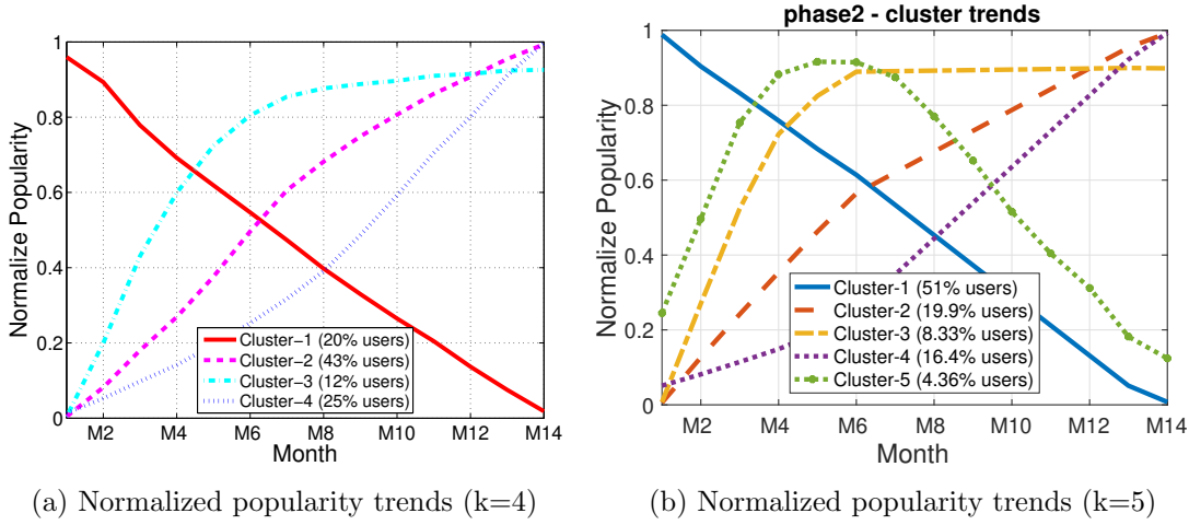
Figure 3.12 – Popularity trends in two phases
