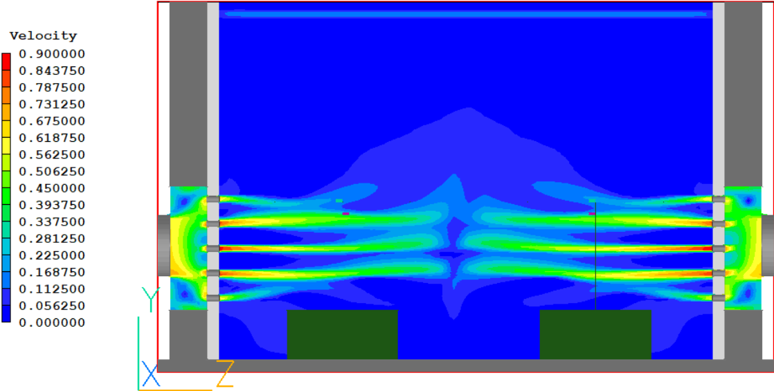
Figure 4.17: Velocity profile in the enclosure at the higher air flow rate - Front View.
