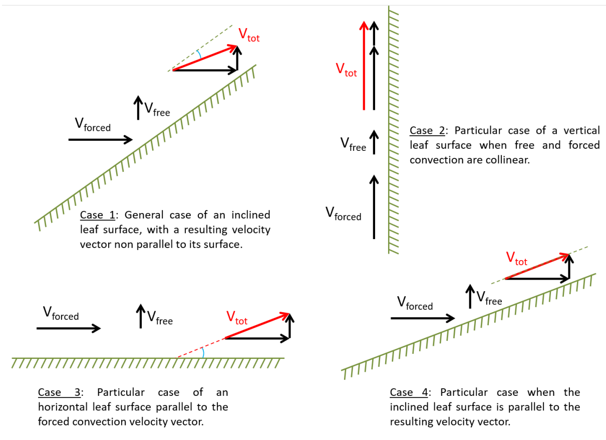
Figure 2.10: Schematic of the leaf surface with the free and forced convection vectors and the resulting vector V_{tot} for four different cases.
