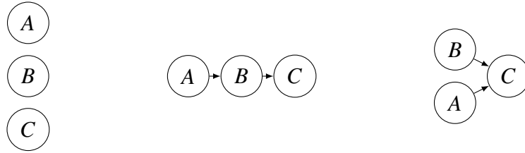
Figure 2.1: Some examples of episodes. An arc from left to right means that the source node precedes the end node in the sequence. The left episode is a parallel episode: the items can occur in any order. The middle episode is a serial episode, where the order between all items is total. The right episode is a general episode. The mapping g between each node and event is represented by the item name in each node.
