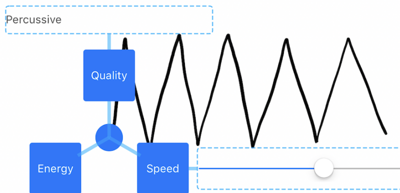
Figure 59: Knotation : Knot attached to a zigzag trajectory. Tapping the knot reveals three attributes: quality , energy and speed . Here, the knot defines a “ percussive ” quality, with a slider to indicate speed.
