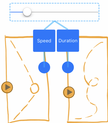
Figure 71: The same controller (slider) could be linked to several attributes (speed and duration) in different choreographic objects.
