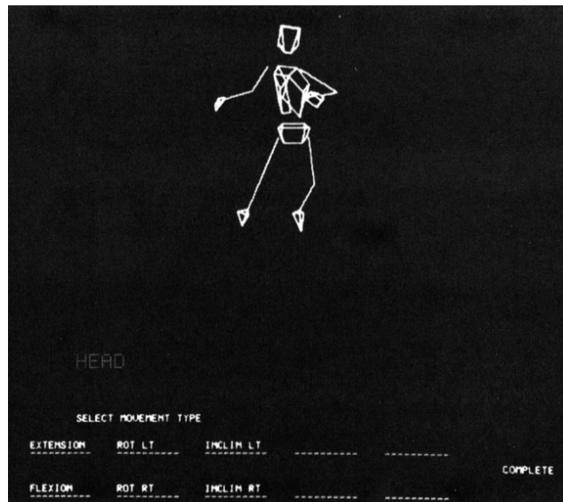
Figure 50: Choosing a body part in the CHOREO system. Source: Savage and Officer (1977).
