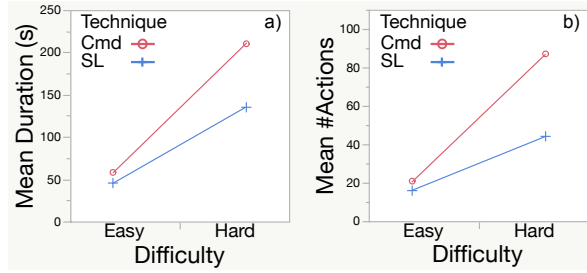
Figure 24: Experiment: Interaction effects between TECHNIQUE and DIFFICULTY for (a) duration and (b) number of actions.
