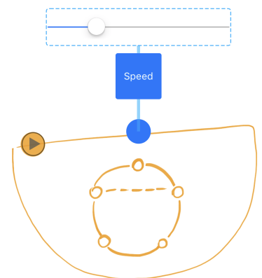
Figure 60: Knotation : A floorplan with a speed knot controlled by a slider.
