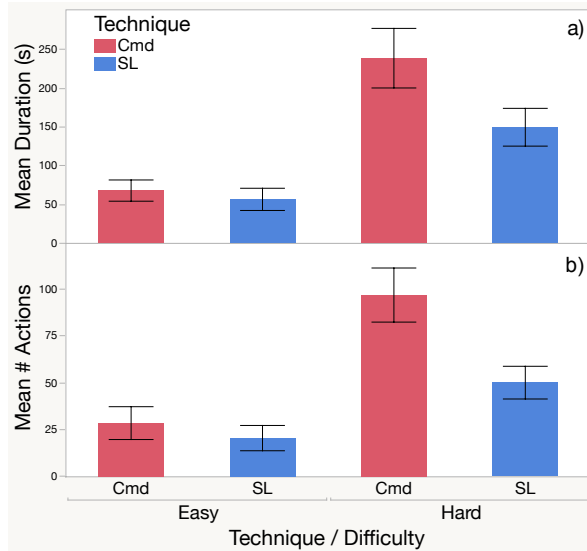
Figure 25: Experiment: Mean duration (a) and Mean number of actions (b) by TECHNIQUE \times DIFFICULTY , with 95% confidence intervals.
