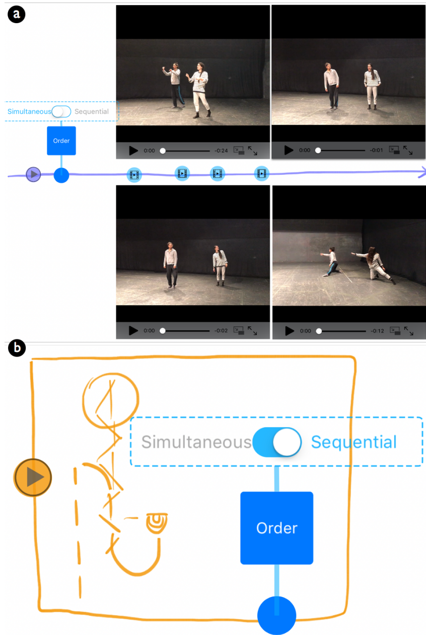
Figure 63: Knotation : Playing multiple videos at the same time with a simultaneous timeline (a). Animating trajectories one by one in a sequential floorplan (b).
