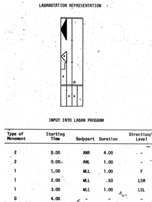
Figure 49: Input to Wolofsky's Laban program. Source: Wolofsky (1974).
