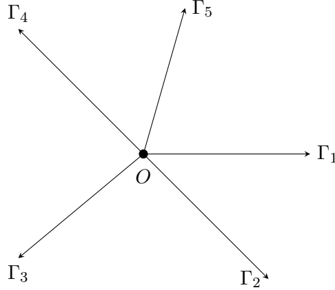
Figure 2.1: The junction \mathcal{G} with 5 edges on \mathbb{R}^2
