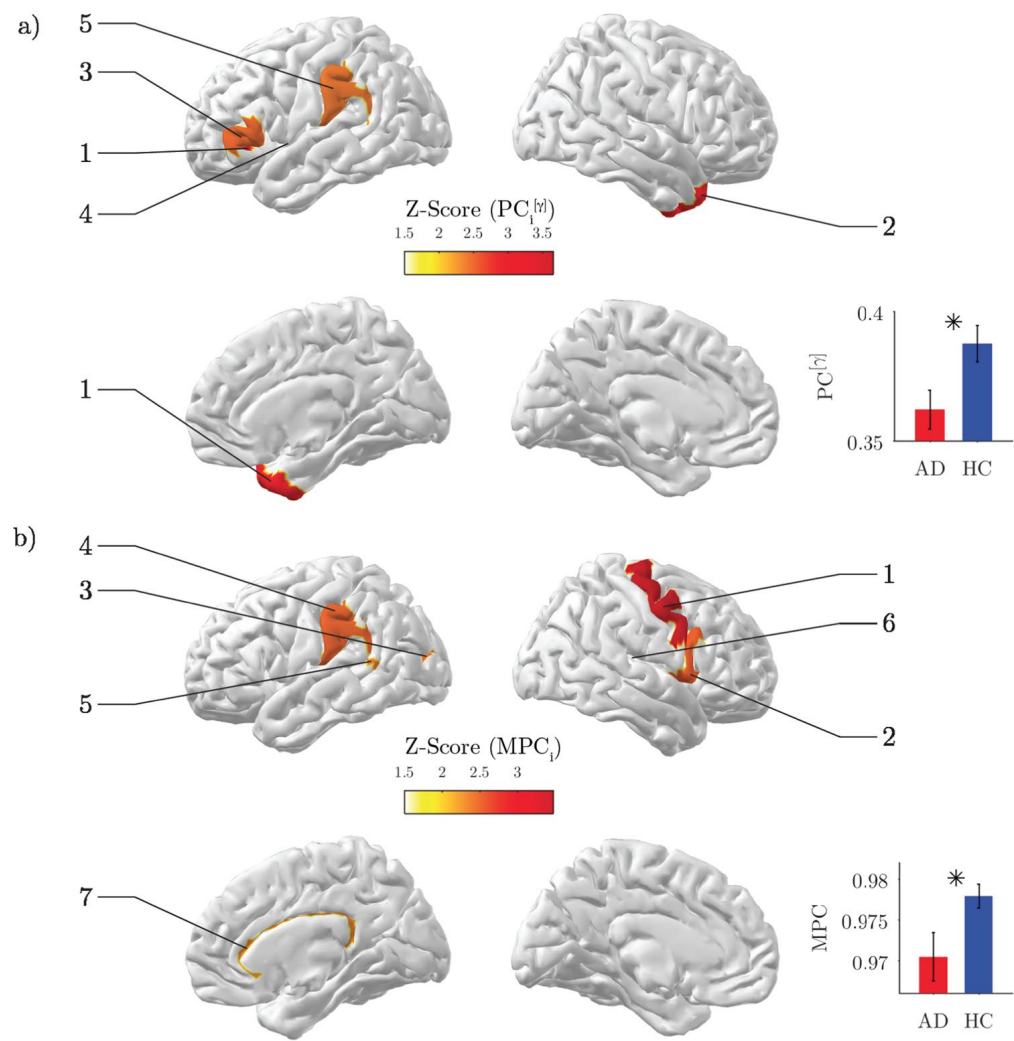
Figure 3. Network analysis of brain connectivity. (a) Inter-modular centrality. Statistical brain maps of group differences for local participation coefficients PC_i in the gamma band. Only significant differences are illustrated ( p < 0.05 , FDR corrected). The labels same ranks are used as labels. The inset shows the results for the global PC ; vertical bars stand for group-averaged values while error bars denote standard error means. In both cases, Z-scores are computed using a non-parametric permutation t-test. (b) Inter-frequency centrality. Statistical brain maps of group differences for local multi-participation coefficients MPC_i . The inset shows the results for the global MPC ; same conventions as in (a) .
