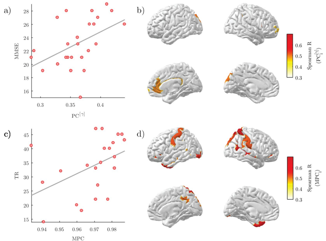
Figure 6. Correlation between brain network properties and cognitive/memory scores. (a) Scatter plot of the global participation coefficient in the \gamma band ( PC^{[\gamma]} ) and the mini-mental state examination (MMSE) score of AD subjects (Spearman's correlation R = 0.4909 , p = 0.0127 ). (b) Correlation brain maps of the local participation coefficient in the \gamma band ( PC_i^{[\gamma]} ) and the mini-mental state examination (MMSE) score of AD subjects. Only significant R values are illustrated ( p < 0.05 , FDR corrected). (c) Scatter plot of the global multi-participation coefficient (MPC) and the total recall (TR) score of AD subjects (Spearman's correlation R = 0.5547 , p = 0.0074 ). (d) Correlation brain maps of the local multi-participation coefficient ( MPC_i ) and the total recall (TR) score of AD subjects. Only significant R values are illustrated ( p < 0.05 , FDR corrected).
