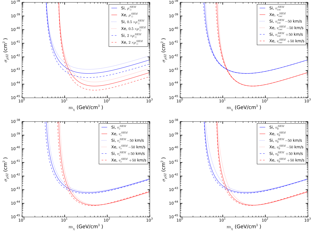
Figure 2.3: The figure shows the impact on DMDD exclusion curves of variations in the astrophysical parameters usually fixed by the SHM, \rho_\odot , v_{\text{esc}} , v_c and v_0 (see section 1.8). The limits are computed for illustration using Poisson statistics assuming 0 events detected (thus applying N_{th} \leq 2.30 to obtain a 90% C.L. limit) in a recoil energy range comprised between E_T = 5 keV and E_{\text{max}} = 100 keV, with a total exposure of 500 kg \times day. We consider two different target nuclei, silicon (lighter) and xenon (heavier). Top left panel: the local dark matter density \rho_\odot . Top right panel: the local Galactic escape speed v_{\text{esc}} . Bottom left panel: the local circular speed v_c . Bottom right panel: the most probable speed v_0 (which gives also the velocity dispersion) of the cut Maxwell-Boltzmann velocity distribution assumed.
