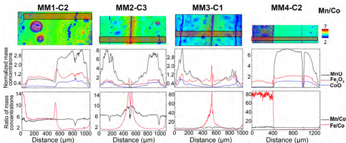
Figure 2.C.3.1 Focus on the evolution of Mn, Co and Fe concentration over the four thin sections. Top: Mn/Co XRF map (same conditions as Figure 2.C.2.3). The red rectangle represents the line chosen to calculate the following profiles (sum over an height of 100\mu\text{m} : 50 pixels). Middle: 1D profiles of Co, Fe and Mn. Bottom: 1D profiles of Mn/Co and Fe/Co.
