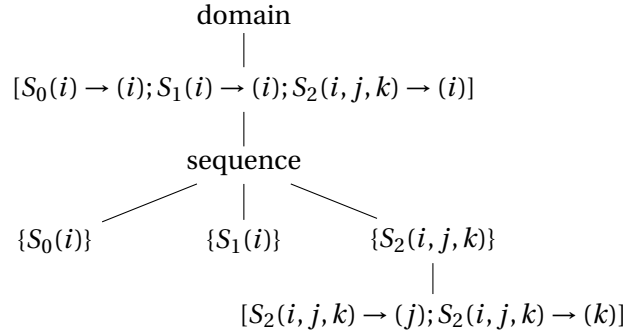
Figure 4.4 – A correct schedule tree of the example
