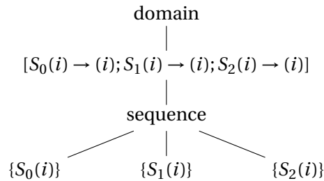
Figure 3.3 – Original schedule tree of the example
