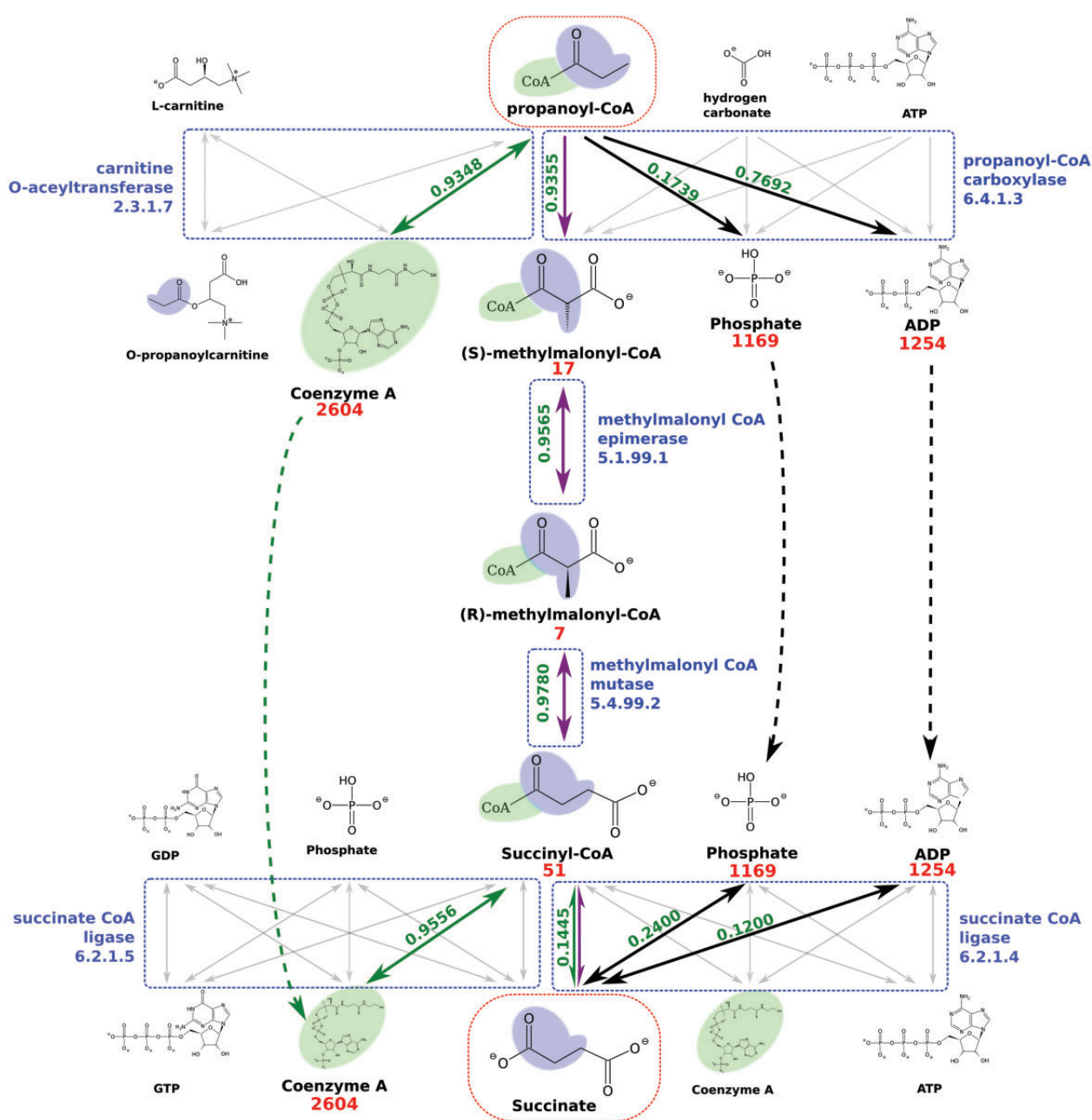
Figure 6. Path searches applied to the propanoyl-CoA to succinate degradation pathway using different weighting policies. Edges involved in at least one path are in bold. MACCS fingerprint similarities are displayed on edges, compound degrees are displayed below nodes. The part of the molecules highlighted in the same colour represents atom mapping. The pathway as described in HumanCyc, shown here in the middle, goes through (S)-methylmalonyl-CoA, (R)-methylmalonyl-CoA and succinyl-CoA. The same path was retrieved using Dijkstra shortest path algorithm on Recon2 human global network weighted by degree, degree square, degree cube and chemical similarity using PubChem, Klekota-Roth, EState and CDK's extended fingerprints. The shortest paths computed on unweighted graph only use ADP or phosphate as intermediary compounds (paths on the right); the shortest path computed using MACCS and CDK's substructure fingerprint (path on the left) goes from propanoyl-CoA to succinate through coenzyme A and succinyl-CoA.
