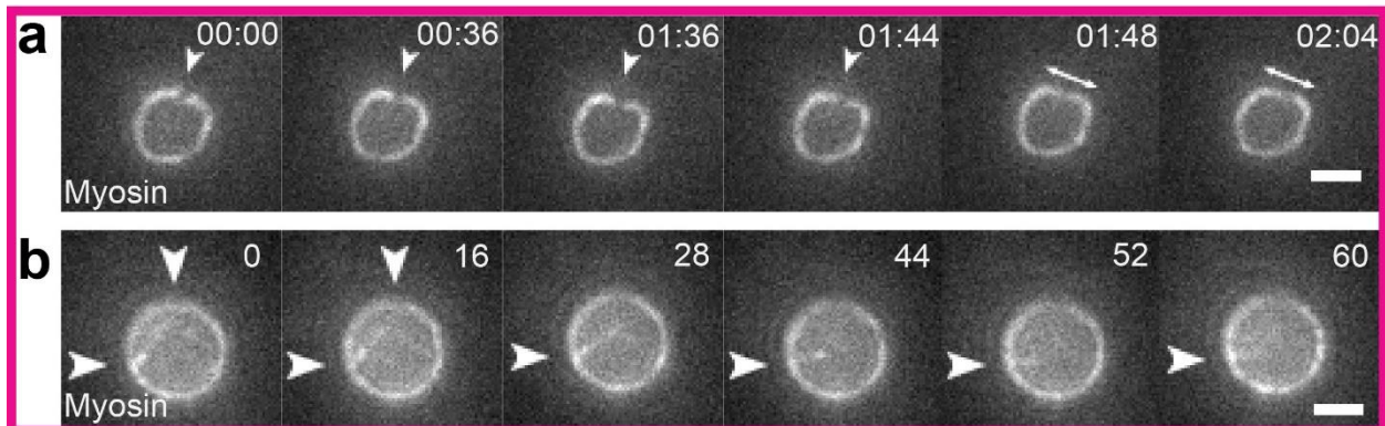
Figure 4.21. Defects in the ring, visualized by myosin. (a) Spontaneous breakage in the ring, which eventually heals to complete the ring (109). (b) Long actin filaments (cables) separating from the ring are integrated back into the ring. All these experiments were done at 36 °C.
