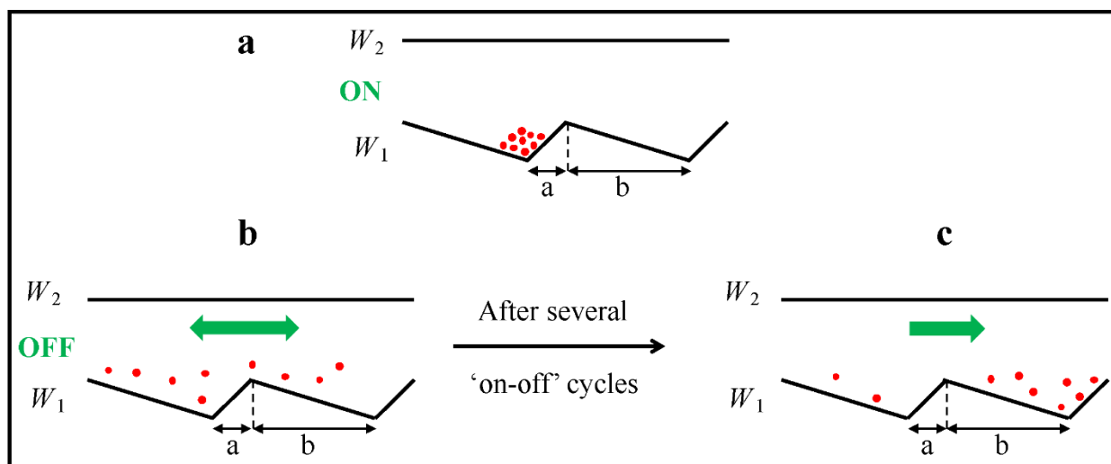
Figure 6.3. Representation of particle-potential system described in Prost et al. (220). The particles can be in two potential states W_1 and W_2 . ‘a’ and ‘b’ represent the shorter and longer slopes, respectively on either side of the maxima in the potential. The red dots denote particles under study. (a) When W_1 is switched ‘on’, particles are trapped in the minima due to the asymmetric nature ( b > a ). (a) But when W_1 is switched ‘off’, the particles experience a flat profile ( W_2 ), and are free to diffuse (indicated by green arrows). When subjected to several ‘on-off’
