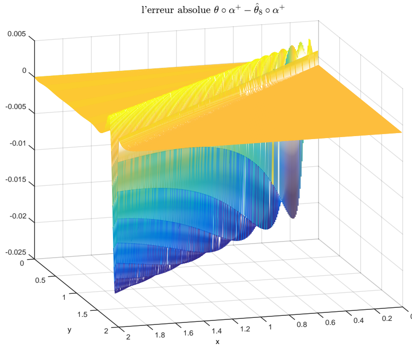
FIGURE 3.5 – Erreur absolue \theta \circ \alpha^+ - \hat{\theta}_8 \circ \alpha^+
