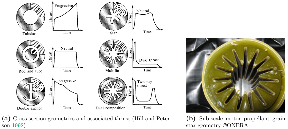
Figure 1.4: Examples of propellant grain cross sections
